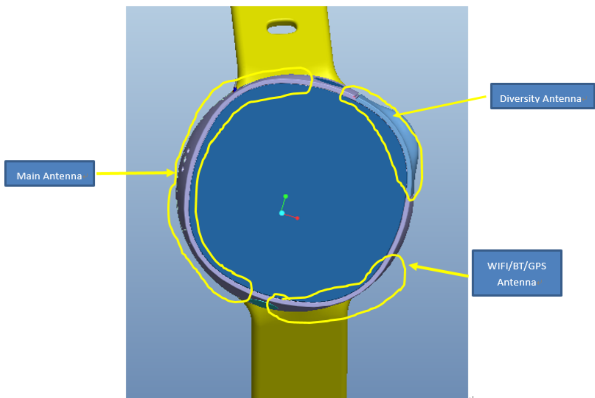
Antenna specification.
