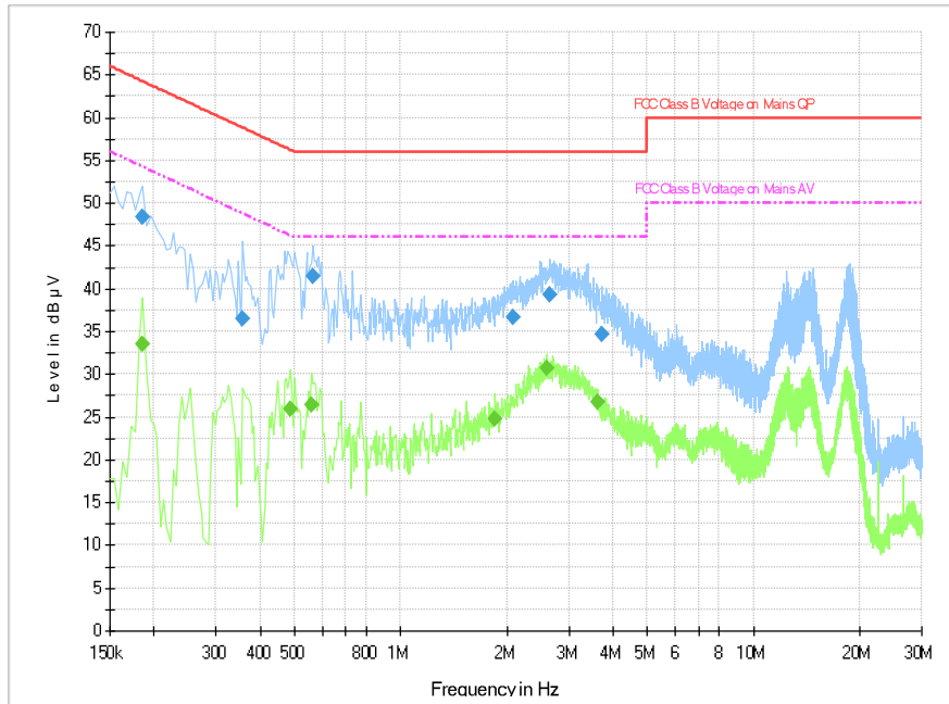
Fig.B.9.1 AC Powerline Conducted Emission-traffic
