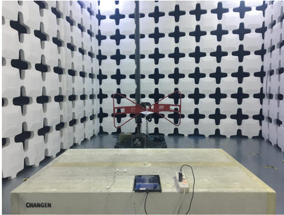
9. Radiated Emissions (Part 15B Charging Mode with FM Mode,30MHz-1GHz)
