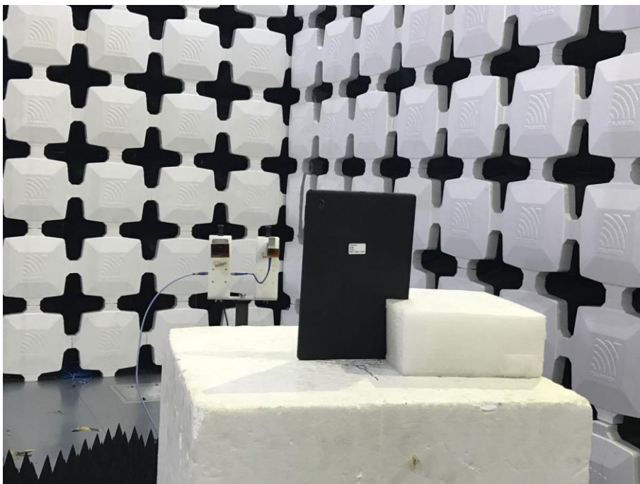
20. Radiated Emissions (Part 22/24/27, 26.5GHz -40GHz)
