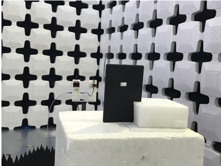
17. Radiated Emissions (Part 15C&Part 15E, 26.5GHz -40GHz)
