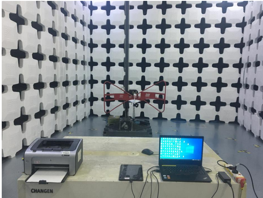
1. Radiated Emissions (Part 15B Data Transfer Mode,30MHz-1GHz)
