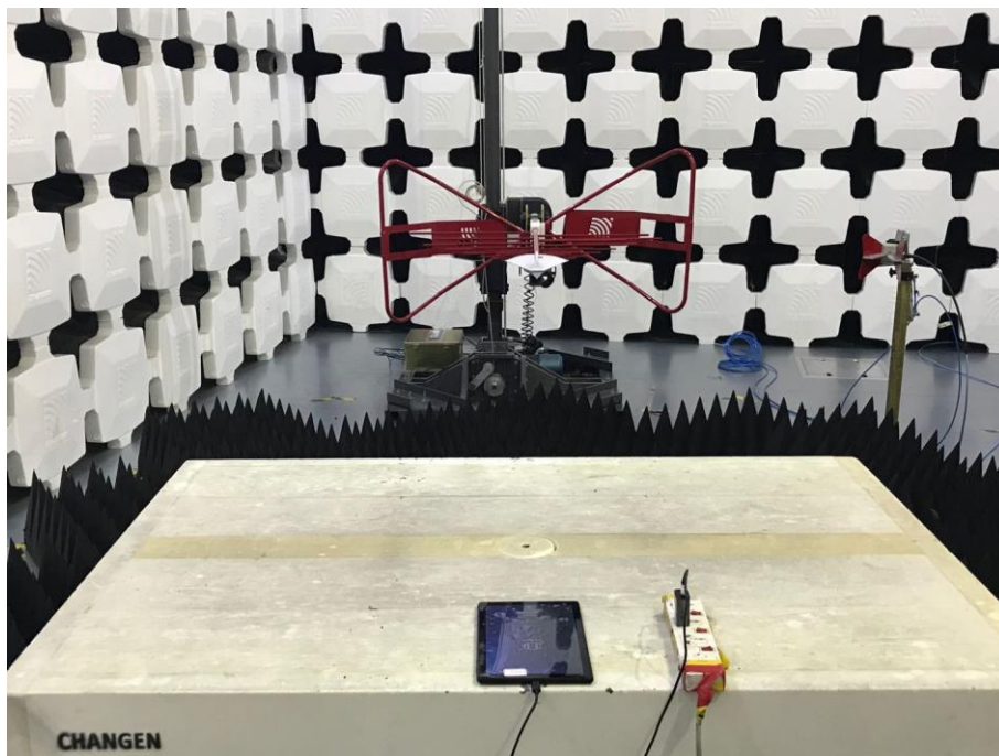
6. Radiated Emissions (Part 15B Charging Mode with Camera Mode/Video Player Mode/GSM receiver/WCDMA receiver/LTE receiver,1GHz-18GHz)
