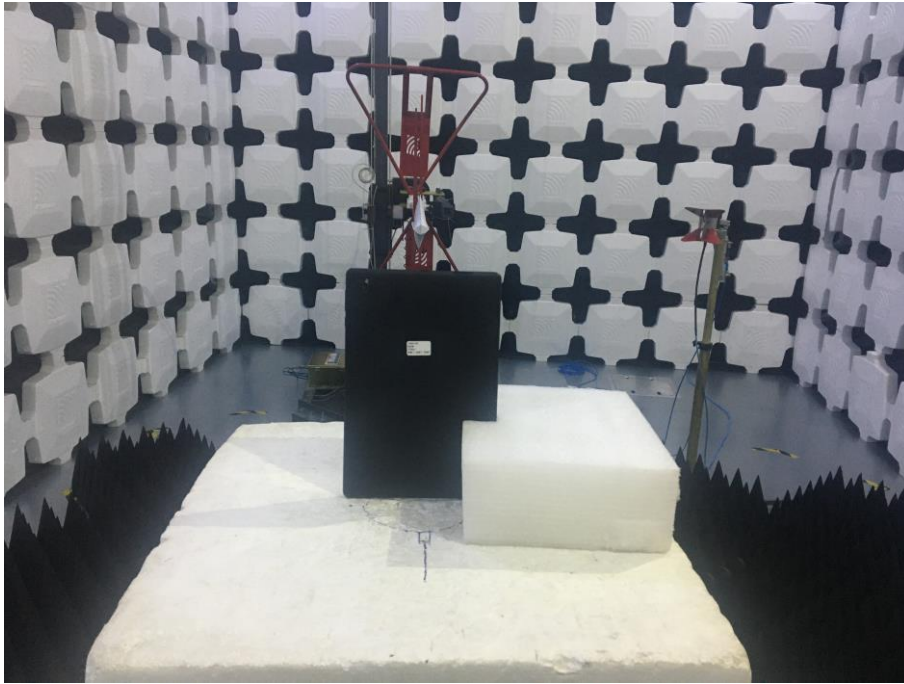
15. Radiated Emissions (Part 15C&Part 15E, 1GHz -18GHz)
