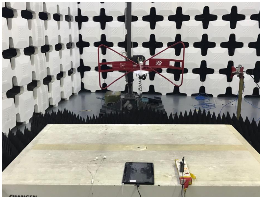
10. Radiated Emissions (Part 15B Charging Mode with FM Mode,1GHz-18GHz)
