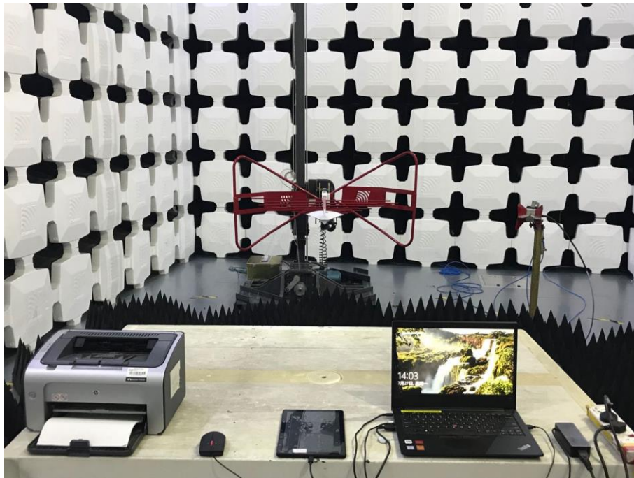
2. Radiated Emissions (Part 15B Data Transfer Mode,1GHz-18GHz)
