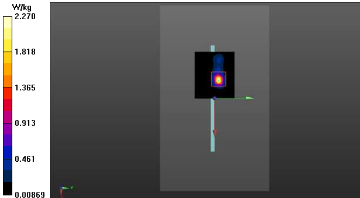
Fig.14 WLAN 5G Body
