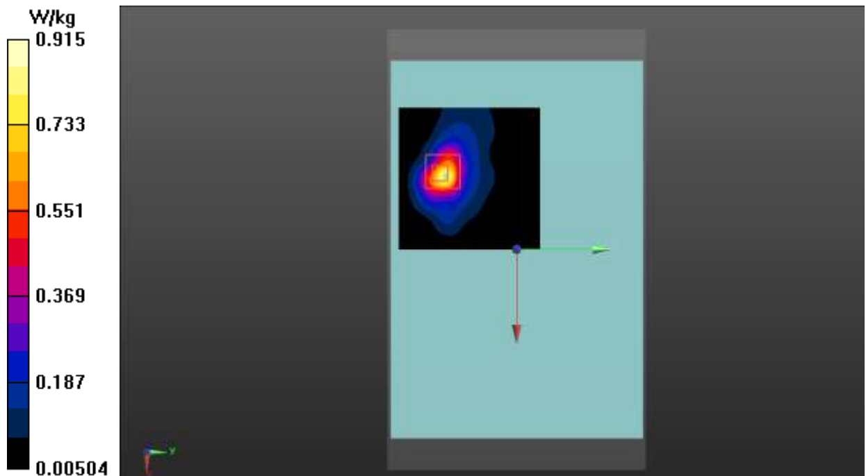
Fig.13 WLAN 2.4G Body
