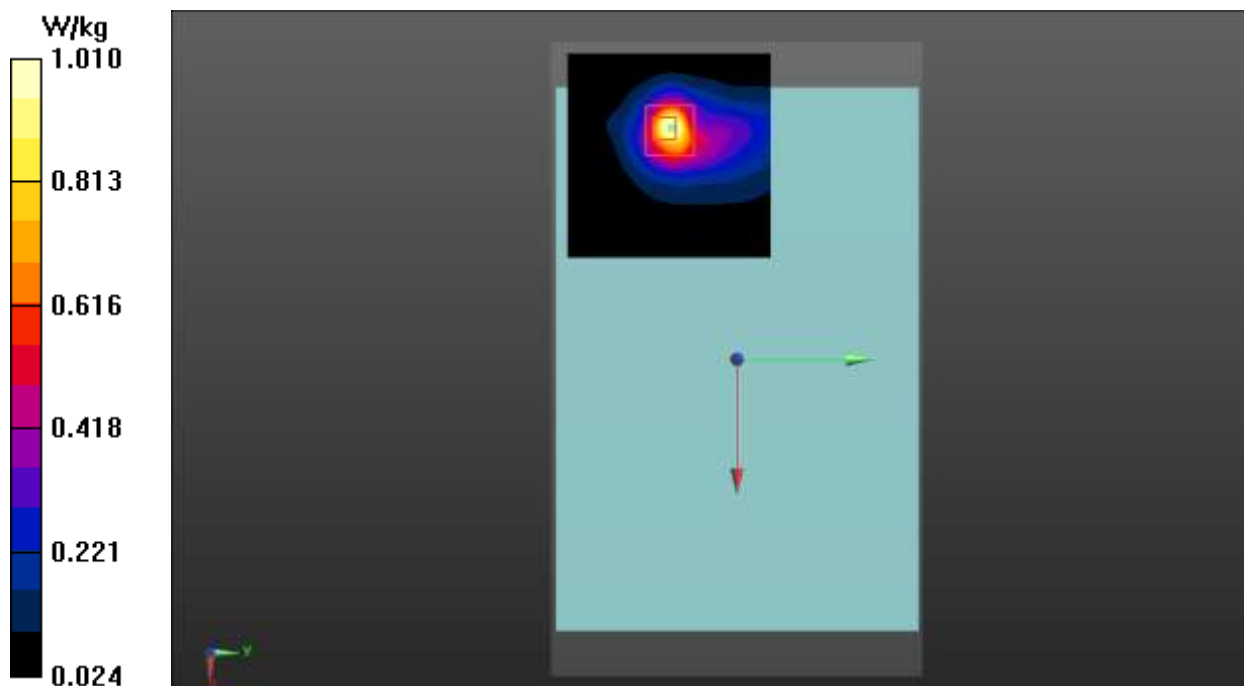
Fig.11 LTE Band 66 Body
