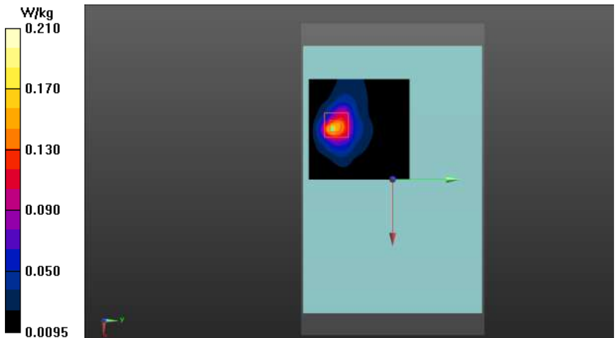
Fig.12 Bluetooth 2.4G Body
