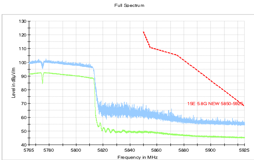
Fig. 28 Band Edges (802.11ac-HT80, 5775MHz)
