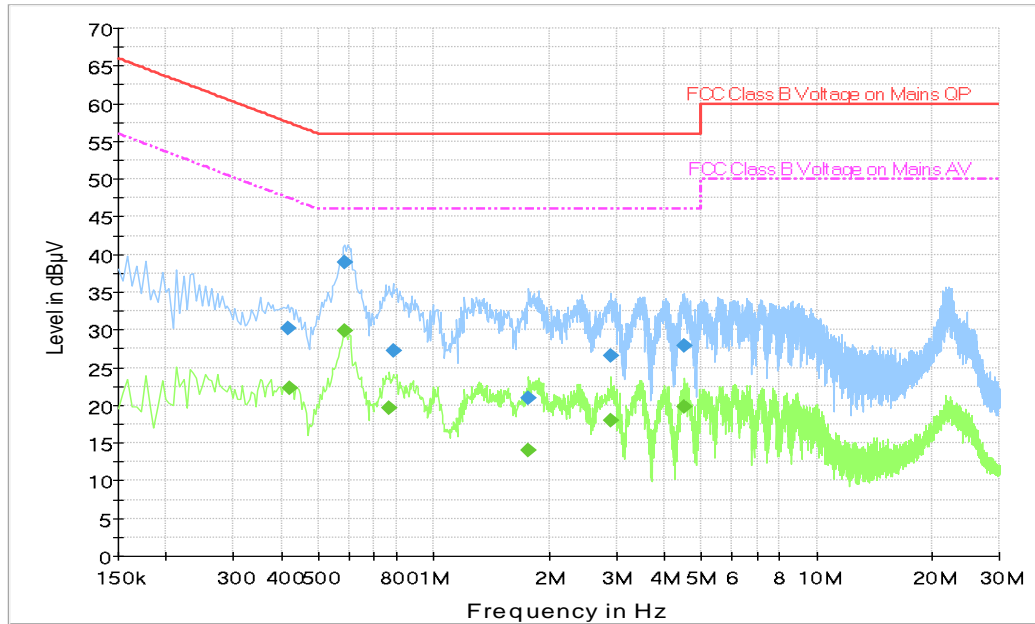
Fig. 30 AC Power line Conducted Emission-Idle
