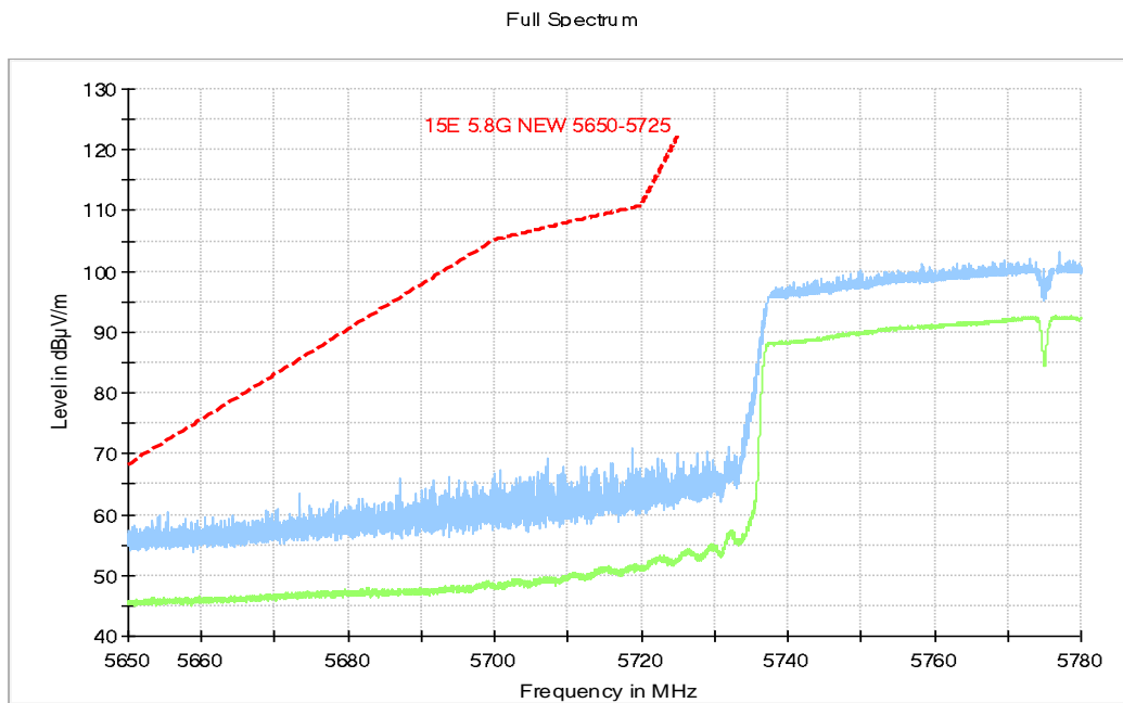
Fig. 27 Band Edges (802.11ac-HT80, 5775MHz)
