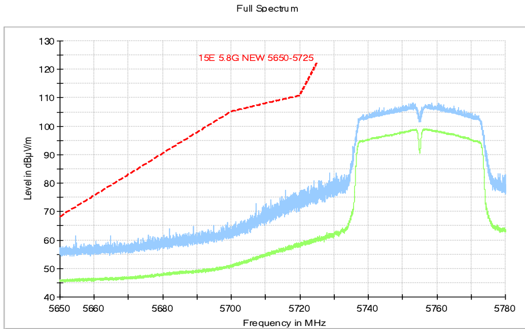
Fig. 20 Band Edges (802.11n-HT40, 5755MHz)
