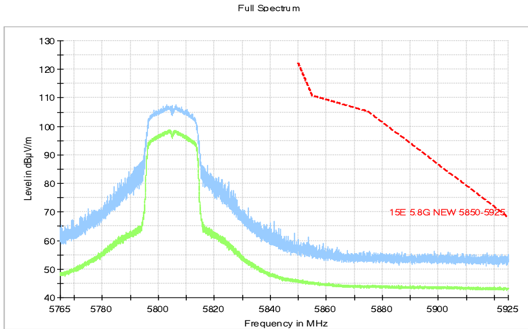
Fig. 19 Band Edges (802.11n-HT20, 5805MHz)
