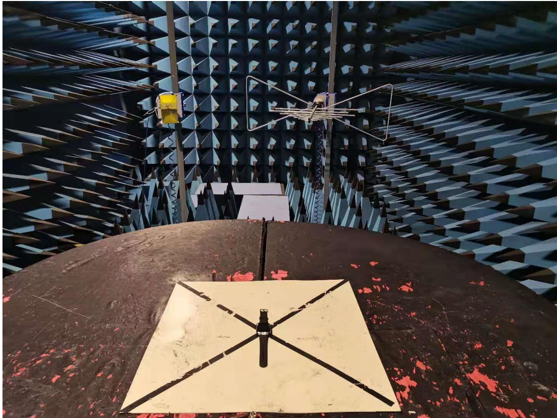
Radiated Emission 1-18GHz -Front
