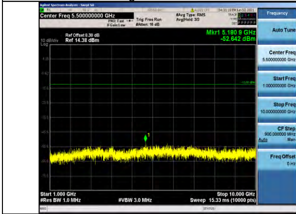
Band71-15MHz-16QAM-133197-1RB#0- Range2:1000~10000MHz
