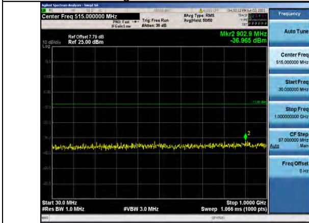
Band71-15MHz-16QAM-133297-1RB#0- Range1:30~1000MHz
