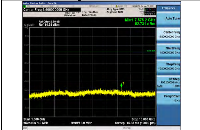
Band 13-5MHz-QPSK-23230-1RB#0-Range2:1000~10000MHz
