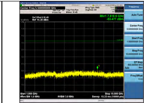
Band71-15MHz-16QAM-133297-1RB#0- Range2:1000~10000MHz
