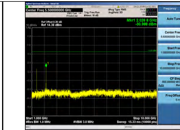
Band71-10MHz-16QAM-133297-1RB#0- Range2:1000~10000MHz
