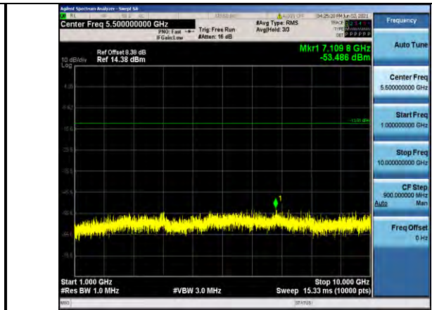
Band71-20MHz-16QAM-133322-1RB#0- Range2:1000~10000MHz
