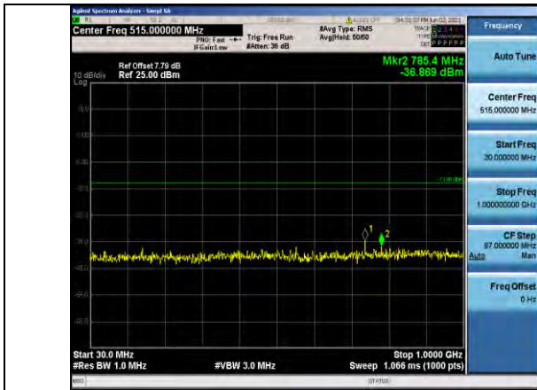
Band71-15MHz-16QAM-133197-1RB#0- Range1:30~1000MHz
