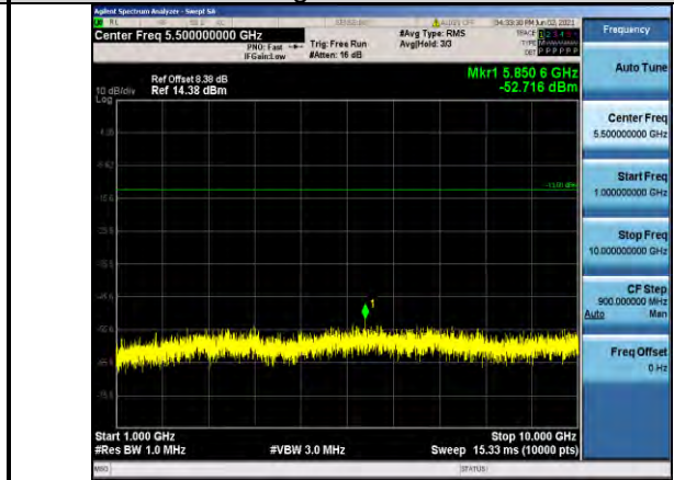
Band71-15MHz-16QAM-133397-1RB#0- Range2:1000~10000MHz
