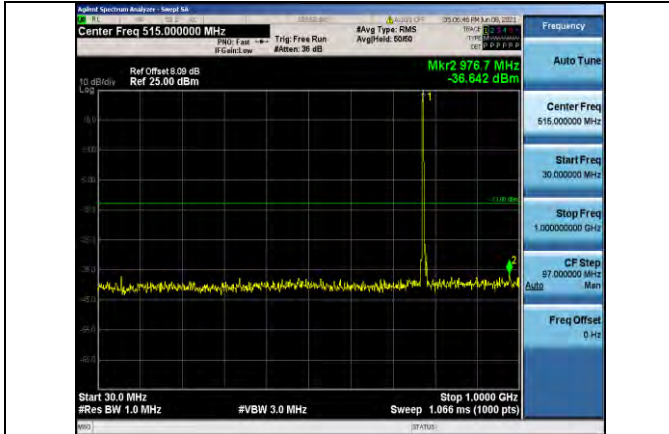
Band13-5MHz-QPSK-23205-1RB#0- Range1:30~1000MHz
