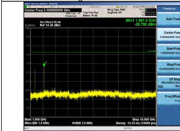
Band71-10MHz-16QAM-133172-1RB#0- Range2:1000~10000MHz
