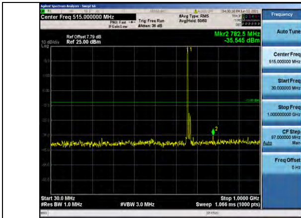
Band71-15MHz-QPSK-133197-1RB#0-Range1:30~1000MHz
