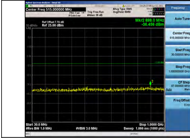
Band71-20MHz-16QAM-133322-1RB#0- Range1:30~1000MHz
