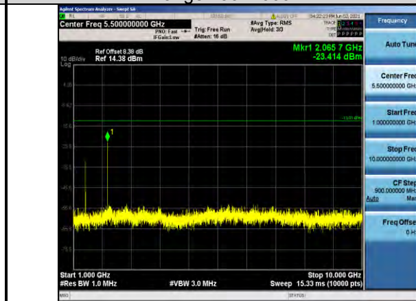
Band71-10MHz-16QAM-133422-1RB#0- Range2:1000~10000MHz
