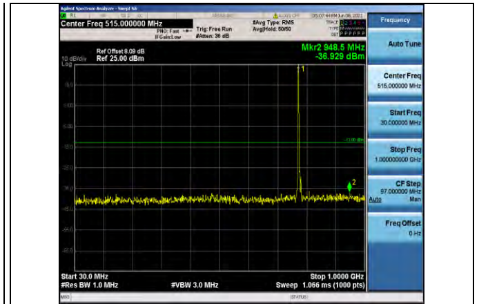
Band13-5MHz-16QAM-23205-1RB#0- Range1:30~1000MHz
