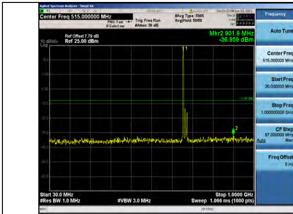
Band71-20MHz-QPSK-133222-1RB#0-Range1:30~1000MHz
