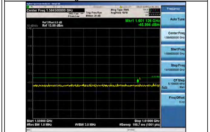
Band13-5MHz-QPSK-23205-1RB#0- Range3:1559~1610MHz
