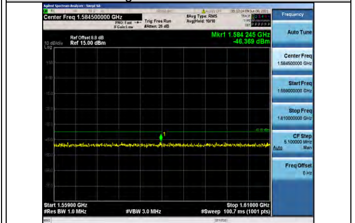
Band13-5MHz-16QAM-23255-1RB#0- Range3:1559~1610MHz
