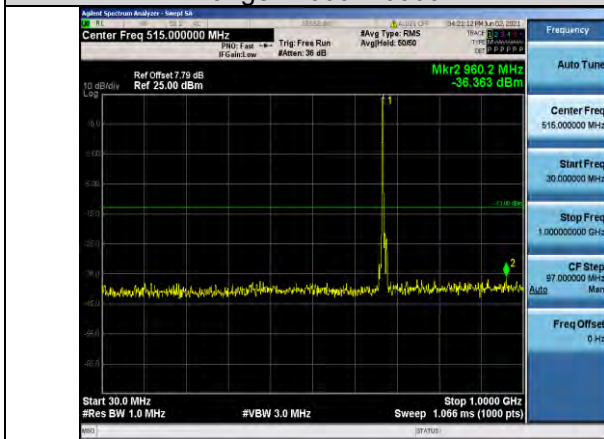
Band71-10MHz-16QAM-133297-1RB#0- Range1:30~1000MHz
