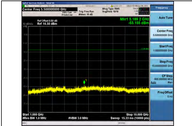
Band13-5MHz-16QAM-23205-1RB#0- Range2: 1000~10000MHz
