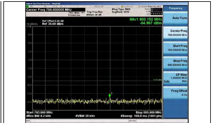
Band13-5MHz-16QAM-23255-1RB#0- Range5:793~805MHz
