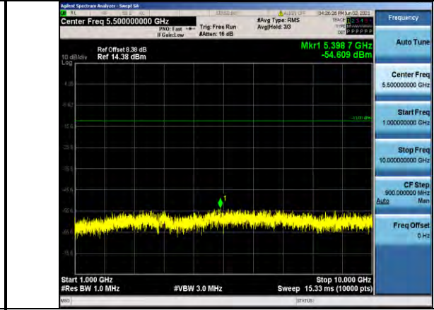
Band71-20MHz-16QAM-133372-1RB#0- Range2:1000~10000MHz
