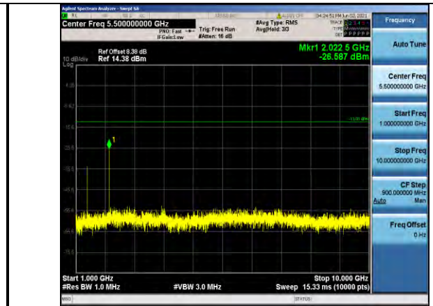
Band71-20MHz-QPSK-133322-1RB#0-Range2:1000~10000MHz
