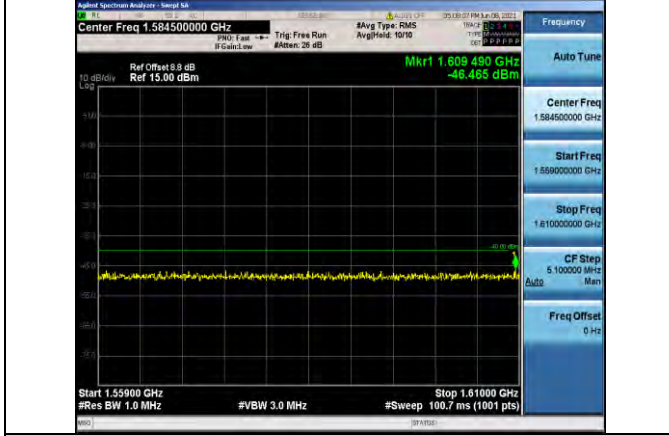
Band13-5MHz-16QAM-23205-1RB#0- Range3: 1559~1610MHz
