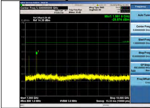
Band71-15MHz-QPSK-133197-1RB#0-Range2:1000~10000MHz
