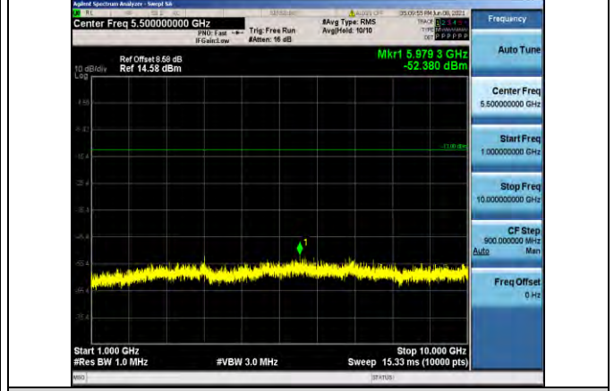
Band13-5MHz-16QAM-23230-1RB#0- Range2: 1000~10000MHz
