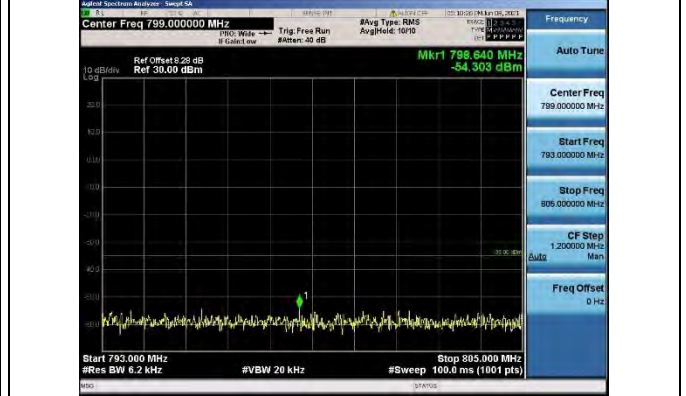
Band13-5MHz-16QAM-23230-1RB#0- Range5: 793~805MHz
