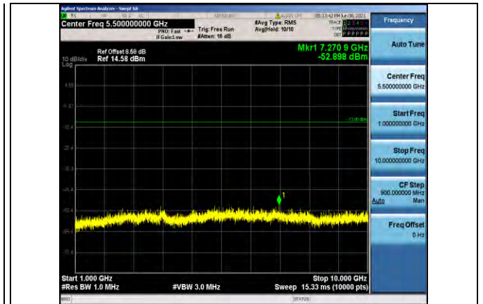
Band13-10MHz-QPSK-23230-1RB#0- Range2:1000~10000MHz
