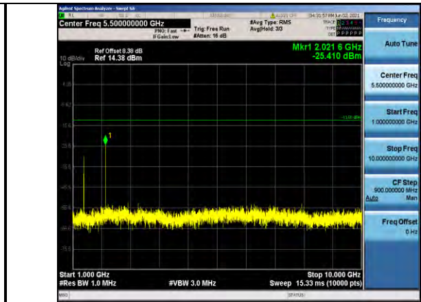
Band71-15MHz-QPSK-133297-1RB#0-Range2:1000~10000MHz
