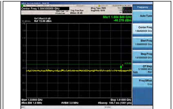
Band 13-5MHz-QPSK-23230-1RB#0-Range3:1559~1610MHz
