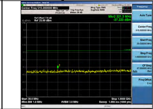
Band71-15MHz-16QAM-133397-1RB#0- Range1:30~1000MHz
