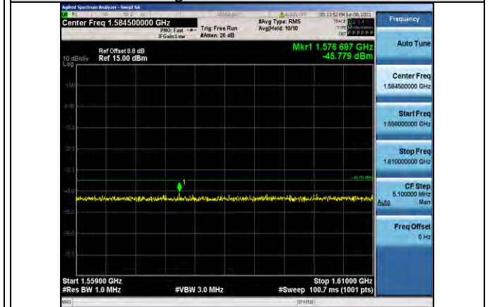
Band13-10MHz-QPSK-23230-1RB#0- Range3:1559~1610MHz
