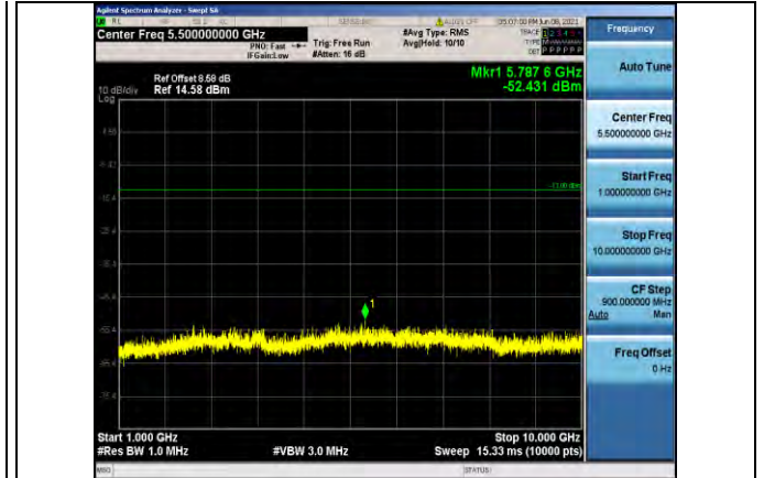
Band13-5MHz-QPSK-23205-1RB#0- Range2:1000~10000MHz
