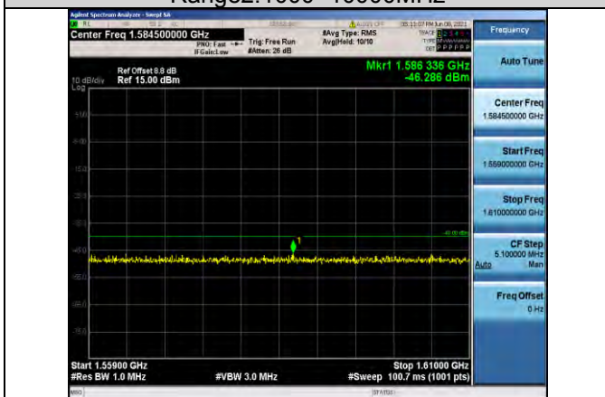
Band13-5MHz-QPSK-23255-1RB#0- Range3:1559~1610MHz
