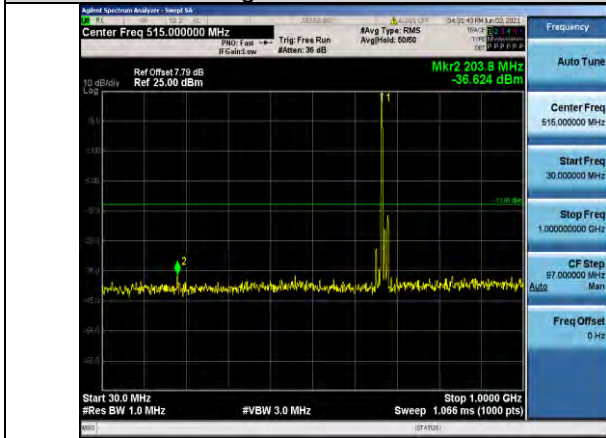
Band71-15MHz-QPSK-133297-1RB#0-Range1:30~1000MHz
