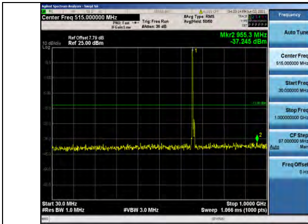
Band71-10MHz-16QAM-133172-1RB#0- Range1:30~1000MHz
