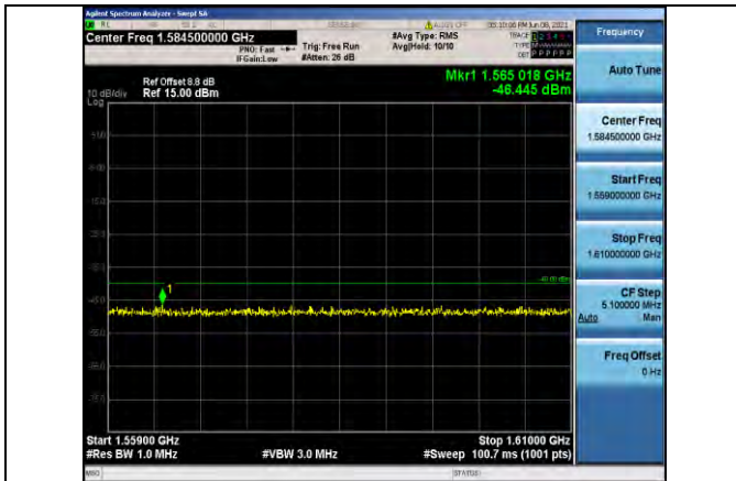
Band13-5MHz-16QAM-23230-1RB#0- Range3:1559~1610MHz
