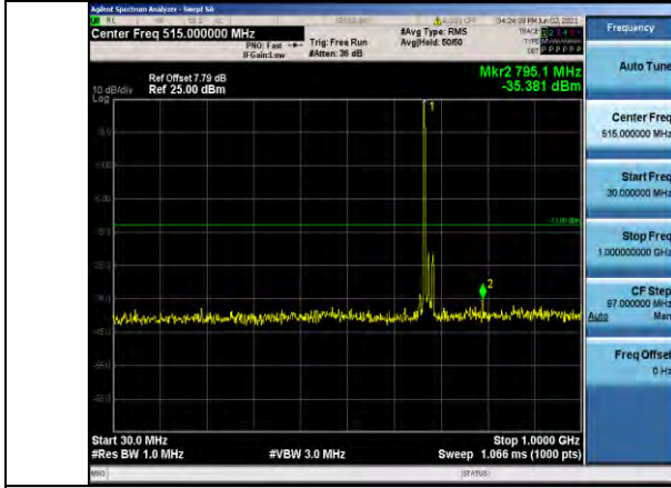
Band71-20MHz-QPSK-133322-1RB#0-Range1:30~1000MHz
