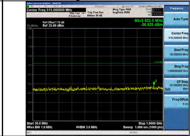
Band71-20MHz-16QAM-133372-1RB#0- Range1:30~1000MHz
