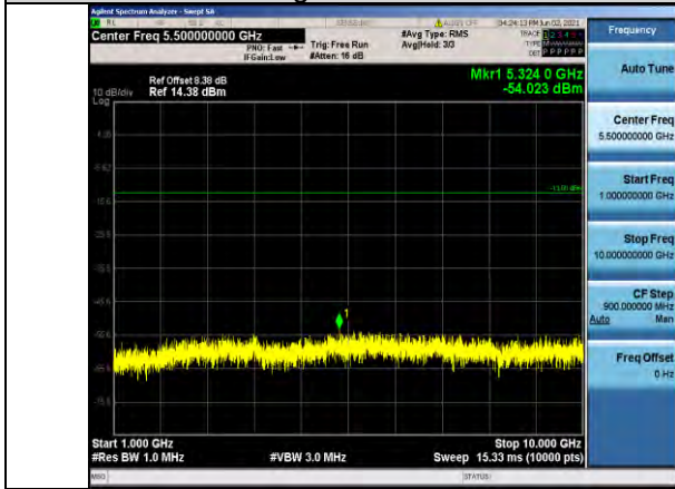
Band71-20MHz-16QAM-133222-1RB#0- Range2:1000~10000MHz
