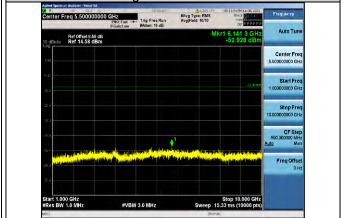
Band13-5MHz-16QAM-23255-1RB#0- Range2:1000~10000MHz
