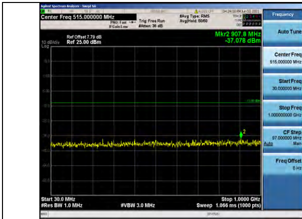
Band71-20MHz-16QAM-133222-1RB#0- Range1:30~1000MHz
