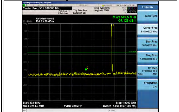
Band13-10MHz-16QAM-23230-1RB#0- Range1:30~1000MHz
