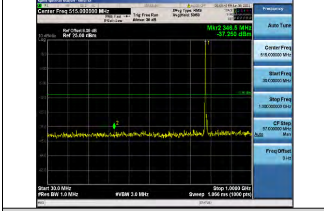
Band13-5MHz-16QAM-23230-1RB#0- Range1: 30~1000MHz
