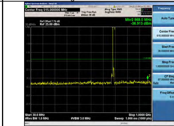
Band71-10MHz-16QAM-133422-1RB#0- Range1:30~1000MHz
