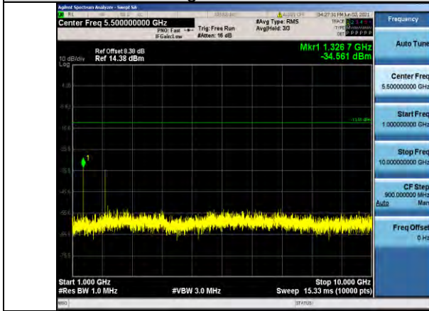
Band71-5MHz-16QAM-133147-1RB#0- Range2:1000~10000MHz
