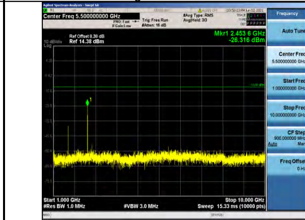
Band26-3MHz-16QAM-26740-1RB#0- Range2:1000~10000MHz
