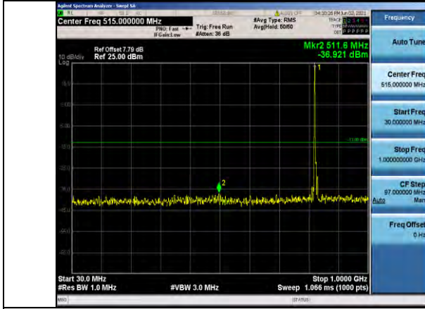
Band5-5MHz-16QAM-20425-1RB#0-Range1:30~1000MHz
