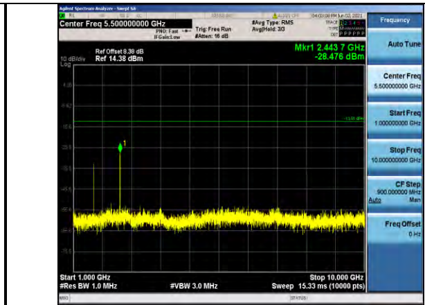
Band26-10MHz-QPSK-26740-1RB#0- Range2:1000~10000MHz
