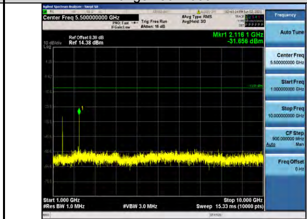
Band12-5MHz-QPSK-23095-1RB#0-Range2:1000~10000MHz
