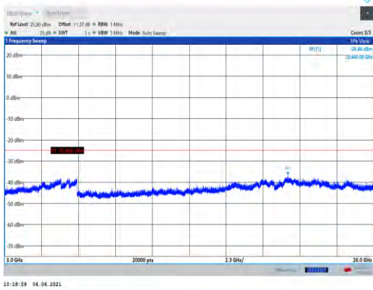
Band41-20MHz-16QAM-41490-1RB#0- Range3:3000~26000MHz
