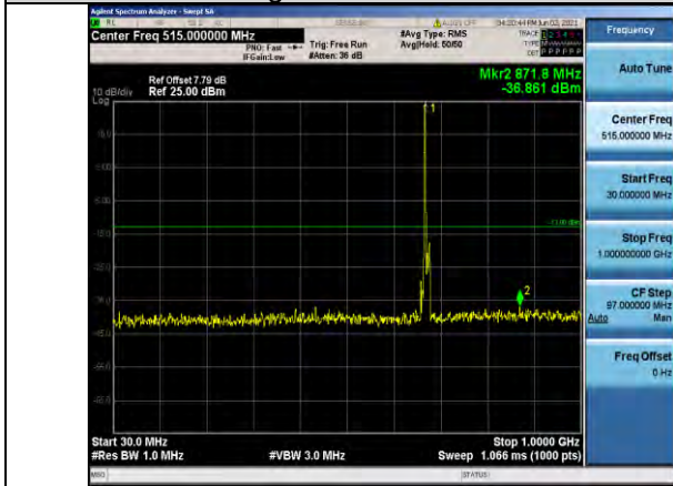
Band71-10MHz-QPSK-133297-1RB#0- Range1:30~1000MHz
