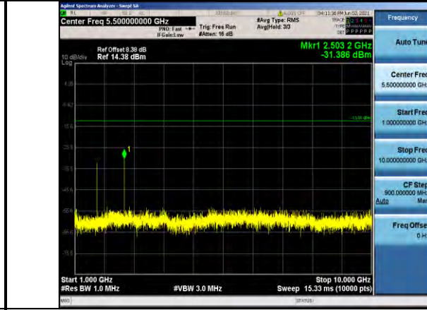
Band5-5MHz-16QAM-20525-1RB#0-Range2:1000~10000MHz
