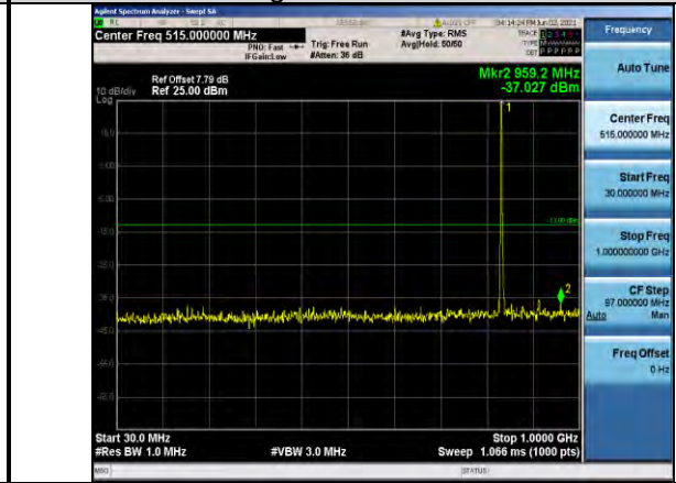
Band5-3MHz-16QAM-20525-1RB#0- Range1:30~1000MHz
