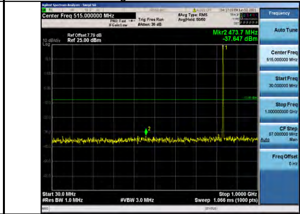
Band5-1.4MHz-16QAM-20525-1RB#0- Range1:30~1000MHz
