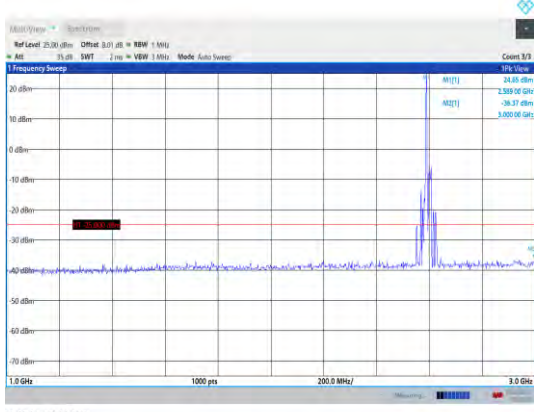
Band41-10MHz-16QAM-40620-1RB#0- Range2:1000~3000MHz
