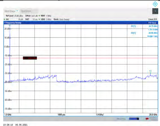
Band66-3MHz-QPSK-132322-1RB#0- Range2:1000~20000MHz
