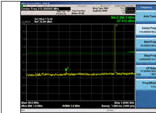
Band26-1.4MHz-16QAM-26783-1RB#0- Range1:30~1000MHz
