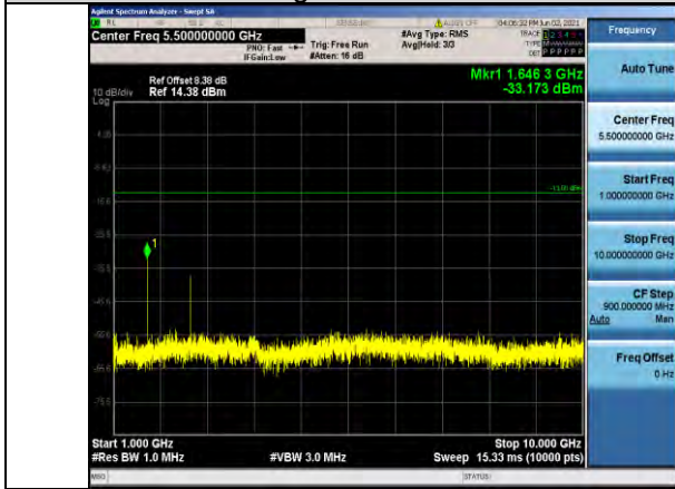
Band26-1.4MHz-16QAM-26783-1RB#0- Range2:1000~10000MHz
