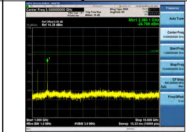
Band71-5MHz-16QAM-133447-1RB#0- Range2:1000~10000MHz
