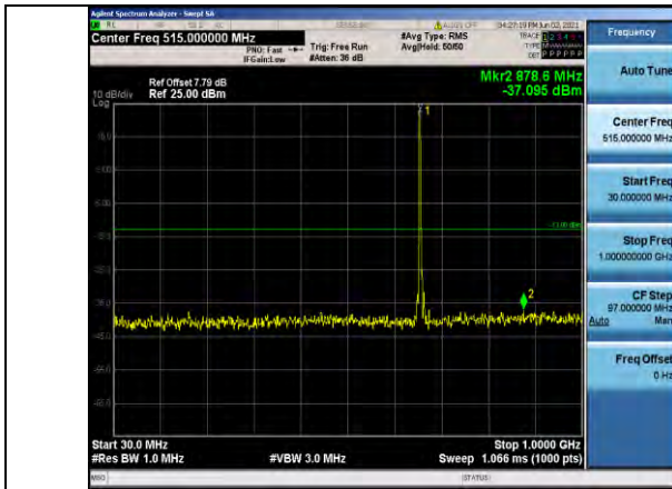
Band71-5MHz-16QAM-133147-1RB#0- Range1:30~1000MHz
