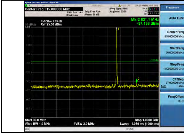
Band71-5MHz-QPSK-133297-1RB#0-Range1:30~1000MHz
