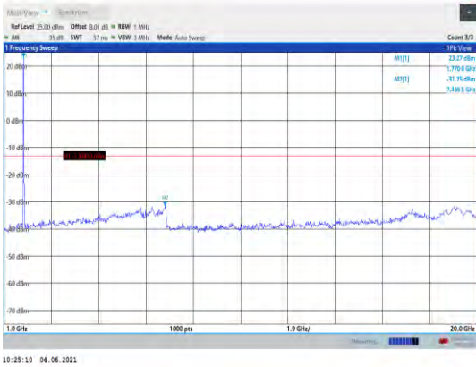
Band66-3MHz-16QAM-132657-1RB#0- Range2:1000~20000MHz
