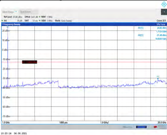
Band66-1.4MHz-16QAM-131979-1RB#0-Range2:1000~20000MHz
