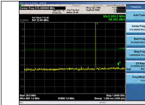
Band12-1.4MHz-16QAM-23173-1RB#0- Range1:30~1000MHz
