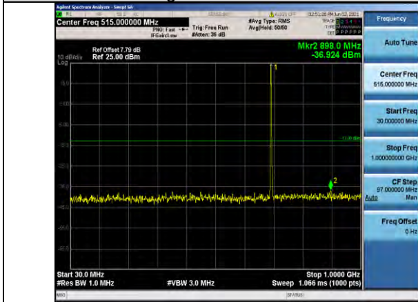
Band12-3MHz-16QAM-23025-1RB#0- Range1:30~1000MHz
