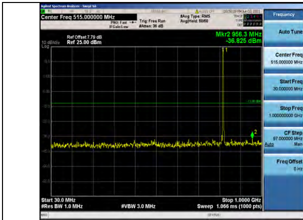
Band26-3MHz-QPSK-26775-1RB#0- Range1:30~1000MHz
