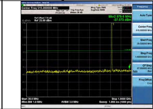
Band26-3MHz-QPSK-26740-1RB#0- Range1:30~1000MHz
