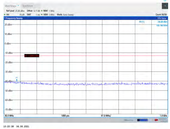
Band66-1.4MHz-QPSK-132322-1RB#0- Range1:30~1000MHz
