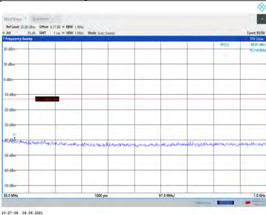
Band66-5MHz-16QAM-131997-1RB#0- Range1:30~1000MHz
