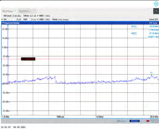
Band66-1.4MHz-16QAM-132665-1RB#0- Range2:1000~20000MHz
