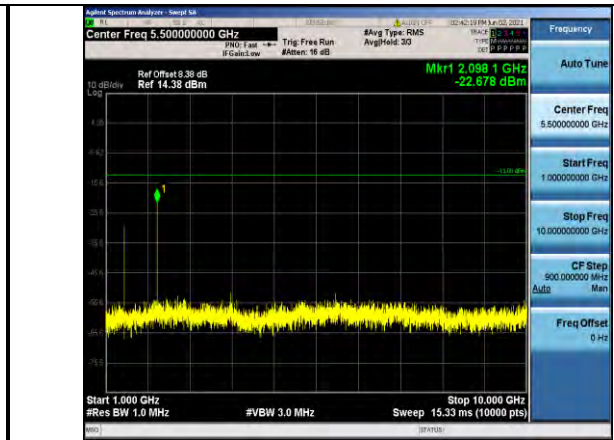
Band12-5MHz-QPSK-23035-1RB#0-Range2:1000~10000MHz
