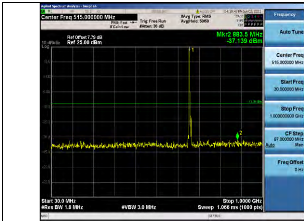
Band71-10MHz-QPSK-133172-1RB#0- Range1:30~1000MHz
