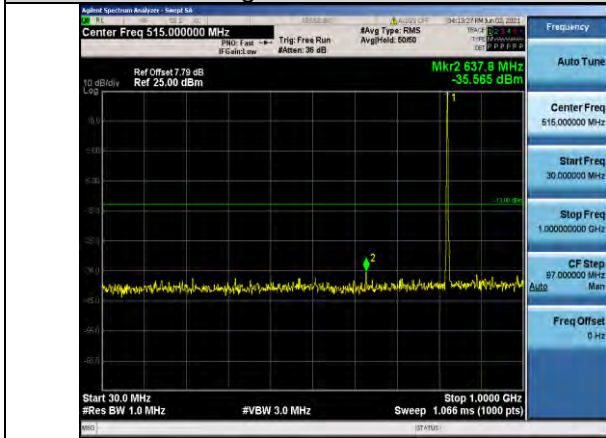
Band5-3MHz-16QAM-20415-1RB#0- Range1:30~1000MHz
