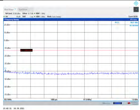
Band66-20MHz-16QAM-132322-1RB#0- Range1:30~1000MHz
