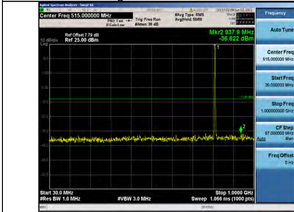
Band26-3MHz-16QAM-26705-1RB#0- Range1:30~1000MHz
