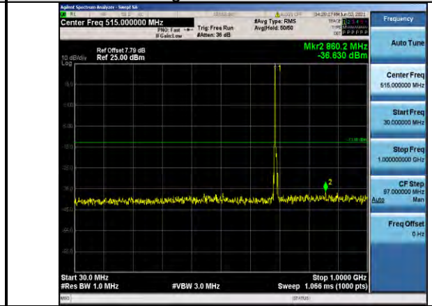
Band71-5MHz-16QAM-133447-1RB#0- Range1:30~1000MHz
