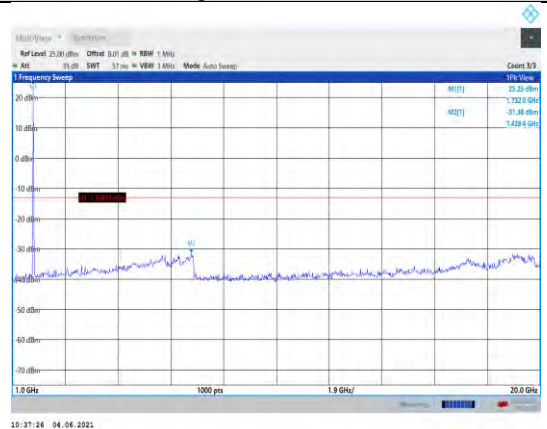
Band66-15MHz-16QAM-132322-1RB#0- Range2:1000~20000MHz
