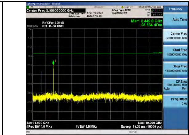
Band26-1.4MHz-16QAM-26697-1RB#0- Range2:1000~10000MHz
