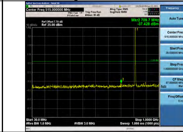
Band26-3MHz-16QAM-26740-1RB#0- Range1:30~1000MHz
