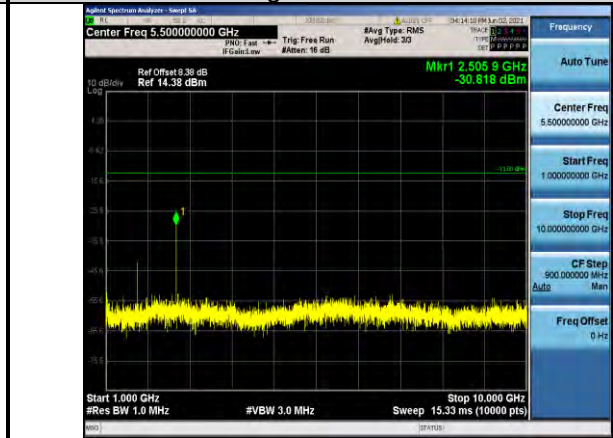
Band5-3MHz-QPSK-20525-1RB#0- Range2:1000~10000MHz
