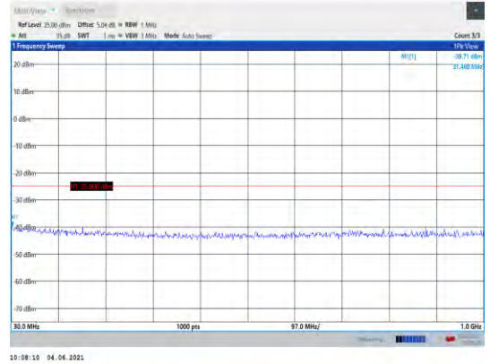
Band41-15MHz-QPSK-40620-1RB#0- Range1:30~1000MHz
