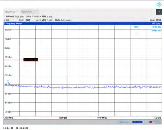
Band66-3MHz-16QAM-132322-1RB#0- Range1:30~1000MHz
