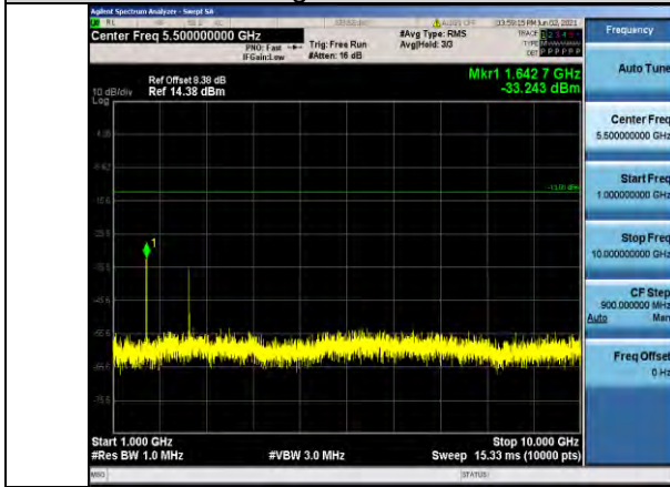
Band26-3MHz-16QAM-26775-1RB#0- Range2:1000~10000MHz
