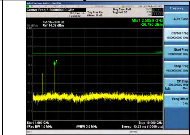
Band5-3MHz-16QAM-20525-1RB#0- Range2:1000~10000MHz
