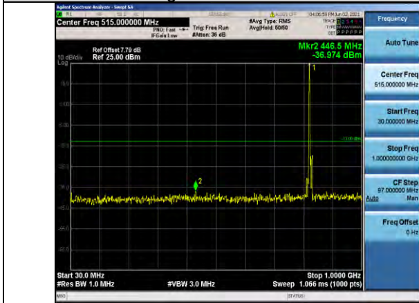
Band5-10MHz-QPSK-20450-1RB#0- Range1:30~1000MHz
