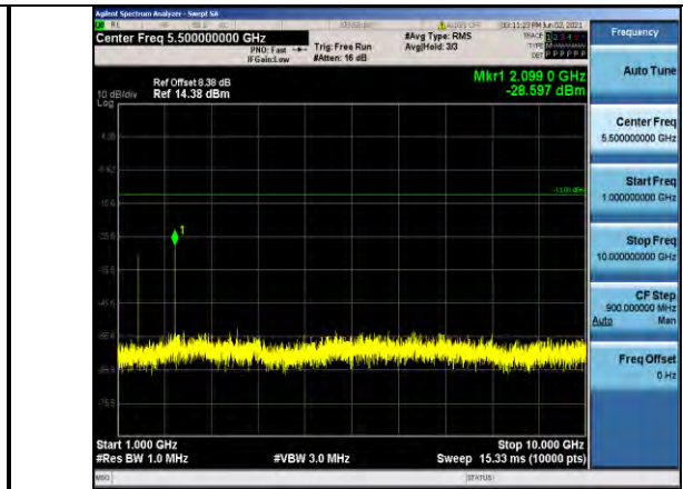
Band12-10MHz-16QAM-23060-1RB#0-Range2:1000~10000MHz
