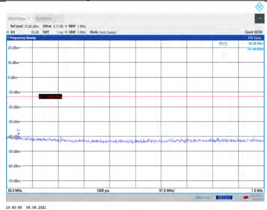
Band66-20MHz-16QAM-132572-1RB#0- Range1:30~1000MHz
