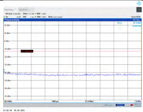
Band66-10MHz-16QAM-132322-1RB#0- Range1:30~1000MHz
