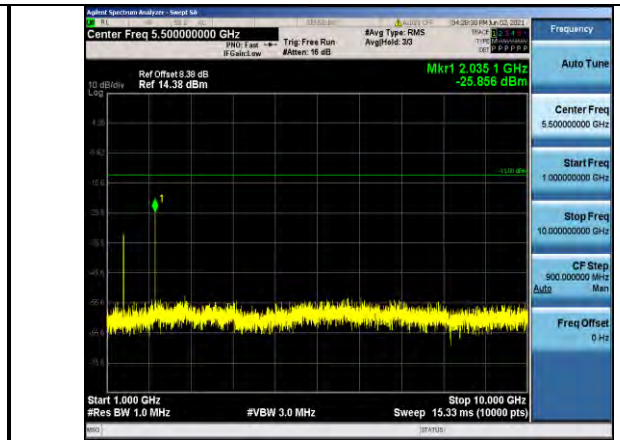
Band71-5MHz-16QAM-133297-1RB#0- Range2:1000~10000MHz
