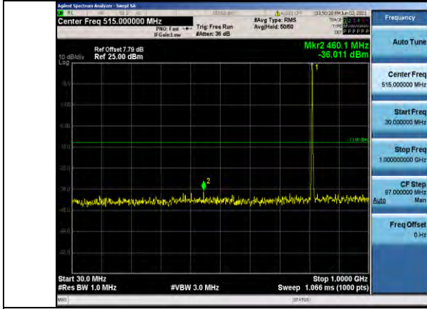
Band26-3MHz-QPSK-26705-1RB#0- Range1:30~1000MHz
