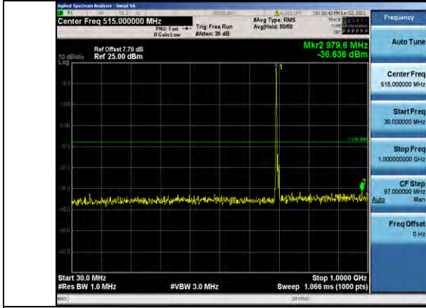
Band12-10MHz-QPSK-23060-1RB#0- Range1:30~1000MHz
