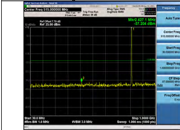
Band26-1.4MHz-QPSK-26697-1RB#0-Range1:30~1000MHz
