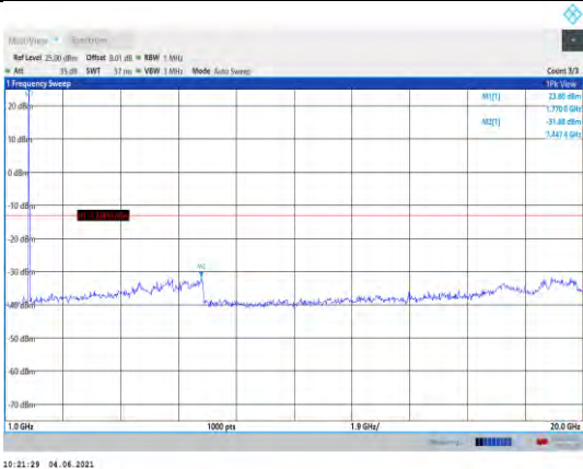
Band66-1.4MHz-QPSK-132665-1RB#0-Range2:1000~20000MHz
