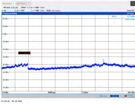
Band41-15MHz-QPSK-40620-1RB#0- Range3:3000~26000MHz
