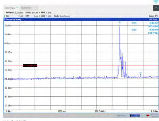
Band41-20MHz-16QAM-39750-1RB#0- Range2:1000~3000MHz
