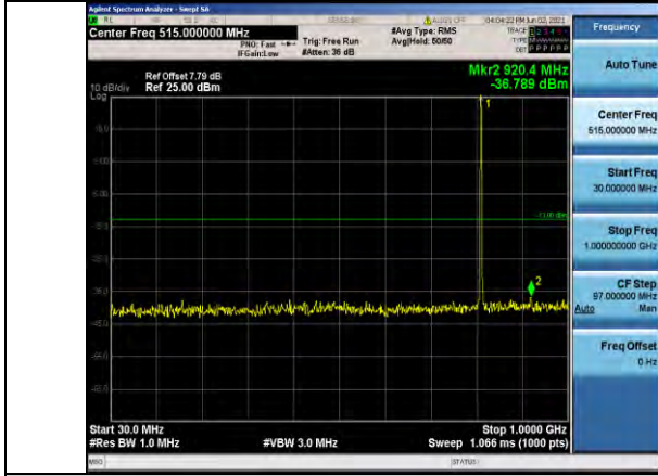
Band26-1.4MHz-16QAM-26697-1RB#0- Range1:30~1000MHz
