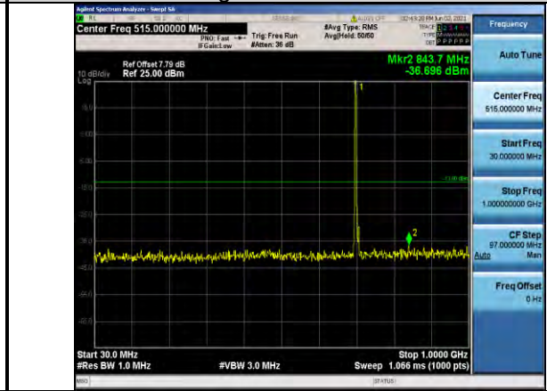
Band12-5MHz-16QAM-23095-1RB#0- Range1:30~1000MHz
