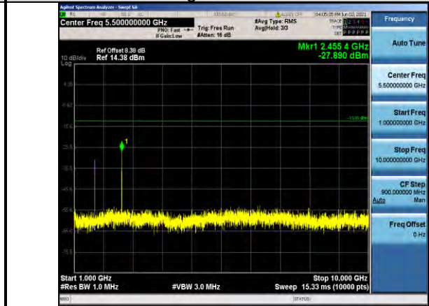
Band26-1.4MHz-QPSK-26740-1RB#0-Range2:1000~10000MHz
