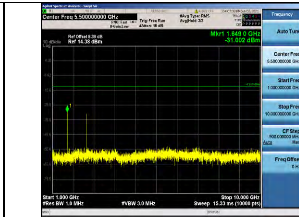
Band5-10MHz-16QAM-20450-1RB#0-Range2:1000~10000MHz
