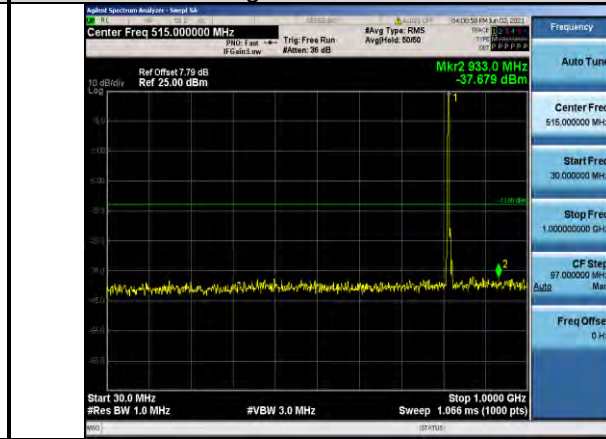
Band26-5MHz-QPSK-26740-1RB#0- Range1:30~1000MHz
