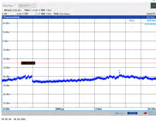
Band41-10MHz-16QAM-39700-1RB#0- Range3:3000~26000MHz
