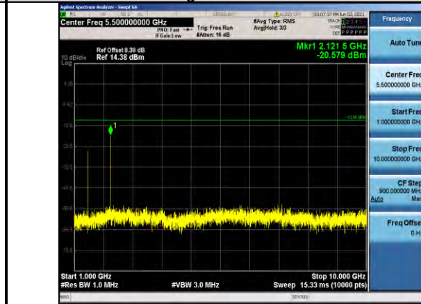
Band12-1.4MHz-QPSK-23095-1RB#0-Range2:1000~10000MHz
