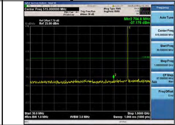
Band26-1.4MHz-16QAM-26740-1RB#0- Range1:30~1000MHz
