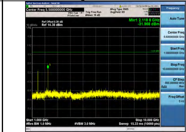
Band12-3MHz-16QAM-23095-1RB#0- Range2:1000~10000MHz
