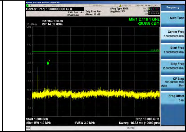
Band12-5MHz-16QAM-23095-1RB#0- Range2:1000~10000MHz
