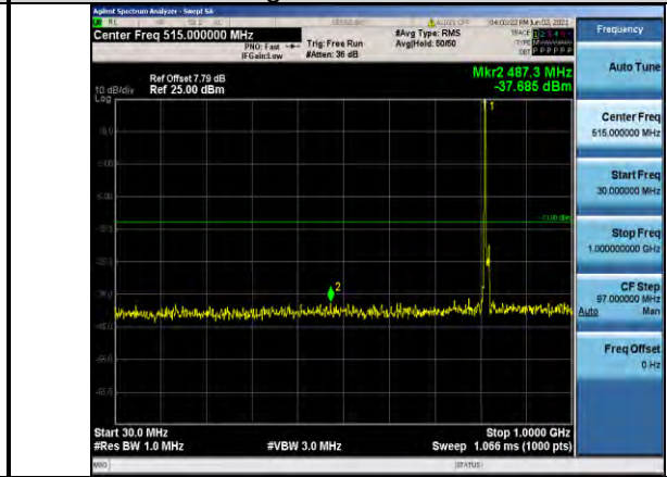
Band26-10MHz-16QAM-26740-1RB#0- Range1:30~1000MHz
