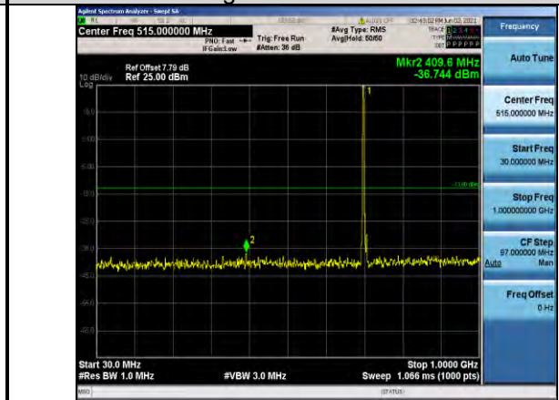
Band12-5MHz-QPSK-23095-1RB#0-Range1:30~1000MHz
