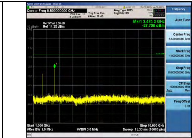
Band5-10MHz-QPSK-20450-1RB#0- Range2:1000~10000MHz
