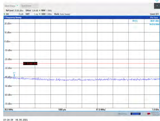
Band41-20MHz-16QAM-39750-1RB#0- Range1:30~1000MHz
