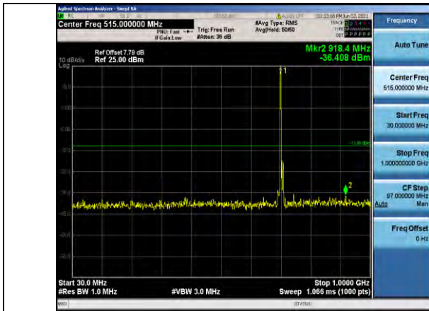
Band12-10MHz-16QAM-23130-1RB#0-Range1:30~1000MHz
