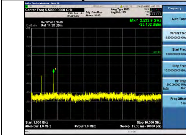
Band5-5MHz-QPSK-20625-1RB#0-Range2:1000~10000MHz
