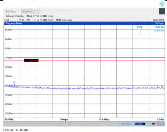
Band66-10MHz-QPSK-132322-1RB#0-Range1:30~1000MHz
