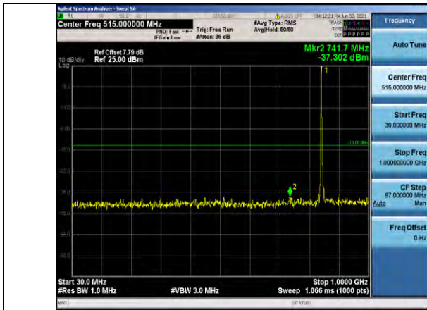
Band5-5MHz-16QAM-20625-1RB#0- Range1:30~1000MHz
