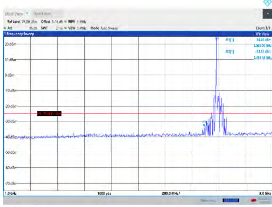
Band41-20MHz-16QAM-40620-1RB#0-Range2:1000~3000MHz
