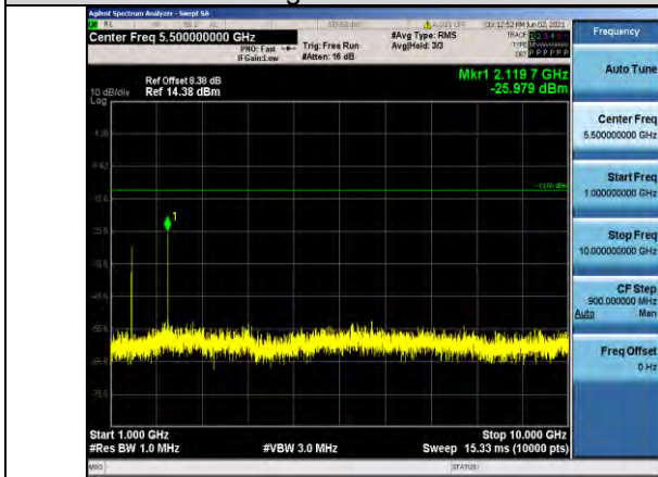
Band12-10MHz-QPSK-23130-1RB#0-Range2:1000~10000MHz
