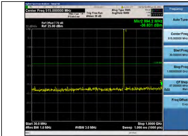
Band12-3MHz-QPSK-23165-1RB#0- Range1:30~1000MHz
