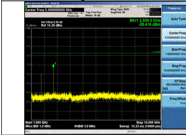
Band5-3MHz-16QAM-20635-1RB#0- Range2:1000~10000MHz
