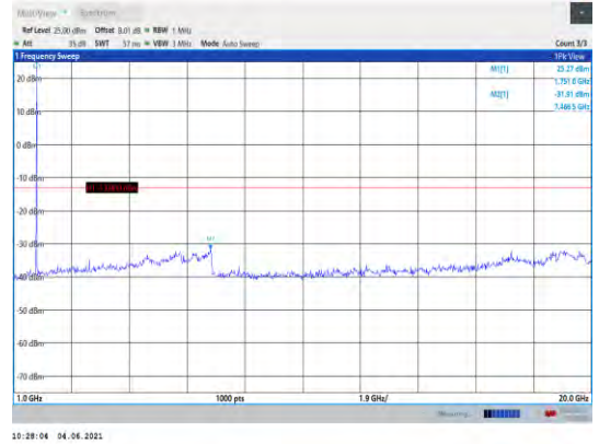
Band66-5MHz-QPSK-132322-1RB#0- Range2:1000~20000MHz
