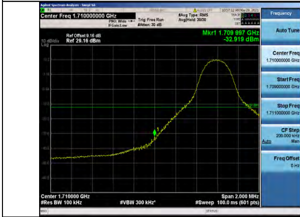
Band66-10MHz-16QAM-132022-1RB#0
