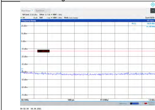
Band4-1.4MHz-QPSK-20175-1RB#0- Range1:30~1000MHz
