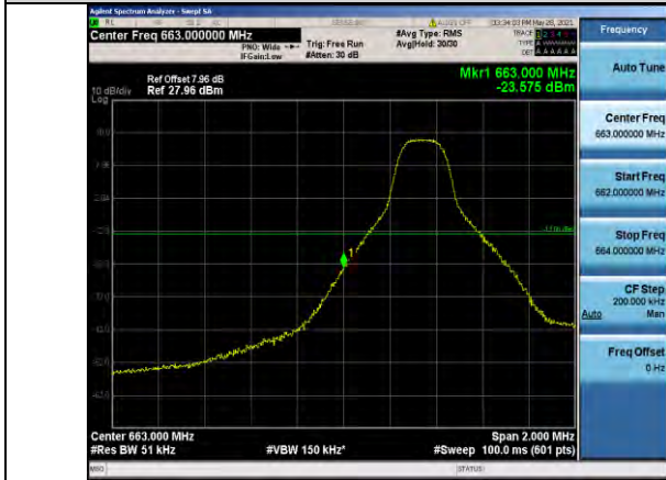
Band71-5MHz-16QAM-133147-1RB#0
