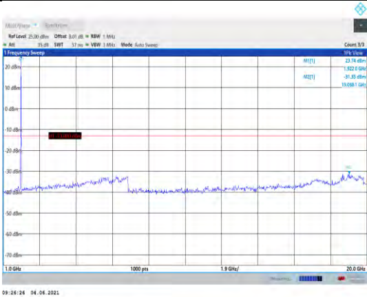
Band25-1.4MHz-16QAM-26683-1RB#0- Range2:1000~20000MHz
