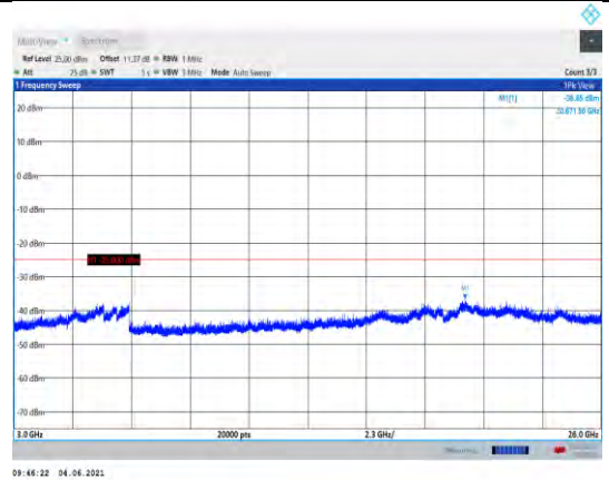
Band41-5MHz-QPSK-39675-1RB#0- Range3:3000~26000MHz
