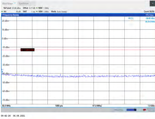
Band25-20MHz-QPSK-26140-1RB#0- Range1:30~1000MHz
