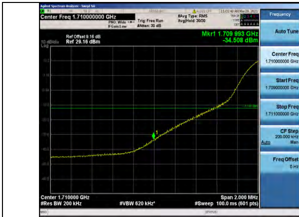
Band66-20MHz-16QAM-132072-1RB#0
