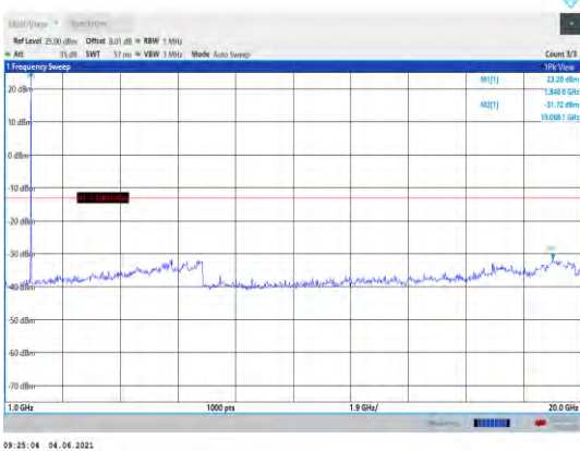
Band25-1.4MHz-16QAM-26047-1RB#0- Range2:1000~20000MHz
