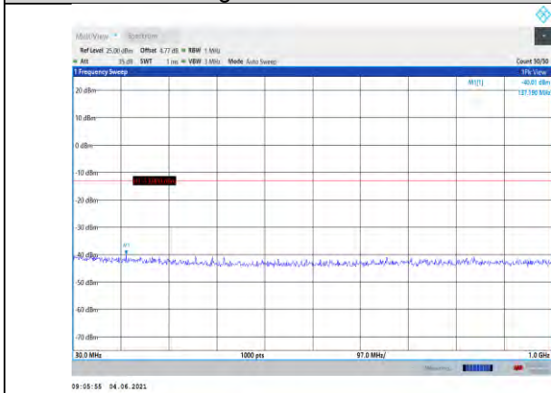
Band4-3MHz-QPSK-20175-1RB#0- Range1:30~1000MHz
