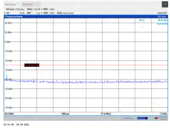
Band41-10MHz-QPSK-40620-1RB#0- Range1:30~1000MHz
