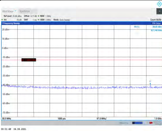
Band4-1.4MHz-16QAM-19957-1RB#0- Range1:30~1000MHz
