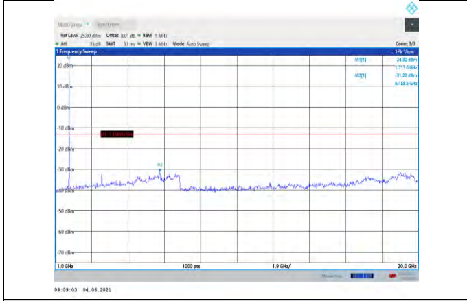
Band4-5MHz-16QAM-19975-1RB#0- Range2:1000~20000MHz
