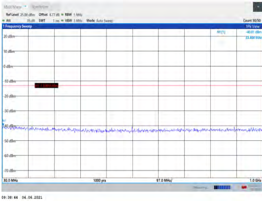
Band25-15MHz-QPSK-26115-1RB#0- Range1:30~1000MHz
