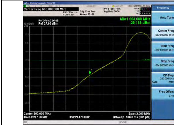
Band71-15MHz-QPSK-133197-1RB#0
