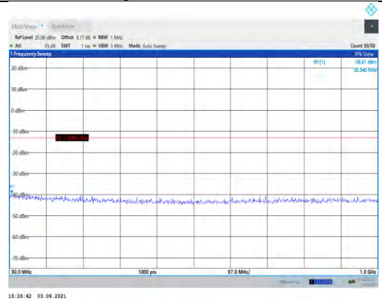
Band2-3MHz-QPSK-19185-1RB#0- Range1:30~1000MHz
