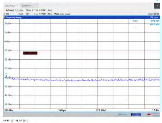
Band25-15MHz-16QAM-26365-1RB#0- Range1:30~1000MHz
