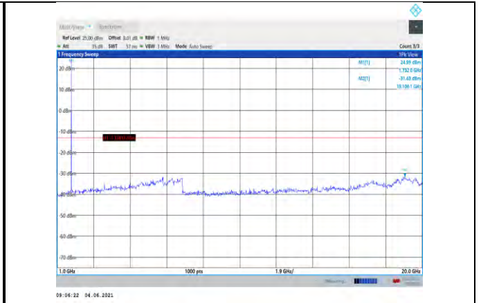
Band4-3MHz-16QAM-20175-1RB#0- Range2:1000~20000MHz
