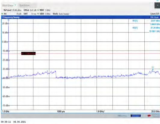
Band25-15MHz-16QAM-26115-1RB#0- Range2:1000~20000MHz
