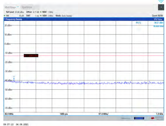
Band25-10MHz-16QAM-26640-1RB#0- Range1:30~1000MHz
