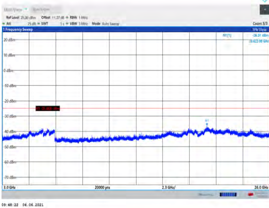
Band41-5MHz-QPSK-40620-1RB#0- Range3:3000~26000MHz
