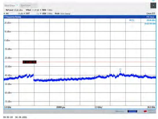
Band41-5MHz-QPSK-41565-1RB#0- Range3:3000~26000MHz
