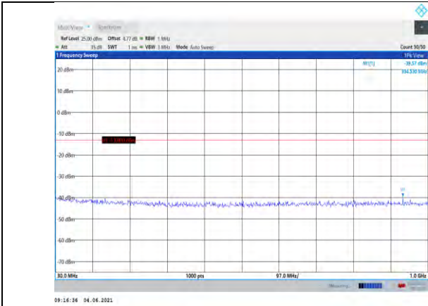
Band4-15MHz-QPSK-20025-1RB#0- Range1:30~1000MHz
