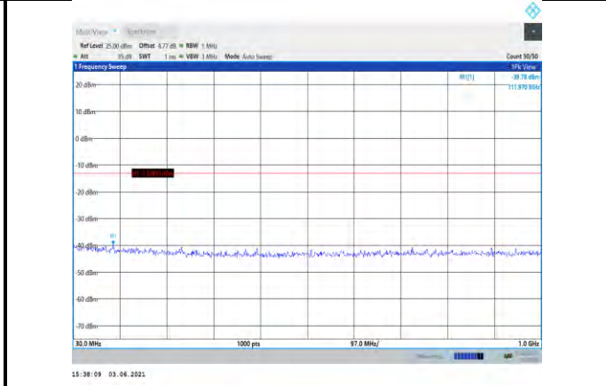
Band2-5MHz-16QAM-19175-1RB#0- Range1:30~1000MHz
