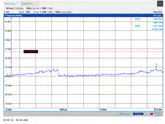
Band25-15MHz-16QAM-26365-1RB#0- Range2:1000~20000MHz
