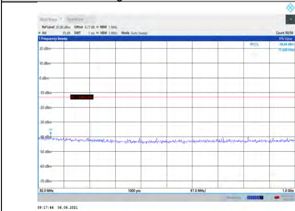
Band4-15MHz-QPSK-20175-1RB#0- Range1:30~1000MHz
