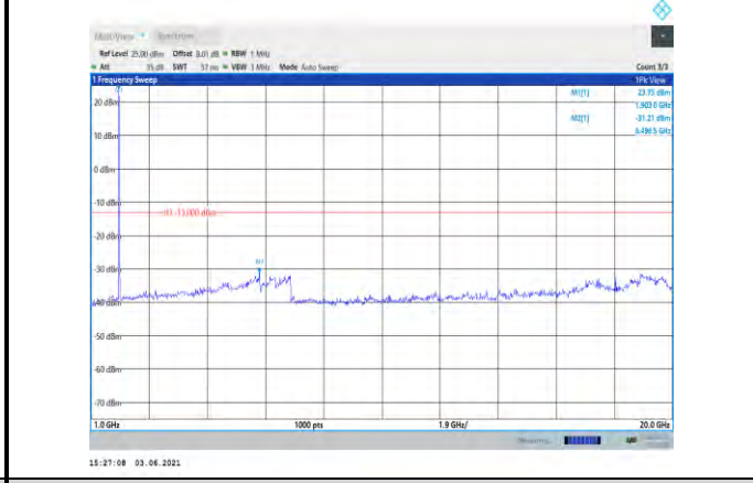
Band2-3MHz-16QAM-19185-1RB#0- Range2:1000~20000MHz
