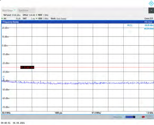
Band41-5MHz-QPSK-39675-1RB#0- Range1:30~1000MHz
