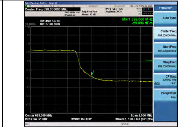
Band71-5MHz-16QAM-133447-25RB#0
