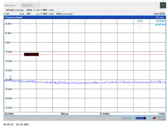
Band25-20MHz-16QAM-26365-1RB#0- Range1:30~1000MHz
