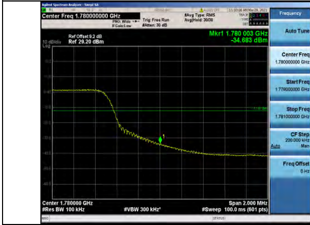
Band66-10MHz-QPSK-132622-50RB#0
