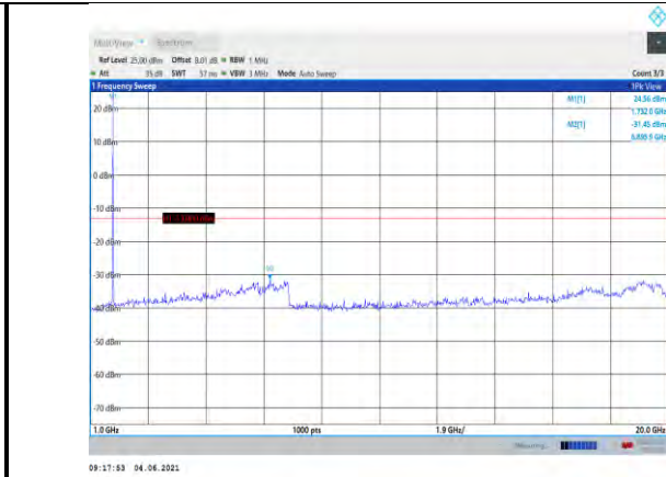
Band4-15MHz-QPSK-20175-1RB#0- Range2:1000~20000MHz
