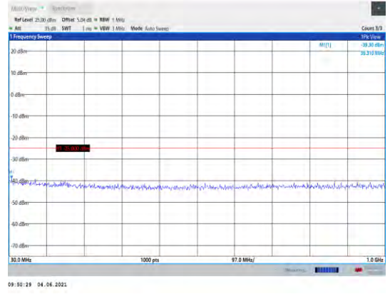
Band41-5MHz-16QAM-41565-1RB#0- Range1:30~1000MHz
