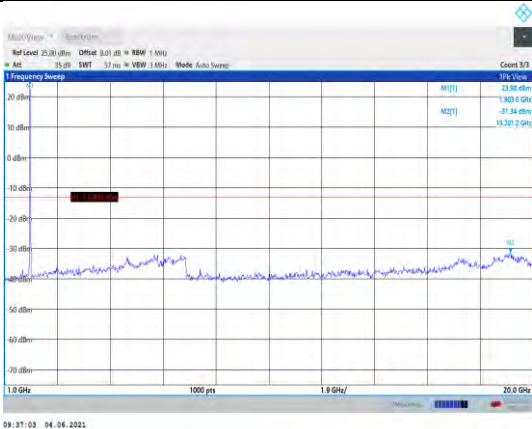
Band25-10MHz-QPSK-26640-1RB#0- Range2:1000~20000MHz
