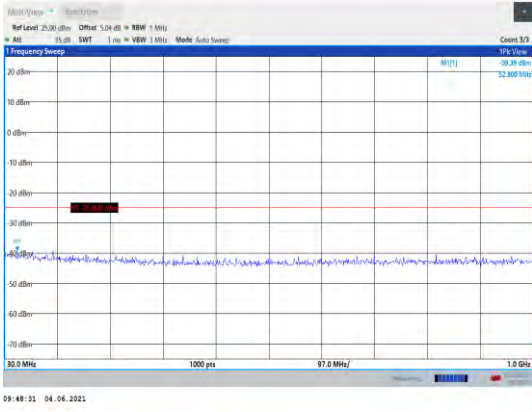
Band41-5MHz-16QAM-40620-1RB#0- Range1:30~1000MHz
