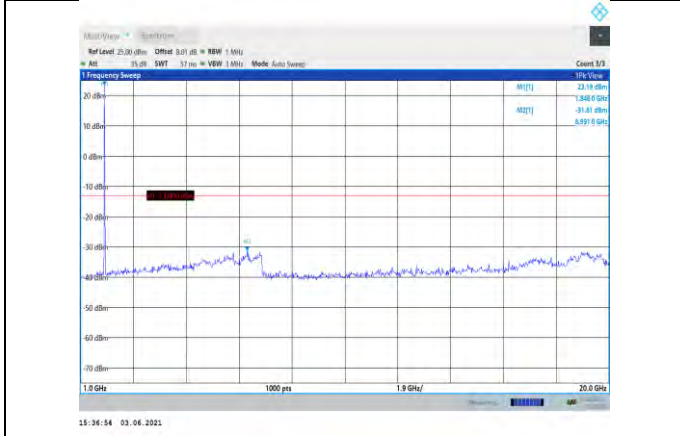
Band2-5MHz-16QAM-18625-1RB#0- Range2:1000~20000MHz
