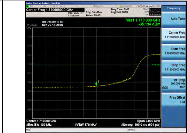
Band66-15MHz-16QAM-132047-75RB#0
