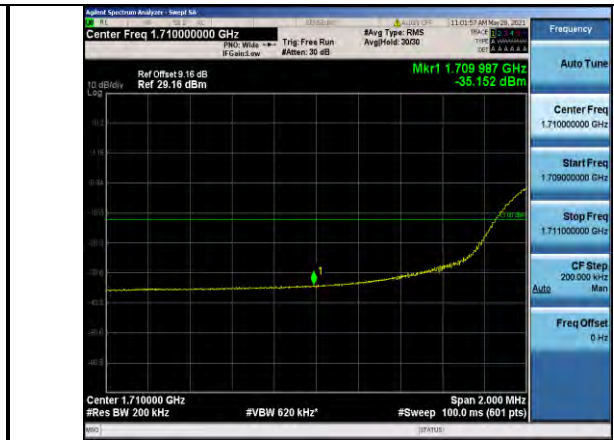
Band66-20MHz-QPSK-132072-100RB#0
