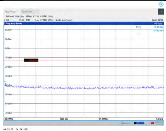
Band25-5MHz-16QAM-26665-1RB#0- Range1:30~1000MHz
