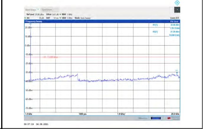
Band4-3MHz-16QAM-20385-1RB#0- Range2:1000~20000MHz
