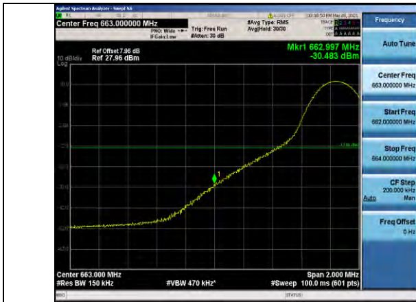
Band71-15MHz-16QAM-133197-1RB#0
