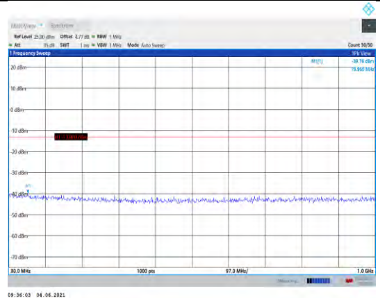
Band25-10MHz-16QAM-26365-1RB#0- Range1:30~1000MHz
