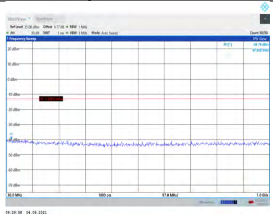
Band25-3MHz-QPSK-26675-1RB#0- Range1:30~1000MHz
