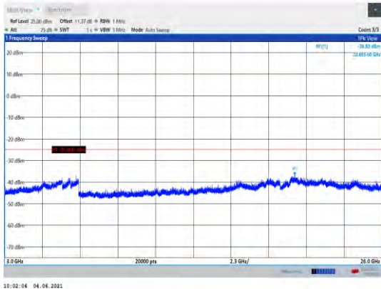
Band41-10MHz-QPSK-40620-1RB#0- Range3:3000~26000MHz
