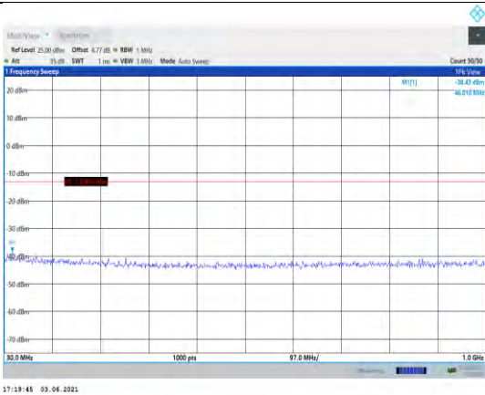
Band2-15MHz-16QAM-18675-1RB#0- Range1:30~1000MHz
