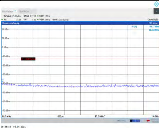
Band25-10MHz-16QAM-26090-1RB#0- Range1:30~1000MHz
