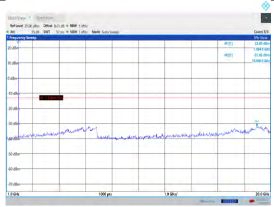
Band25-3MHz-16QAM-26365-1RB#0- Range2:1000~20000MHz
