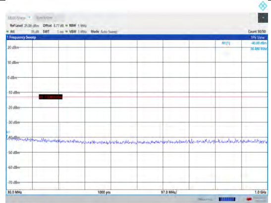
Band25-1.4MHz-QPSK-26683-1RB#0- Range1:30~1000MHz
