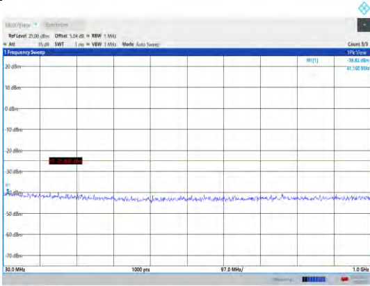
Band41-5MHz-QPSK-41565-1RB#0- Range1:30~1000MHz
