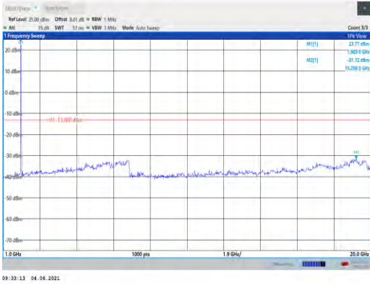
Band25-5MHz-16QAM-26665-1RB#0- Range2:1000~20000MHz
