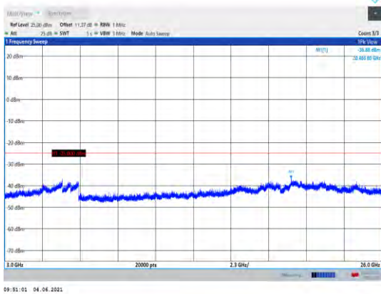
Band41-5MHz-16QAM-41565-1RB#0- Range3:3000~26000MHz
