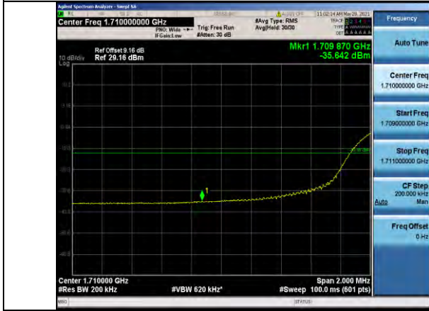
Band66-20MHz-16QAM-132072-100RB#0
