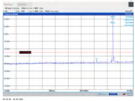
Band41-5MHz-16QAM-41565-1RB#0- Range2:1000~3000MHz
