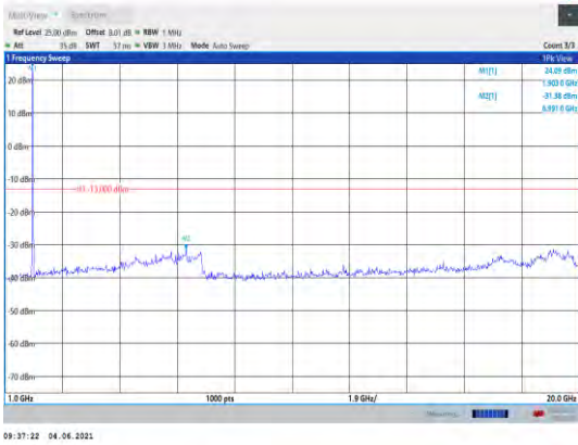
Band25-10MHz-16QAM-26640-1RB#0- Range2:1000~20000MHz
