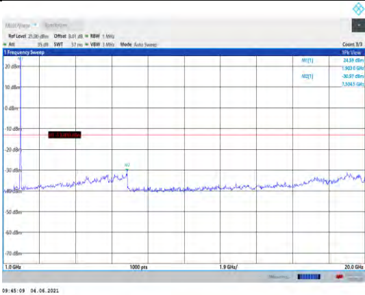
Band25-20MHz-16QAM-26590-1RB#0- Range2:1000~20000MHz
