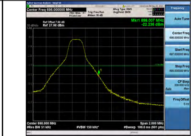
Band71-5MHz-16QAM-133447-1RB#24
