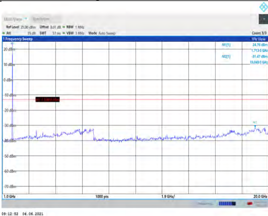
Band4-10MHz-16QAM-20000-1RB#0- Range2:1000~20000MHz
