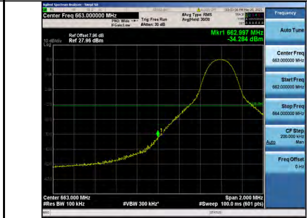
Band71-10MHz-16QAM-133172-1RB#0
