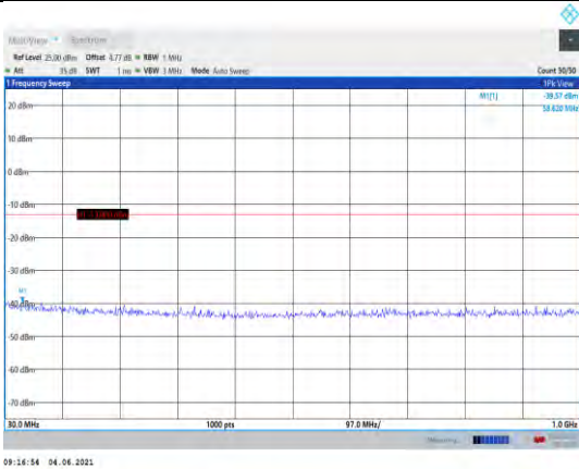
Band4-15MHz-16QAM-20025-1RB#0- Range1:30~1000MHz
