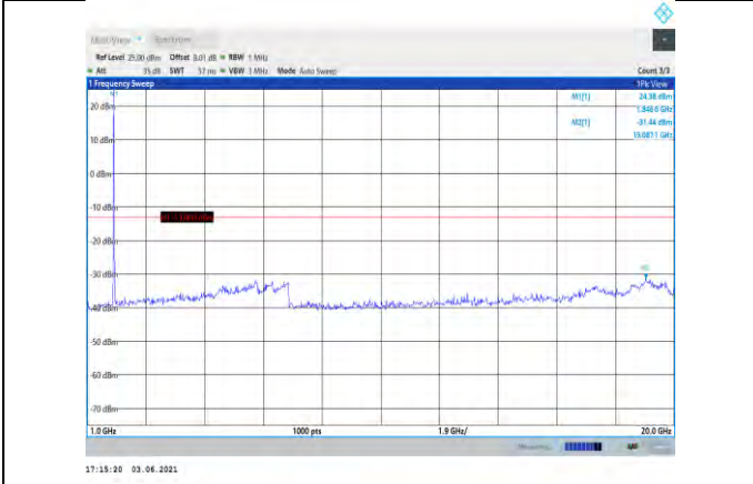
Band2-10MHz-QPSK-18650-1RB#0- Range2:1000~20000MHz
