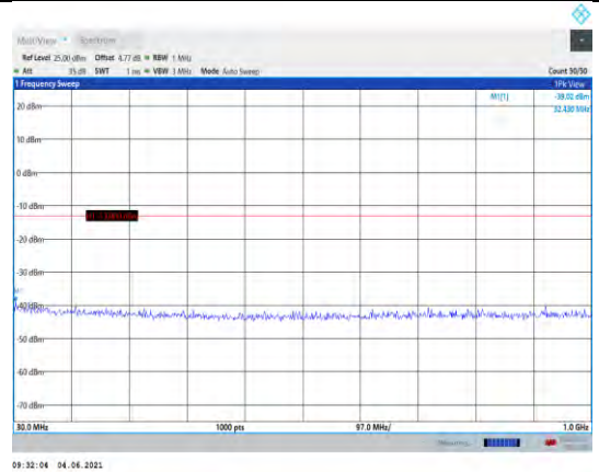
Band25-5MHz-QPSK-26365-1RB#0- Range1:30~1000MHz
