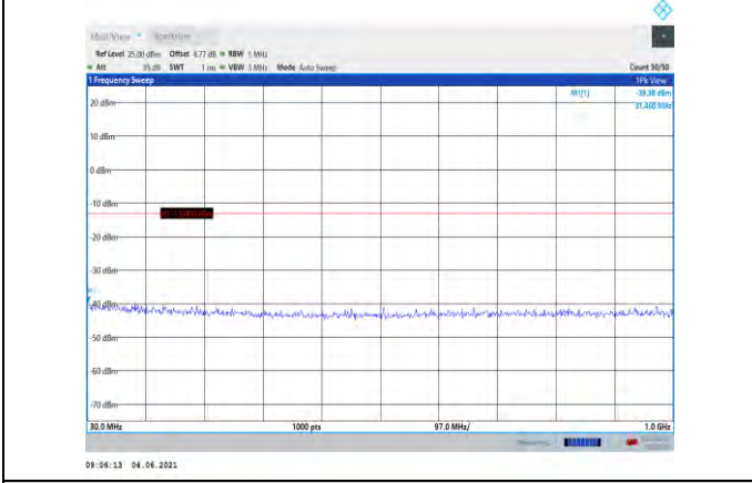
Band4-3MHz-16QAM-20175-1RB#0- Range1:30~1000MHz
