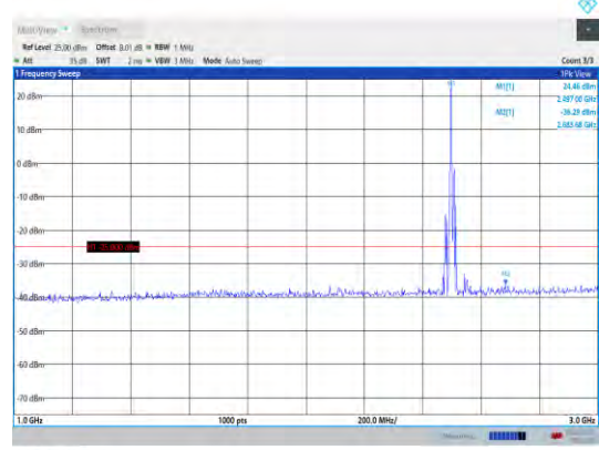
Band41-10MHz-16QAM-39700-1RB#0- Range2:1000~3000MHz
