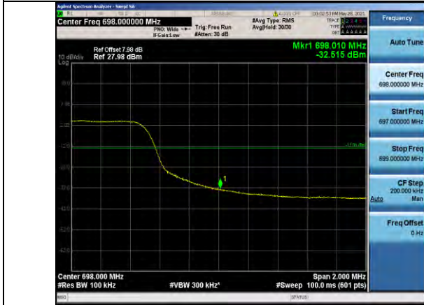
Band71-10MHz-16QAM-133422-50RB#0
