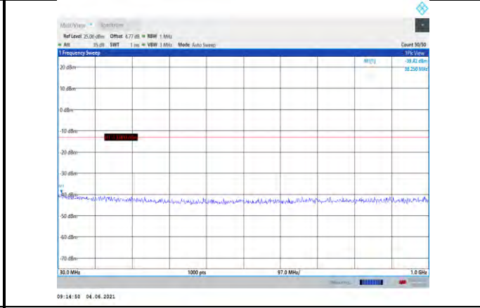
Band4-10MHz-QPSK-20350-1RB#0- Range1:30~1000MHz
