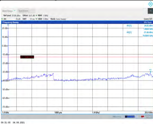
Band25-5MHz-16QAM-26065-1RB#0- Range2:1000~20000MHz
