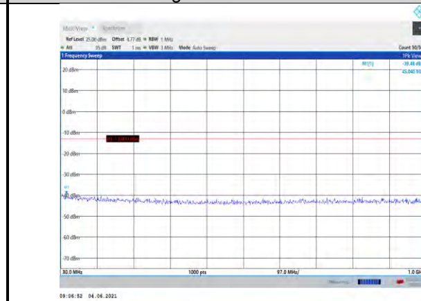
Band4-3MHz-QPSK-20385-1RB#0- Range1:30~1000MHz
