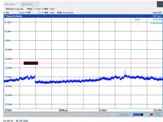
Band41-10MHz-QPSK-41540-1RB#0- Range3:3000~26000MHz
