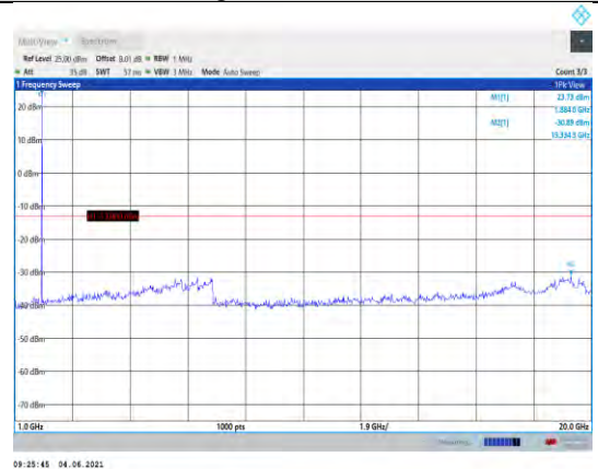
Band25-1.4MHz-16QAM-26365-1RB#0- Range2:1000~20000MHz
