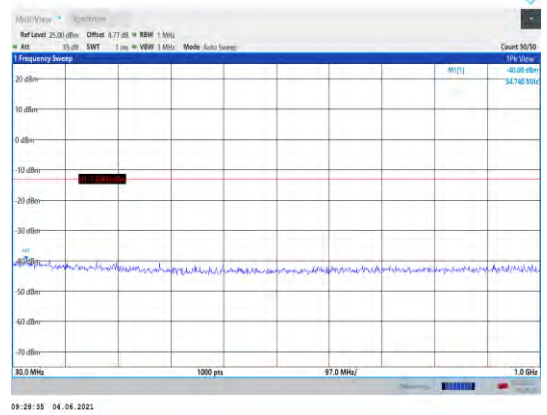
Band25-3MHz-16QAM-26365-1RB#0- Range1:30~1000MHz
