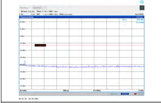
Band4-5MHz-16QAM-20175-1RB#0- Range1:30~1000MHz
