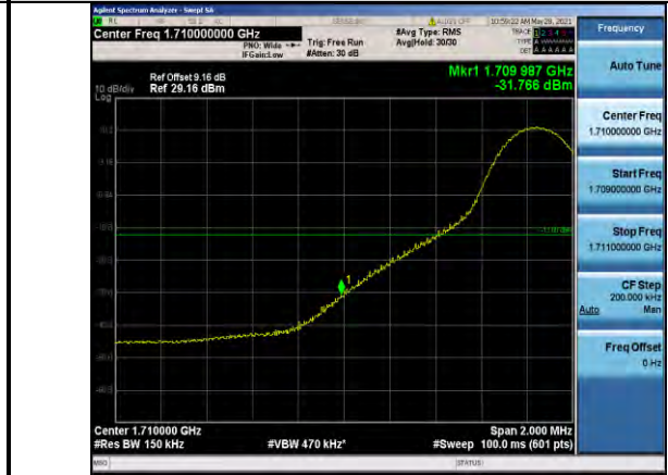
Band66-15MHz-16QAM-132047-1RB#0
