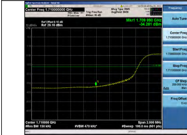
Band66-15MHz-QPSK-132047-75RB#0
