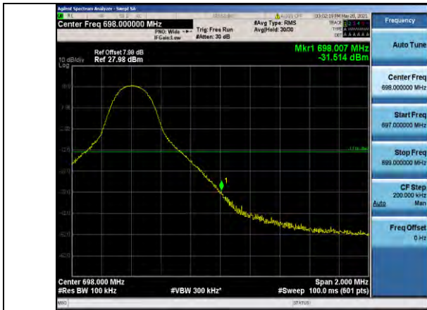
Band71-10MHz-16QAM-133422-1RB#49
