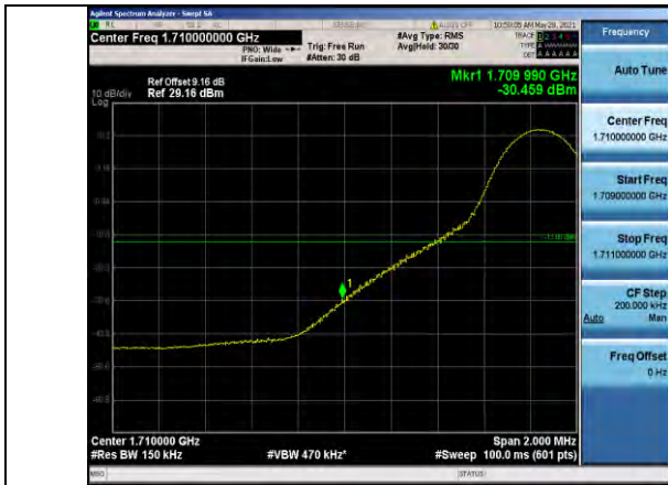
Band66-15MHz-QPSK-132047-1RB#0
