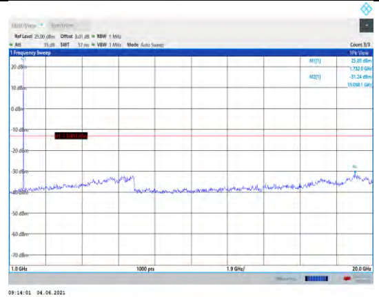
Band4-10MHz-16QAM-20175-1RB#0- Range2:1000~20000MHz
