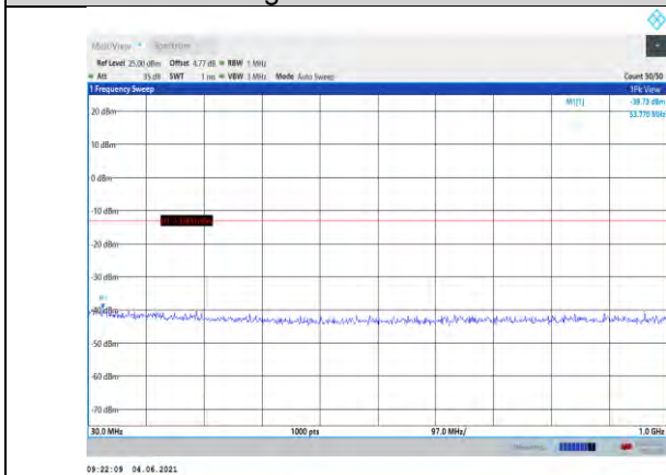
Band4-20MHz-QPSK-20175-1RB#0- Range1:30~1000MHz
