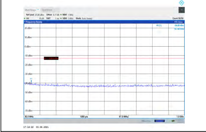
Band2-10MHz-QPSK-18900-1RB#0- Range1:30~1000MHz
