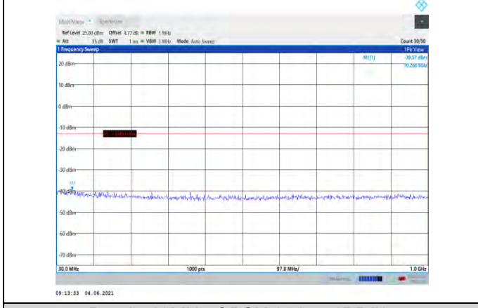
Band4-10MHz-QPSK-20175-1RB#0- Range1:30~1000MHz
