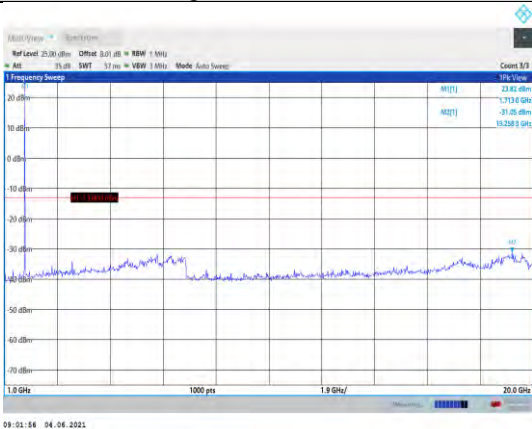
Band4-1.4MHz-16QAM-19957-1RB#0- Range2:1000~20000MHz
