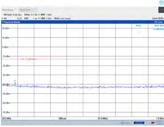
Band25-20MHz-16QAM-26140-1RB#0- Range1:30~1000MHz
