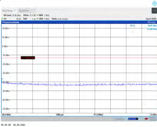
Band25-5MHz-QPSK-26065-1RB#0- Range1:30~1000MHz
