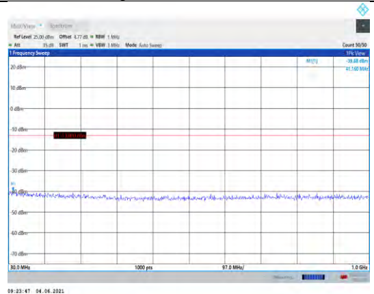
Band4-20MHz-16QAM-20300-1RB#0- Range1:30~1000MHz
