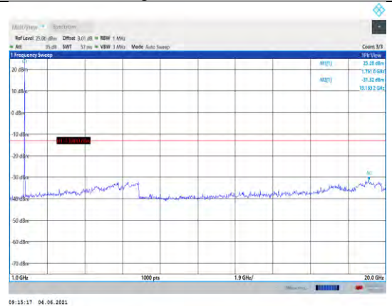
Band4-10MHz-16QAM-20350-1RB#0- Range2:1000~20000MHz
