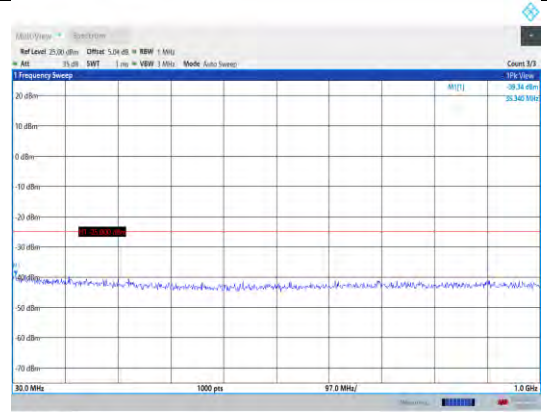
Band41-5MHz-16QAM-39675-1RB#0- Range1:30~1000MHz
