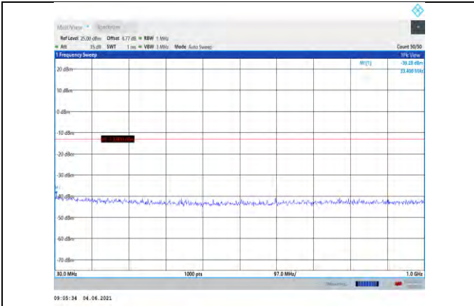
Band4-3MHz-16QAM-19965-1RB#0- Range1:30~1000MHz
