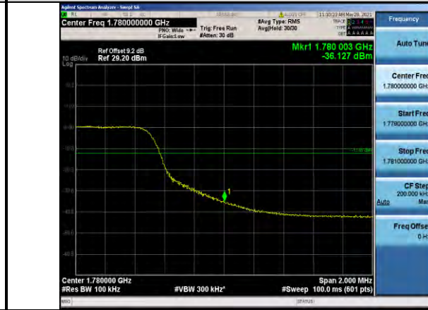
Band66-10MHz-16QAM-132622-50RB#0
