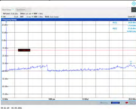
Band4-20MHz-16QAM-20050-1RB#0- Range2:1000~20000MHz
