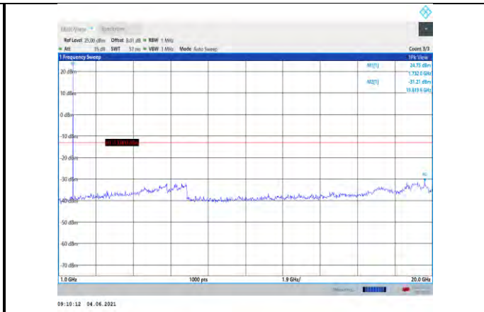
Band4-5MHz-16QAM-20175-1RB#0- Range2:1000~20000MHz
