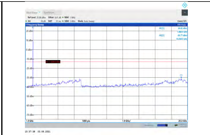
Band2-5MHz-16QAM-18900-1RB#0- Range2:1000~20000MHz
