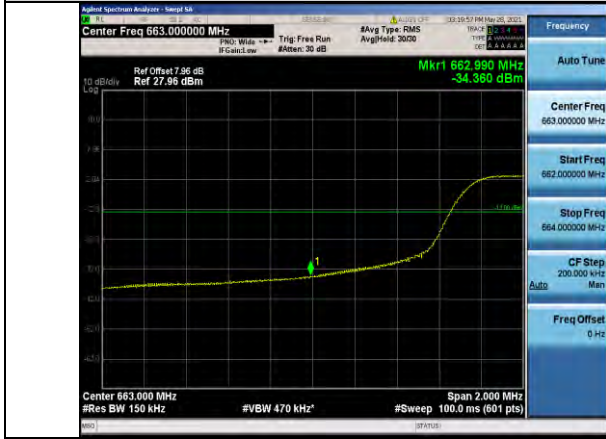
Band71-15MHz-16QAM-133197-75RB#0
