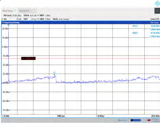
Band25-3MHz-16QAM-26055-1RB#0- Range2:1000~20000MHz
