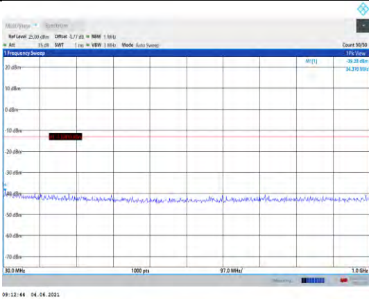
Band4-10MHz-16QAM-20000-1RB#0- Range1:30~1000MHz
