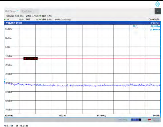
Band4-10MHz-16QAM-20350-1RB#0- Range1:30~1000MHz
