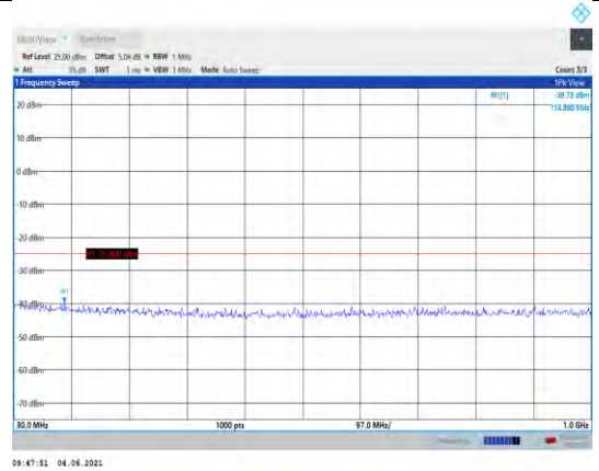
Band41-5MHz-QPSK-40620-1RB#0- Range1:30~1000MHz
