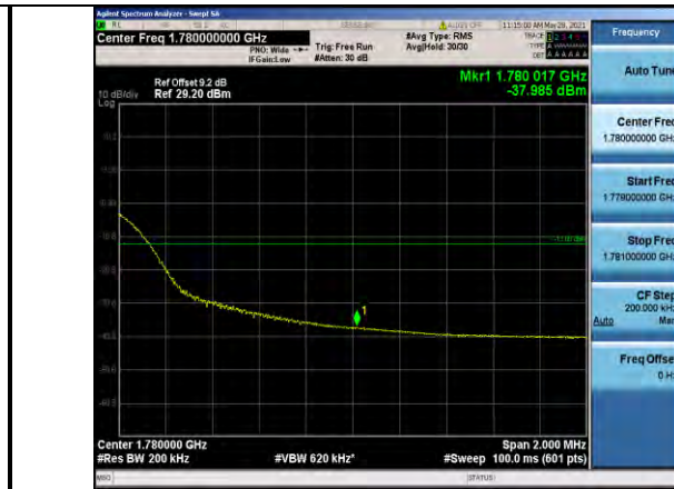
Band66-20MHz-16QAM-132572-100RB#0
