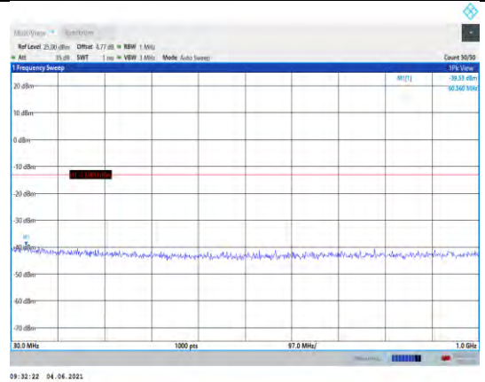
Band25-5MHz-16QAM-26365-1RB#0- Range1:30~1000MHz
