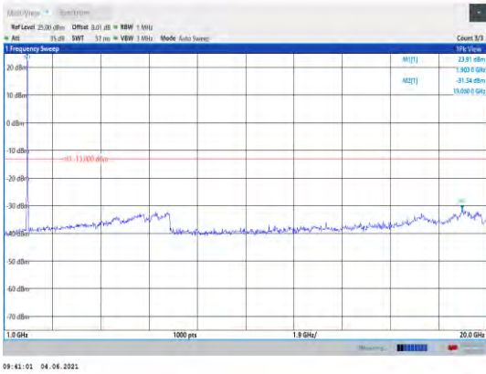
Band25-15MHz-16QAM-26615-1RB#0- Range2:1000~20000MHz
