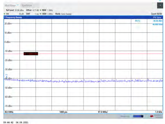
Band25-20MHz-QPSK-26590-1RB#0- Range1:30~1000MHz
