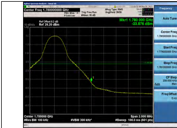
Band66-10MHz-QPSK-132622-1RB#49
