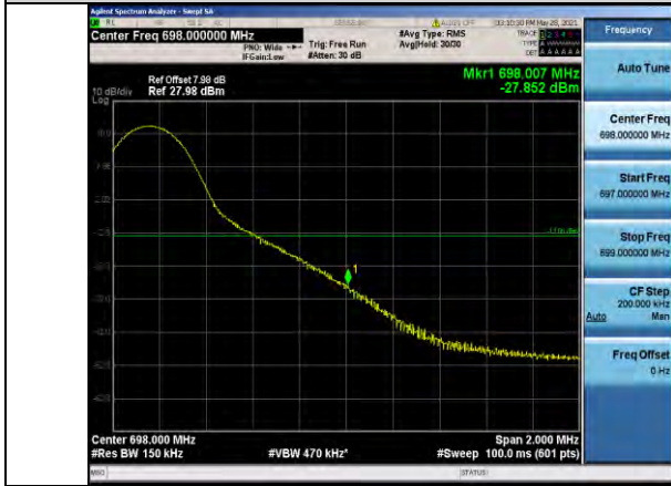
Band71-15MHz-16QAM-133397-1RB#74
