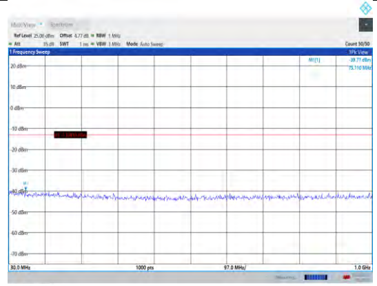
Band25-3MHz-16QAM-26675-1RB#0- Range1:30~1000MHz
