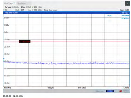
Band25-15MHz-QPSK-26365-1RB#0- Range1:30~1000MHz
