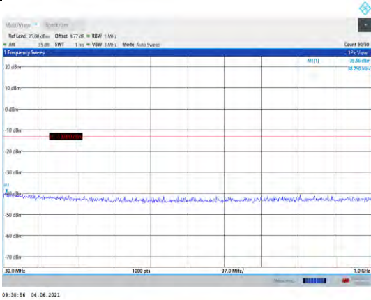
Band25-5MHz-16QAM-26065-1RB#0- Range1:30~1000MHz
