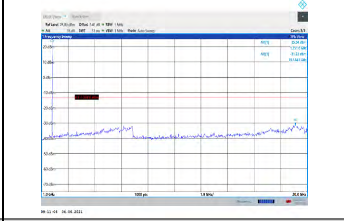
Band4-5MHz-16QAM-20375-1RB#0- Range2:1000~20000MHz
