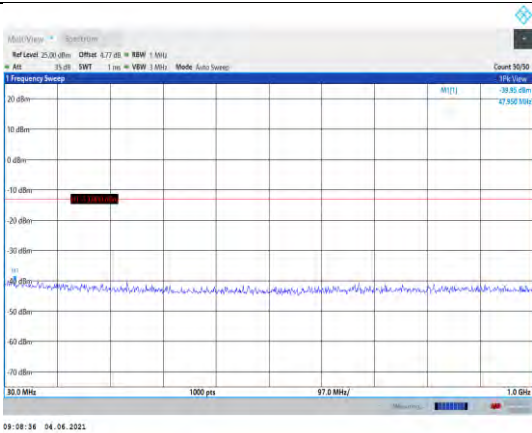
Band4-5MHz-QPSK-19975-1RB#0- Range1:30~1000MHz
