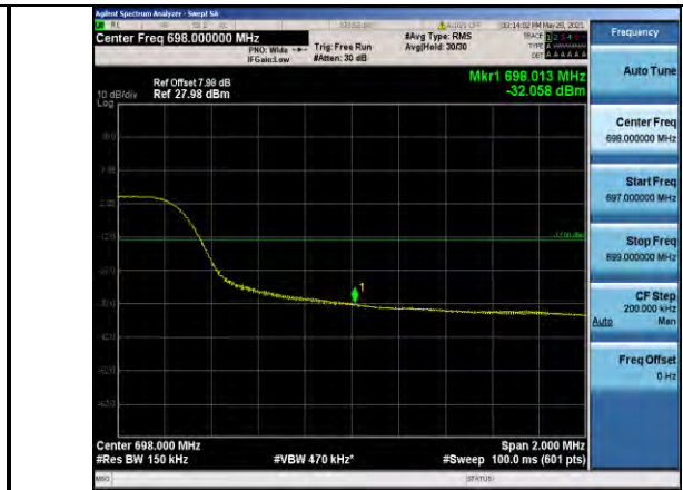
Band71-15MHz-16QAM-133397-75RB#0
