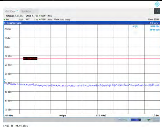
Band2-15MHz-QPSK-19125-1RB#0- Range1:30~1000MHz
