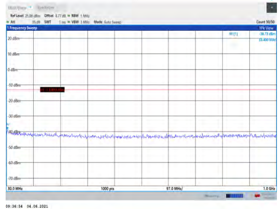
Band25-10MHz-QPSK-26640-1RB#0- Range1:30~1000MHz
