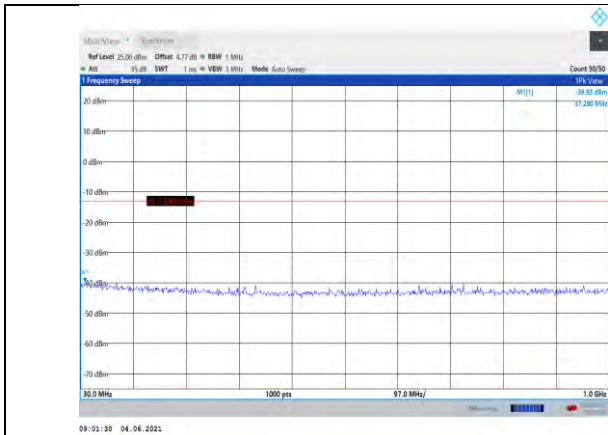
Band4-1.4MHz-QPSK-19957-1RB#0- Range1:30~1000MHz
