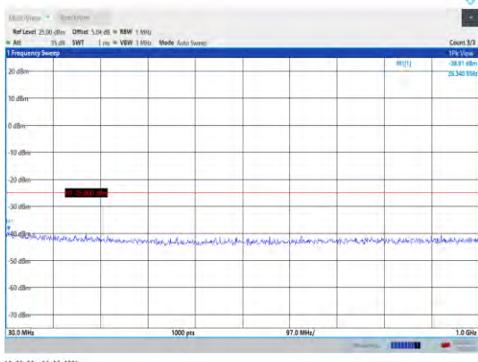
Band41-10MHz-QPSK-41540-1RB#0- Range1:30~1000MHz
