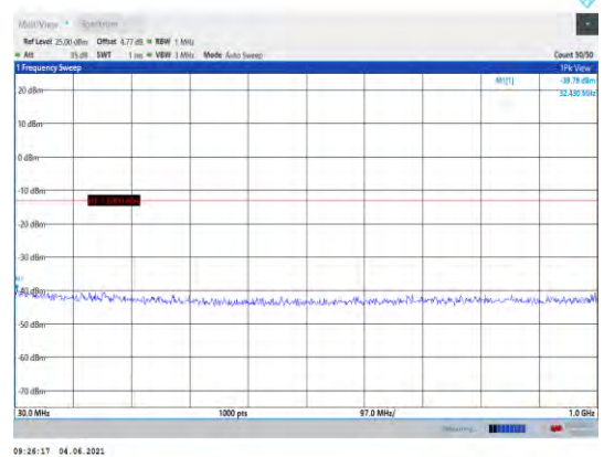
Band25-1.4MHz-16QAM-26683-1RB#0- Range1:30~1000MHz
