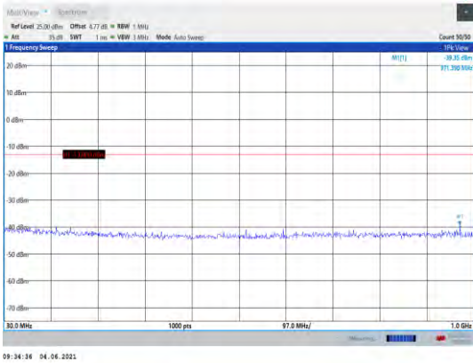
Band25-10MHz-QPSK-26090-1RB#0- Range1:30~1000MHz
