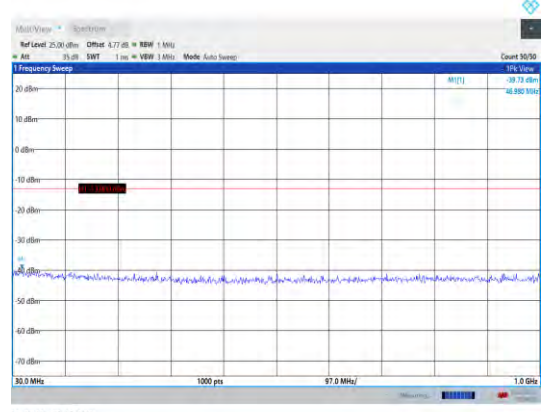
Band25-20MHz-16QAM-26590-1RB#0- Range1:30~1000MHz
