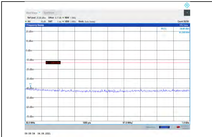
Band4-5MHz-16QAM-19975-1RB#0- Range1:30~1000MHz
