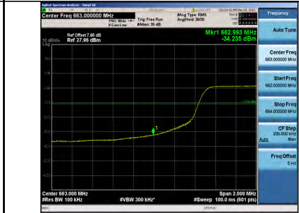
Band71-10MHz-16QAM-133172-50RB#0
