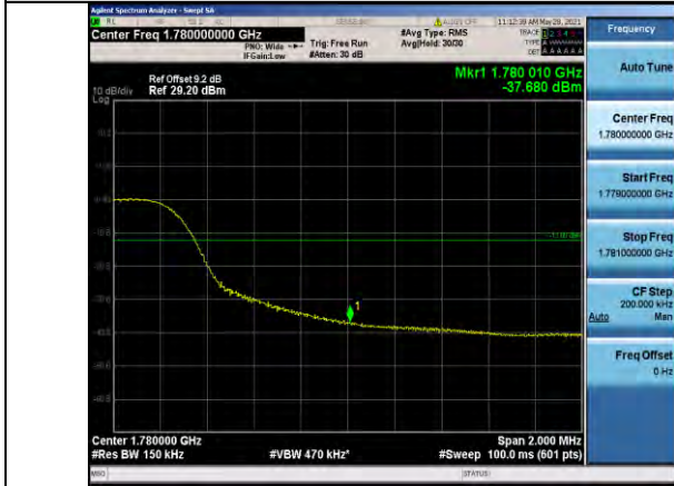
Band66-15MHz-16QAM-132597-75RB#0
