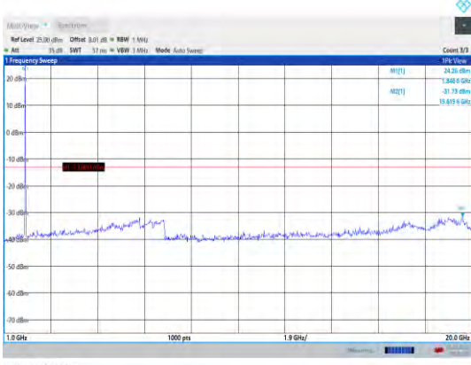
Band25-20MHz-16QAM-26140-1RB#0- Range2:1000~20000MHz
