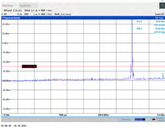
Band41-5MHz-16QAM-40620-1RB#0- Range2:1000~3000MHz
