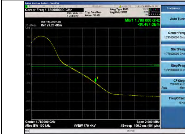
Band66-15MHz-QPSK-132597-1RB#74
