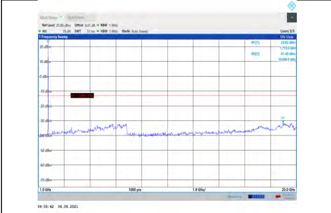
Band4-3MHz-16QAM-19965-1RB#0- Range2:1000~20000MHz
