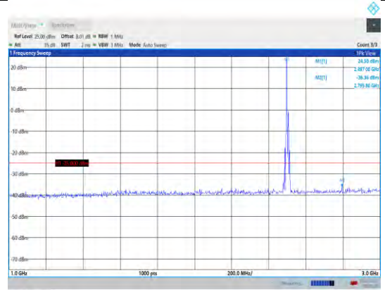
Band41-5MHz-16QAM-39675-1RB#0- Range2:1000~3000MHz
