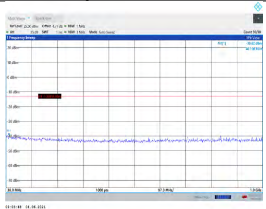
Band4-1.4MHz-16QAM-20393-1RB#0- Range1:30~1000MHz
