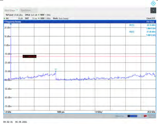
Band25-5MHz-16QAM-26365-1RB#0- Range2:1000~20000MHz
