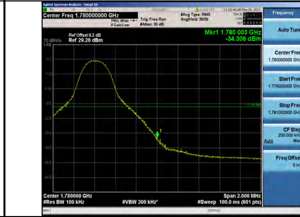
Band66-10MHz-16QAM-132622-1RB#49
