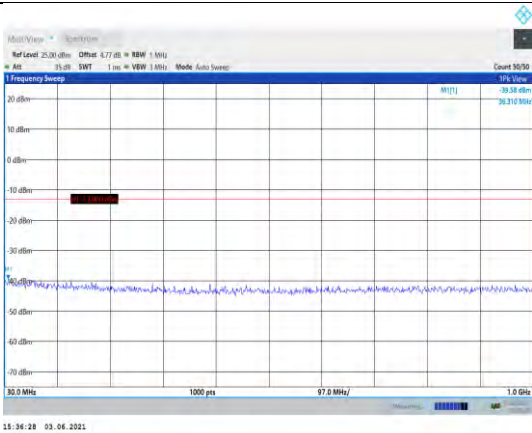
Band2-5MHz-QPSK-18625-1RB#0- Range1:30~1000MHz
