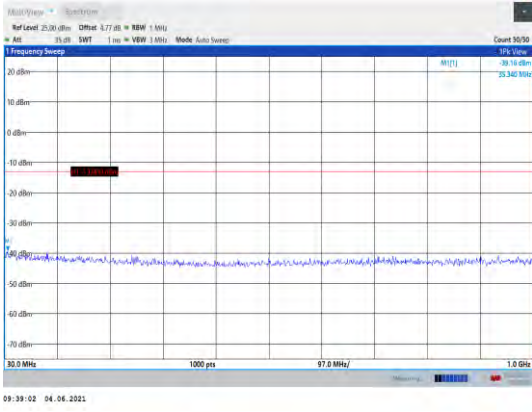
Band25-15MHz-16QAM-26115-1RB#0- Range1:30~1000MHz
