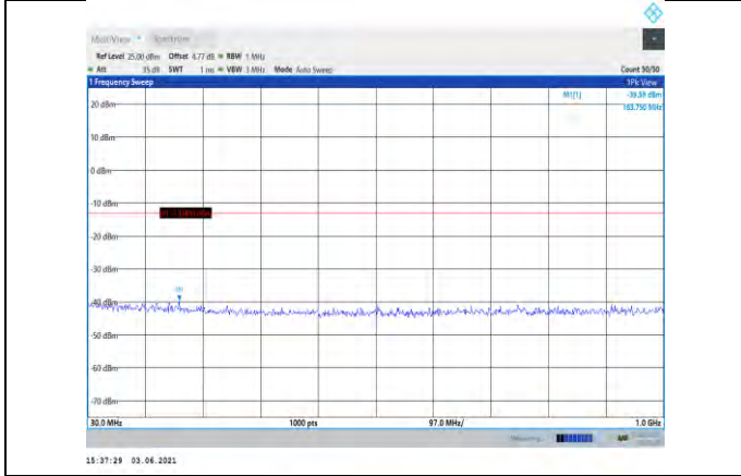
Band2-5MHz-16QAM-18900-1RB#0- Range1:30~1000MHz
