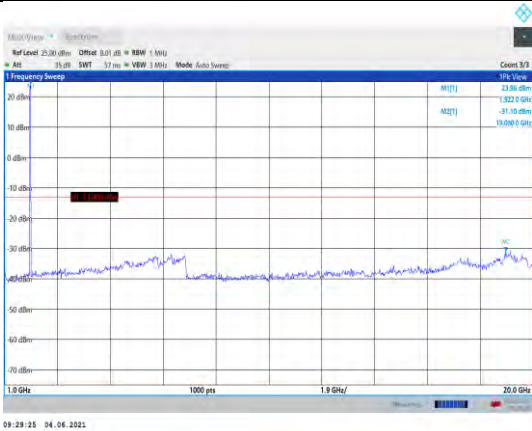
Band25-3MHz-16QAM-26675-1RB#0- Range2:1000~20000MHz
