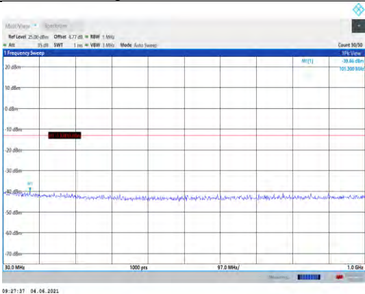
Band25-3MHz-QPSK-26055-1RB#0- Range1:30~1000MHz
