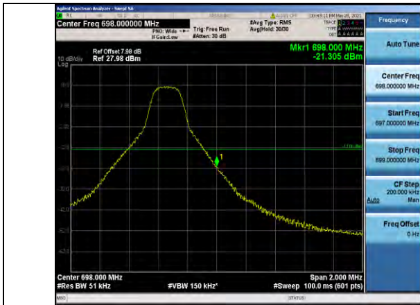
Band71-5MHz-QPSK-133447-1RB#24
