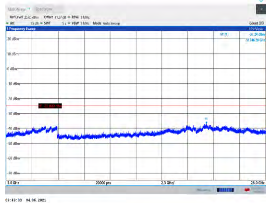
Band41-5MHz-16QAM-40620-1RB#0- Range3:3000~26000MHz
