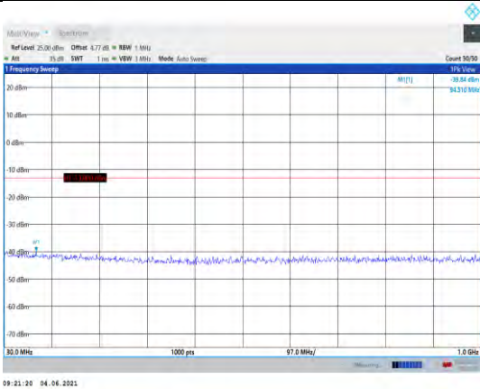
Band4-20MHz-16QAM-20050-1RB#0- Range1:30~1000MHz
