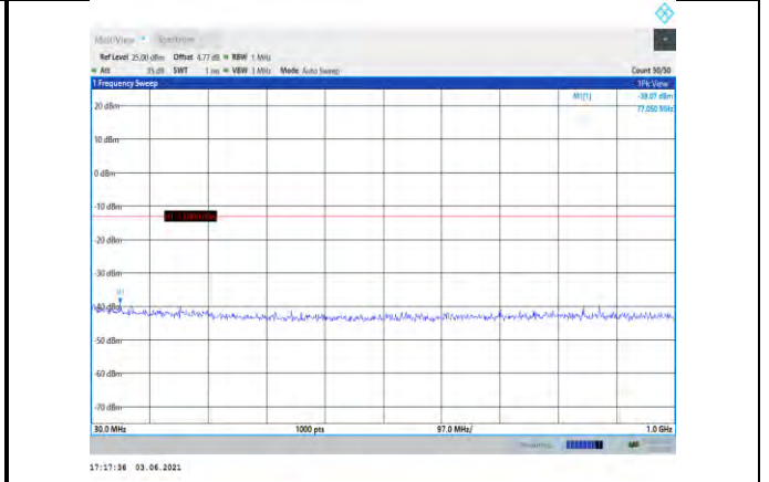
Band2-10MHz-QPSK-19150-1RB#0- Range1:30~1000MHz
