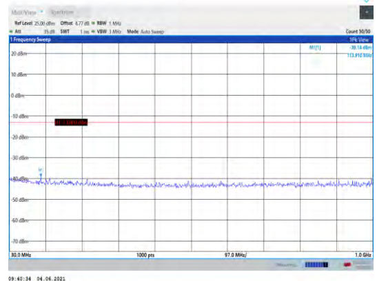
Band25-15MHz-QPSK-26615-1RB#0- Range1:30~1000MHz
