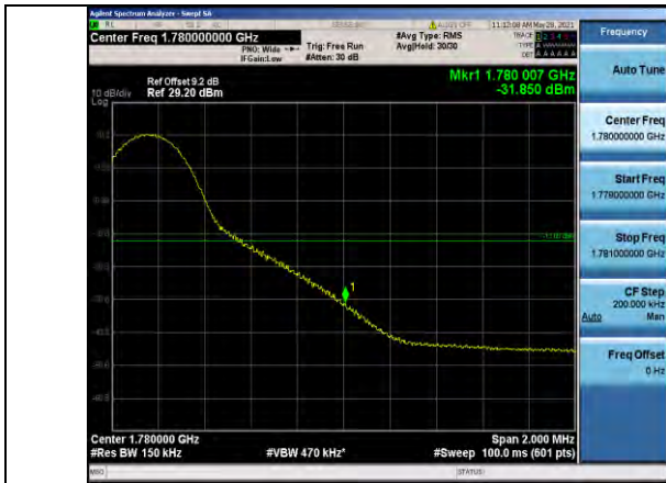
Band66-15MHz-16QAM-132597-1RB#74
