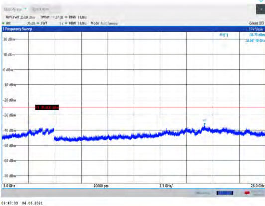
Band41-5MHz-16QAM-39675-1RB#0- Range3:3000~26000MHz
