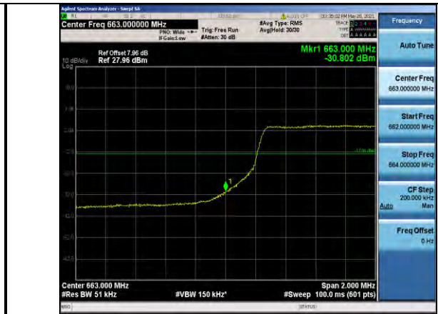
Band71-5MHz-16QAM-133147-25RB#0
