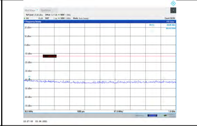
Band2-3MHz-16QAM-19185-1RB#0- Range1:30~1000MHz
