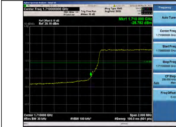
Band66-3MHz-QPSK-131987-15RB#0
