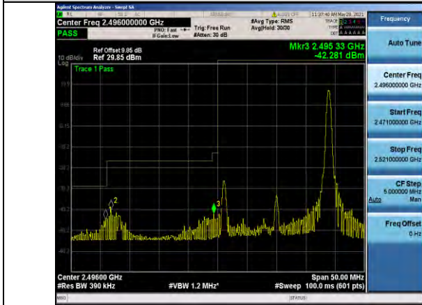
Band41-20MHz-QPSK-39750-1RB#99
