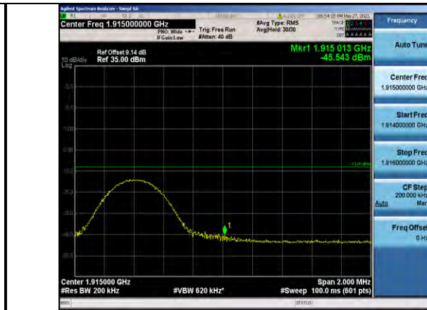
Band25-10MHz-16QAM-26640-1RB#0
