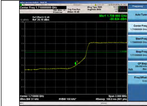
Band66-5MHz-16QAM-131997-25RB#0
