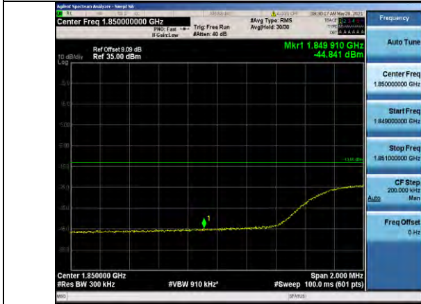
Band25-15MHz-QPSK-26115-1RB#74
