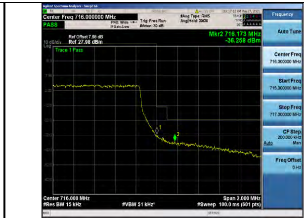
Band12-1.4MHz-16QAM-23173-6RB#0
