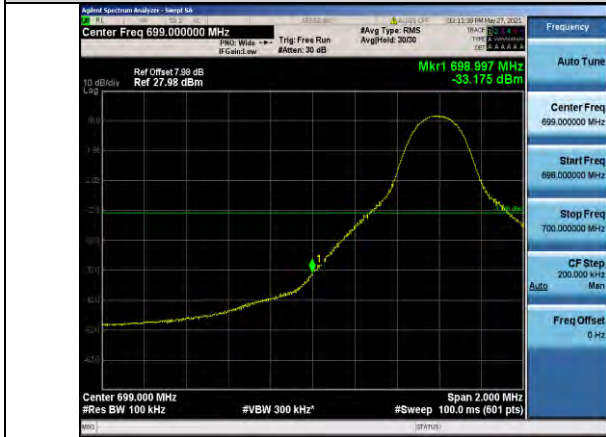
Band12-10MHz-QPSK-23060-1RB#0
