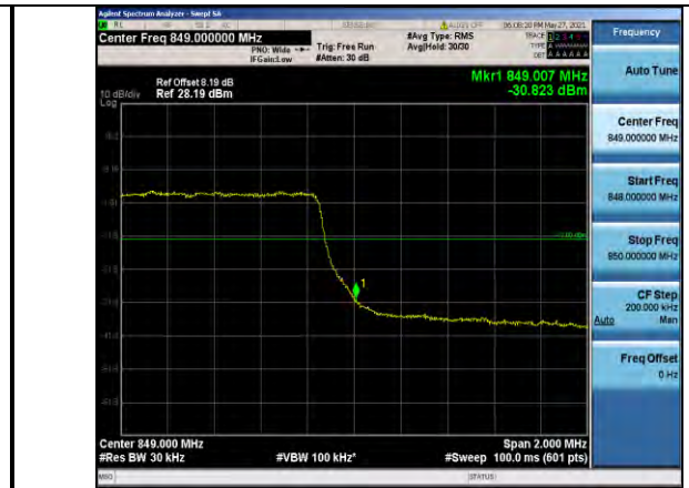
Band5-3MHz-16QAM-20635-15RB#0
