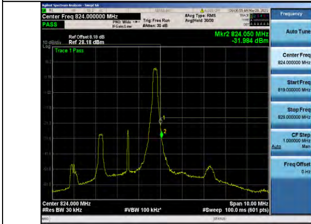
Band26-3MHz-16QAM-26775-1RB#14
