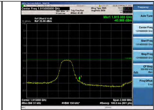
Band25-3MHz-QPSK-26675-1RB#0
