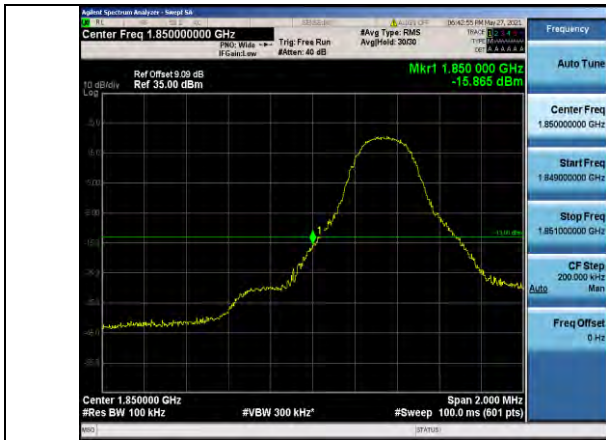
Band25-5MHz-QPSK-26065-1RB#0
