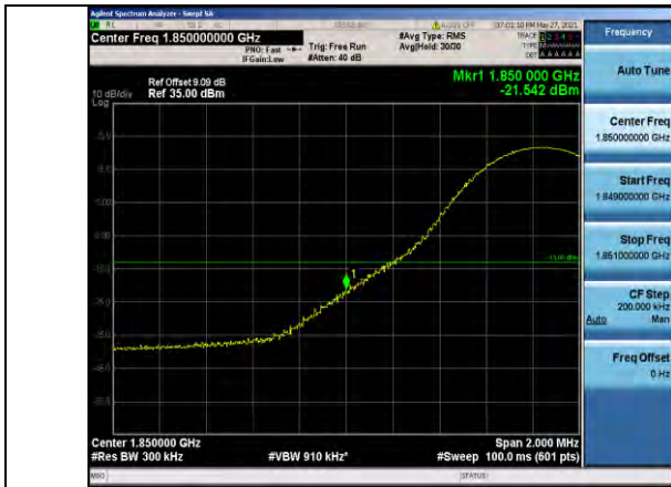
Band25-15MHz-QPSK-26115-1RB#0
