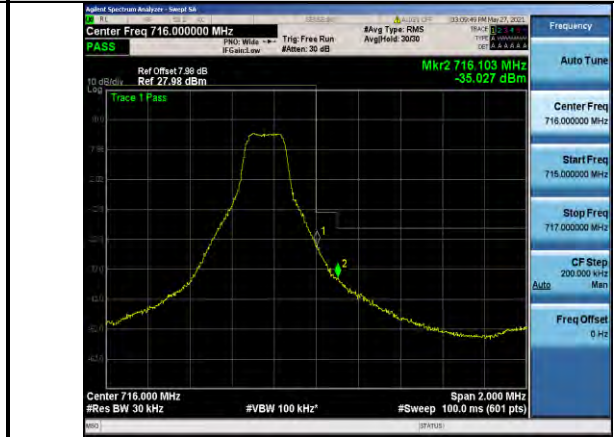
Band12-3MHz-16QAM-23165-1RB#14
