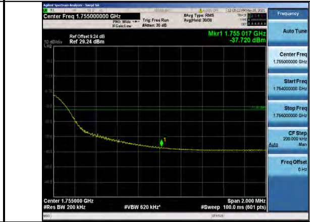
Band4-20MHz-16QAM-20300-100RB#0
