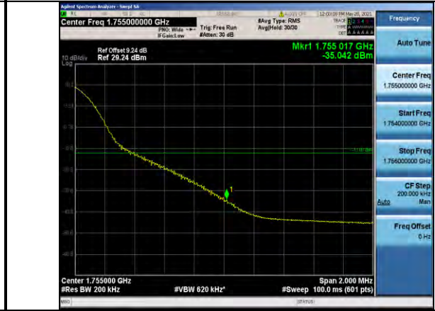
Band4-20MHz-16QAM-20300-1RB#99
