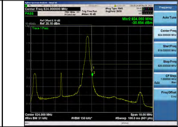
Band26-5MHz-16QAM-26765-1RB#24
