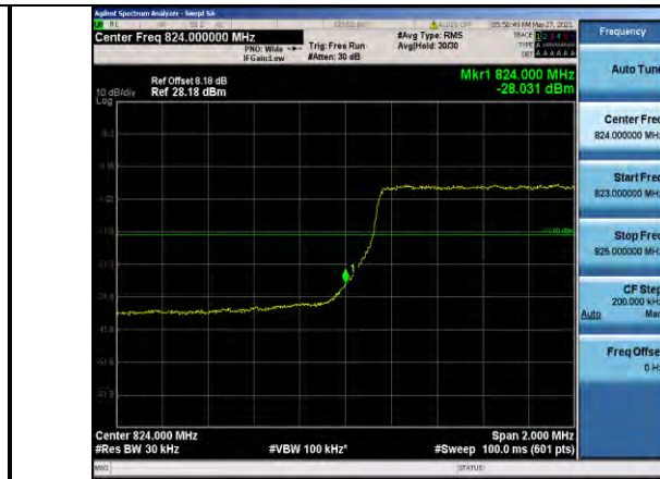
Band5-3MHz-QPSK-20415-15RB#0
