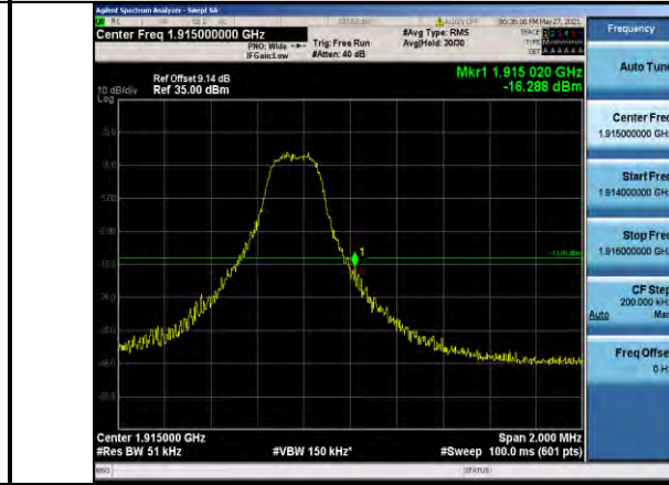
Band25-3MHz-16QAM-26675-1RB#14
