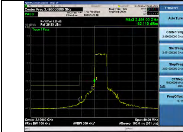
Band41-5MHz-16QAM-39675-25RB#0
