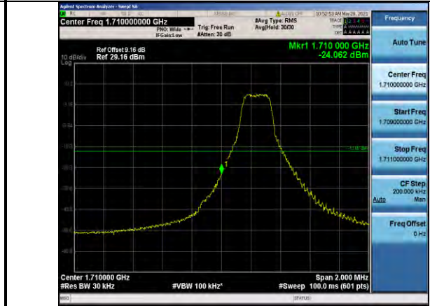
Band66-3MHz-16QAM-131987-1RB#0
