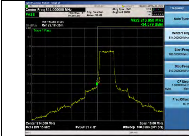
Band26-1.4MHz-QPSK-26697-6RB#0
