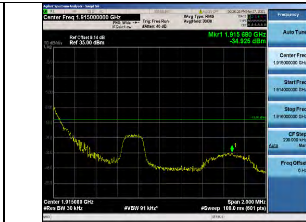
Band25-1.4MHz-QPSK-26683-1RB#0
