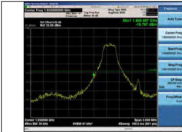
Band25-1.4MHz-16QAM-26047-1RB#0
