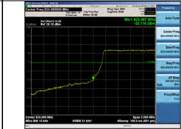
Band5-1.4MHz-16QAM-20407-6RB#0
