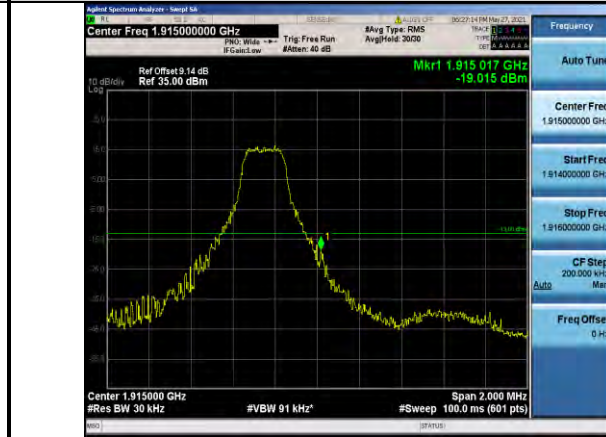
Band25-1.4MHz-16QAM-26683-1RB#5
