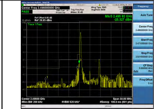
Band41-10MHz-QPSK-39700-1RB#0
