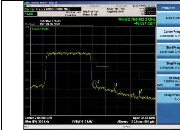
Band41-15MHz-16QAM-41515-75RB#0
