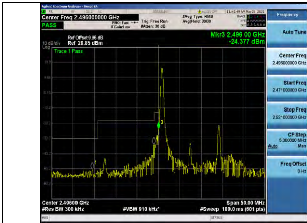
Band41-15MHz-QPSK-39725-1RB#0
