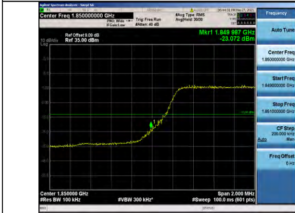
Band25-5MHz-QPSK-26065-25RB#0
