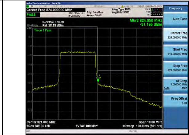
Band26-3MHz-QPSK-26775-15RB#0
