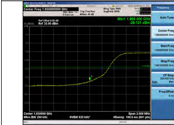
Band25-10MHz-16QAM-26090-50RB#0
