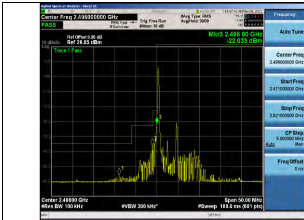
Band41-5MHz-16QAM-39675-1RB#0
