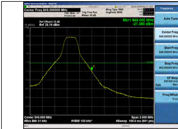
Band5-5MHz-QPSK-20625-1RB#24
