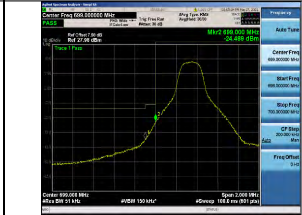
Band12-5MHz-16QAM-23035-1RB#0
