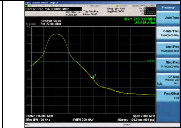
Band12-10MHz-QPSK-23130-1RB#49
