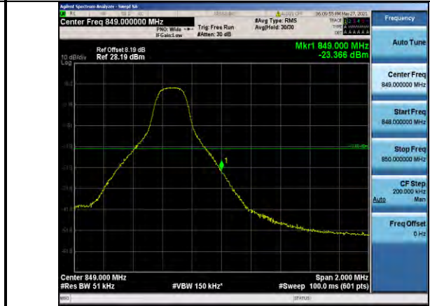
Band5-5MHz-16QAM-20625-1RB#24
