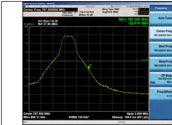
Band13-5MHz-QPSK-23255-1RB#24
