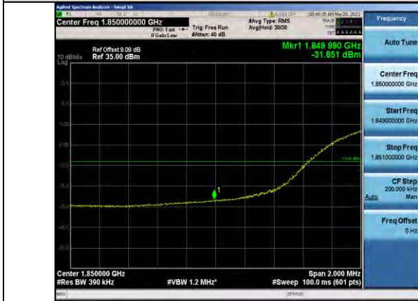
Band25-20MHz-QPSK-26140-100RB#0
