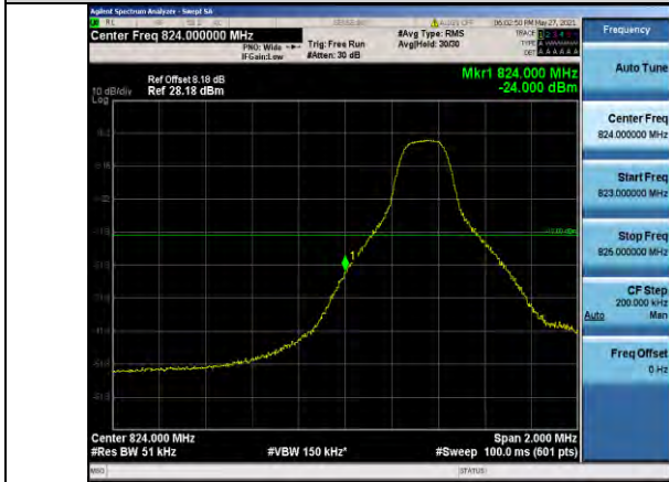
Band5-5MHz-16QAM-20425-1RB#0
