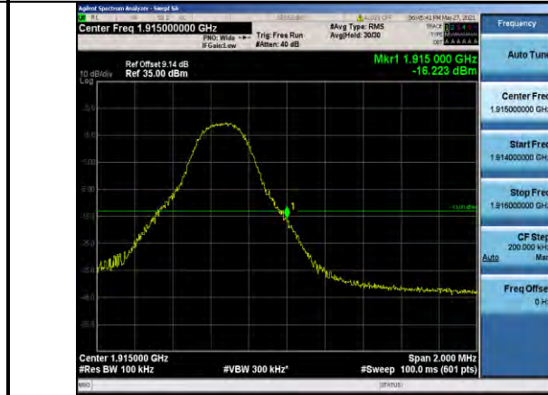
Band25-5MHz-16QAM-26665-1RB#24
