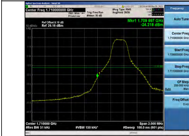
Band66-5MHz-QPSK-131997-1RB#0
