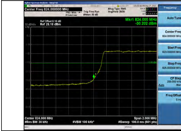
Band5-3MHz-16QAM-20415-15RB#0
