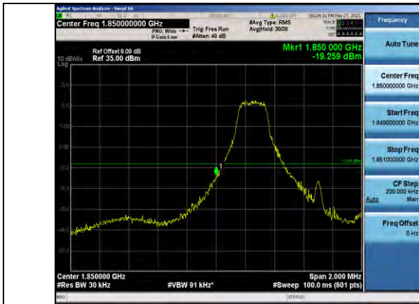
Band25-1.4MHz-QPSK-26047-1RB#0
