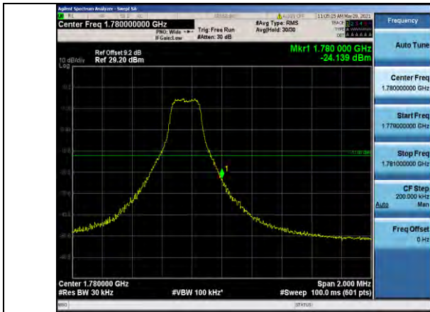
Band66-3MHz-16QAM-132657-1RB#14
