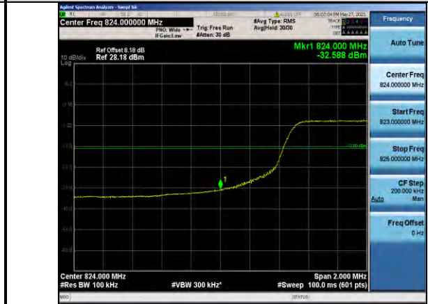
Band5-10MHz-16QAM-20450-50RB#0
