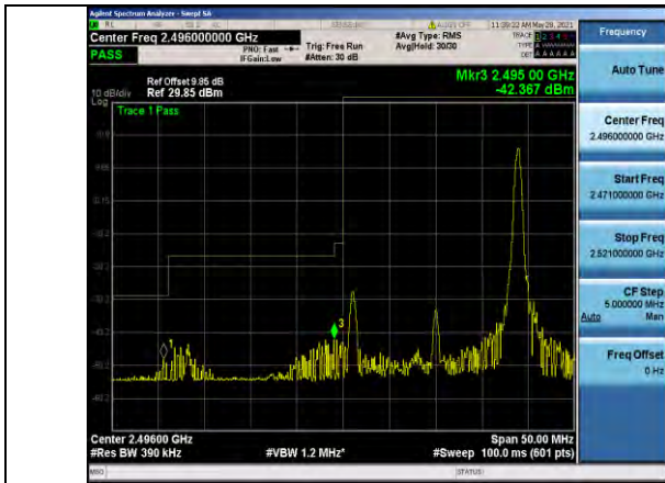
Band41-20MHz-16QAM-39750-1RB#99
