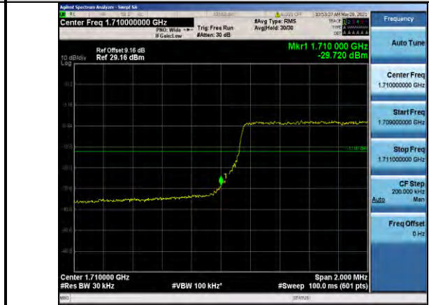
Band66-3MHz-16QAM-131987-15RB#0
