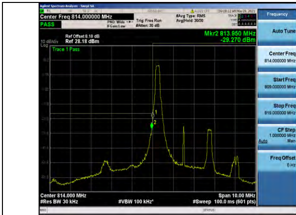
Band26-3MHz-16QAM-26705-1RB#0
