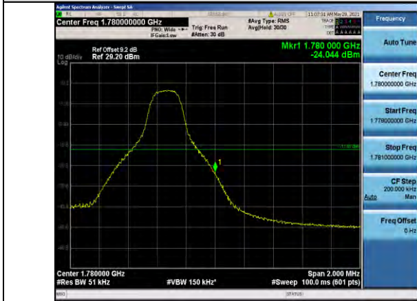
Band66-5MHz-16QAM-132647-1RB#24
