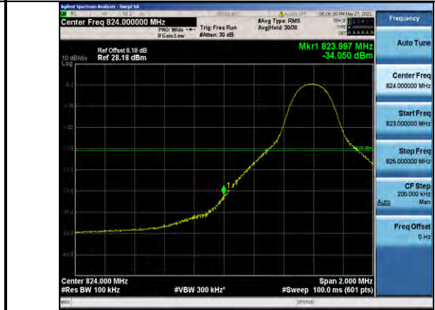
Band5-10MHz-16QAM-20450-1RB#0
