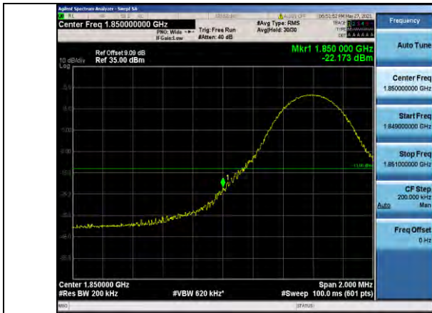
Band25-10MHz-QPSK-26090-1RB#0
