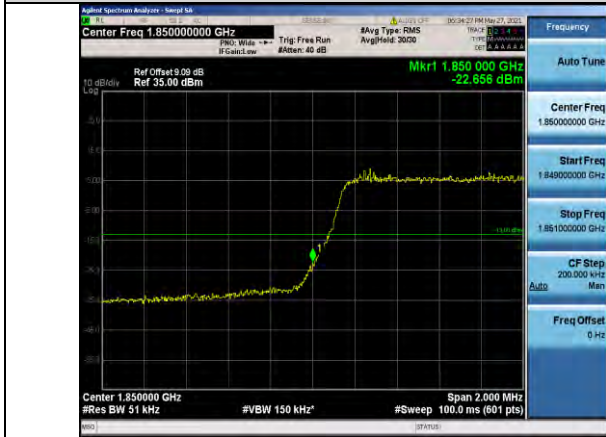
Band25-3MHz-QPSK-26055-15RB#0
