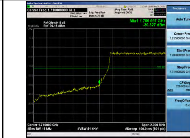
Band66-1.4MHz-QPSK-131979-6RB#0
