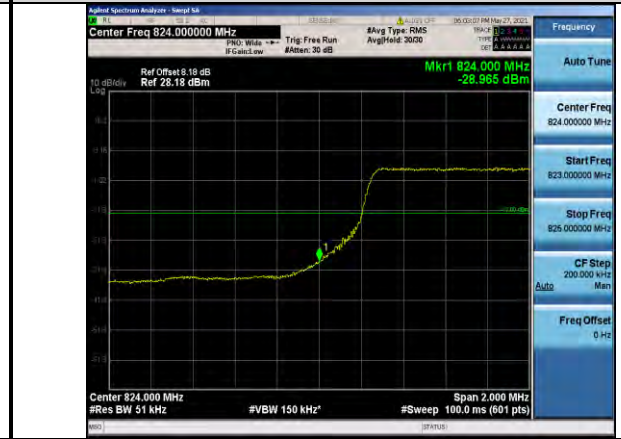
Band5-5MHz-QPSK-20425-25RB#0
