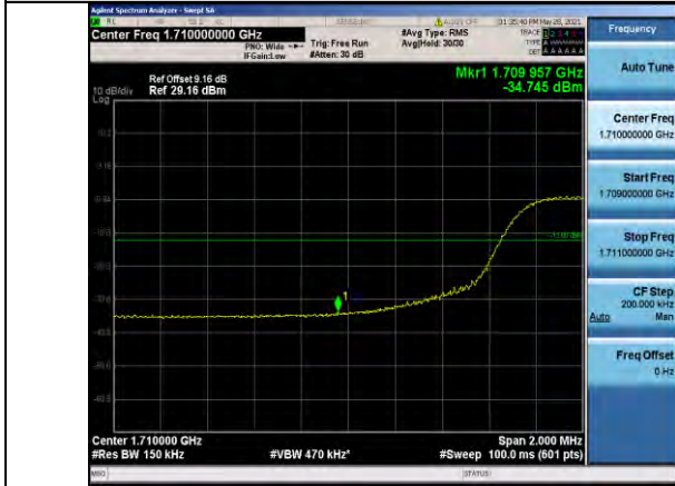
Band4-15MHz-16QAM-20025-75RB#0
