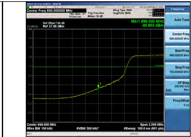
Band12-10MHz-QPSK-23060-50RB#0
