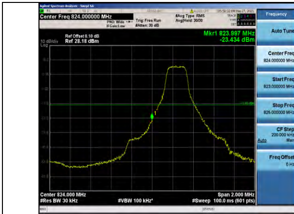
Band5-3MHz-16QAM-20415-1RB#0
