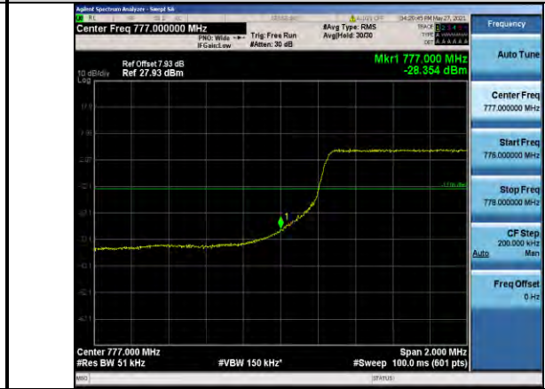
Band13-5MHz-QPSK-23205-25RB#0
