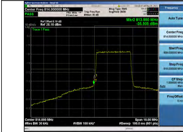
Band26-3MHz-16QAM-26705-15RB#0
