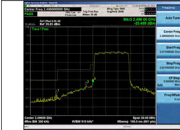
Band41-15MHz-QPSK-39725-75RB#0
