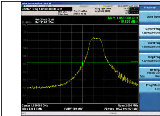
Band25-3MHz-16QAM-26055-1RB#0
