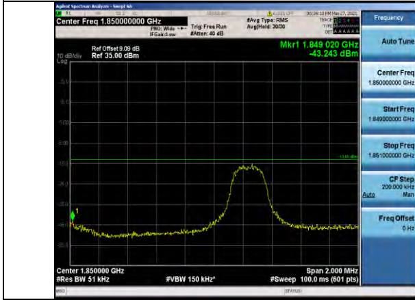
Band25-3MHz-16QAM-26055-1RB#14
