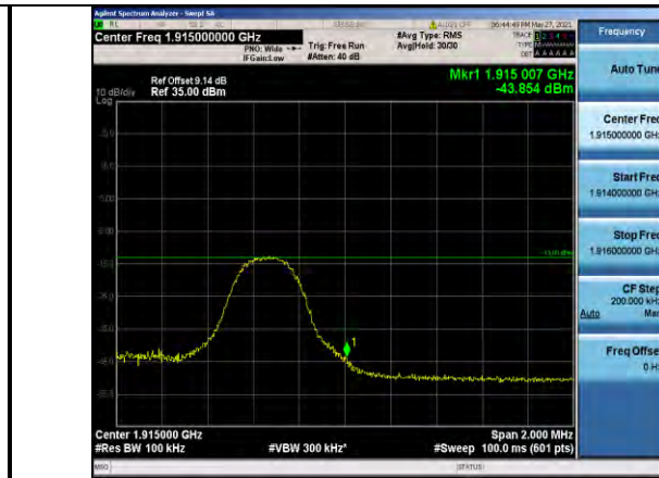
Band25-5MHz-QPSK-26665-1RB#0
