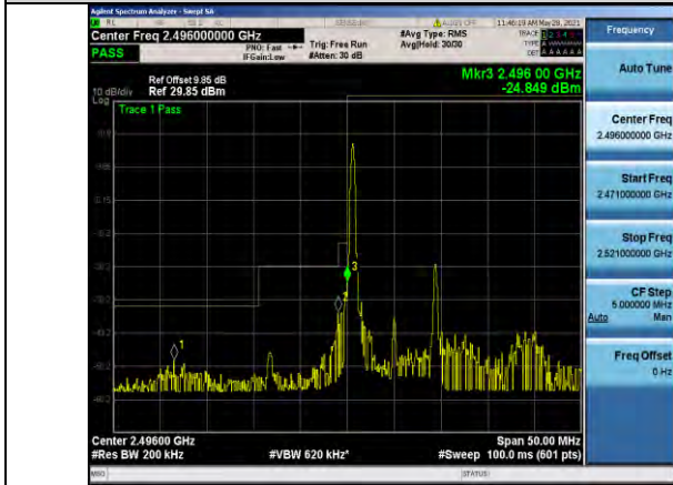
Band41-10MHz-16QAM-39700-1RB#0
