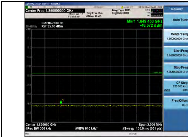
Band25-15MHz-16QAM-26115-1RB#0
