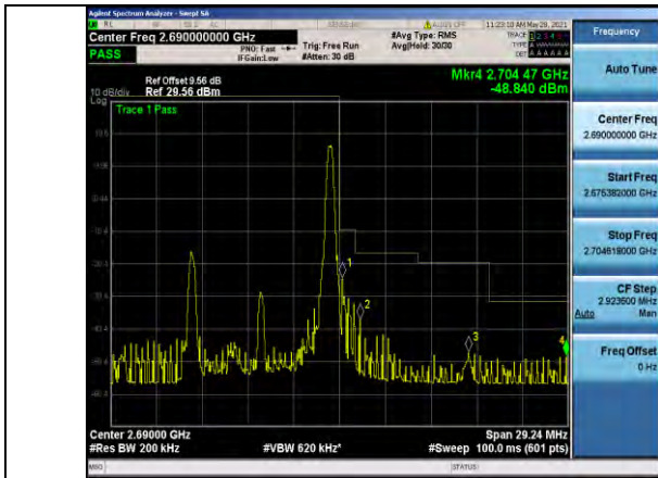
Band41-10MHz-QPSK-41540-1RB#49
