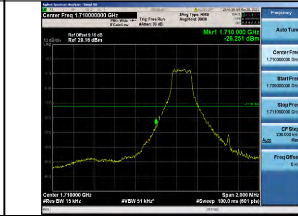
Band66-1.4MHz-QPSK-131979-1RB#0
