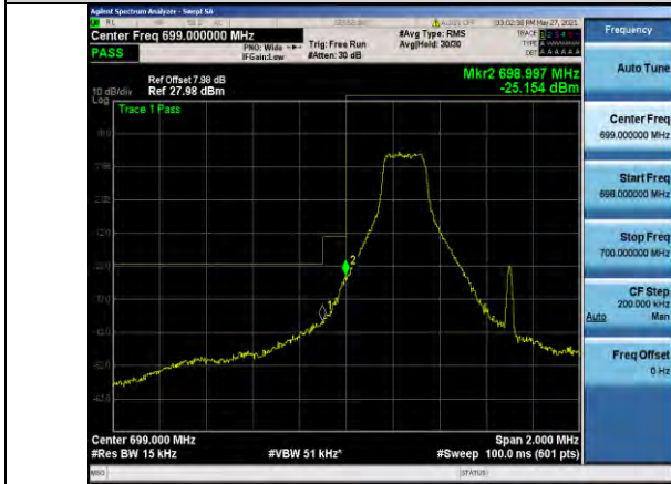
Band12-1.4MHz-QPSK-23017-1RB#0
