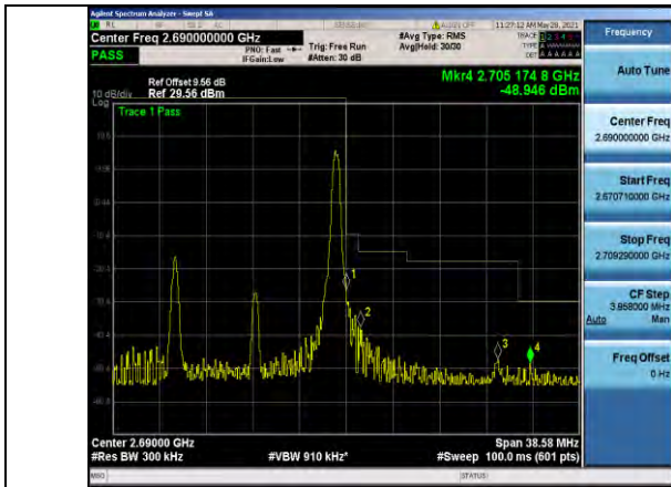
Band41-15MHz-16QAM-41515-1RB#74
