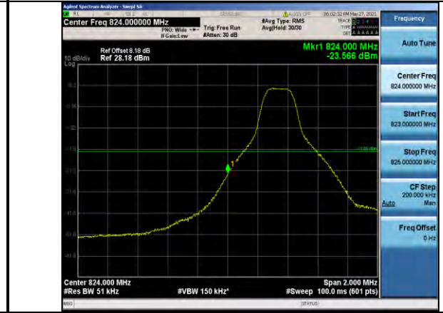
Band5-5MHz-QPSK-20425-1RB#0
