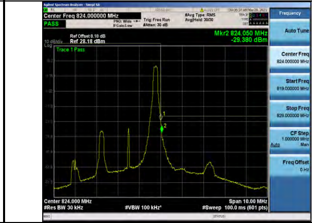
Band26-3MHz-QPSK-26775-1RB#14
