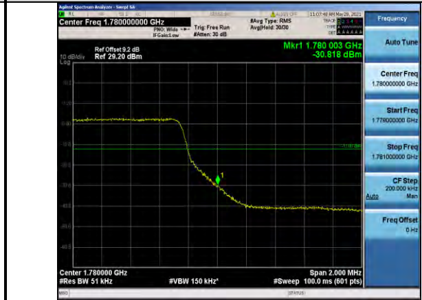
Band66-5MHz-QPSK-132647-25RB#0
