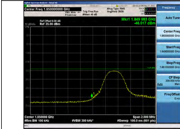
Band25-5MHz-QPSK-26065-1RB#24
