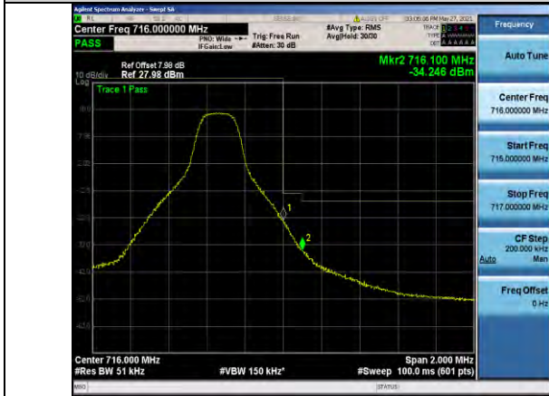
Band12-5MHz-QPSK-23155-1RB#24
