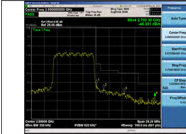
Band41-10MHz-QPSK-41540-50RB#0
