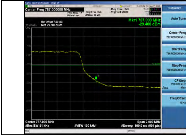
Band13-5MHz-QPSK-23255-25RB#0
