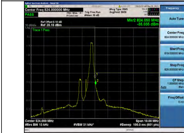
Band26-1.4MHz-QPSK-26783-1RB#5
