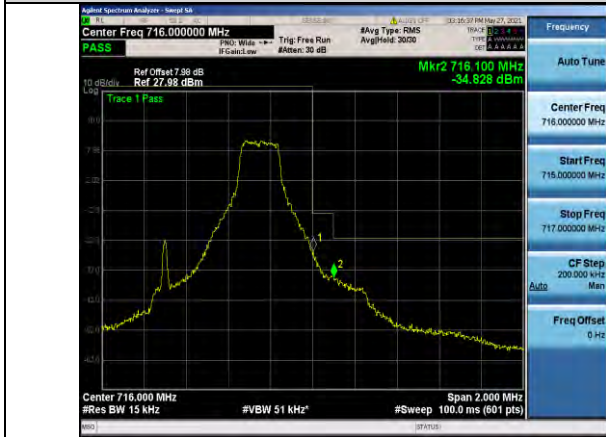
Band12-1.4MHz-16QAM-23173-1RB#5
