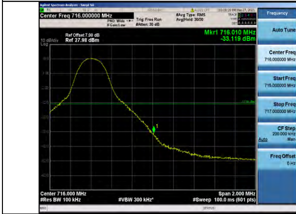
Band12-10MHz-16QAM-23130-1RB#49
