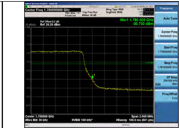
Band66-3MHz-QPSK-132657-15RB#0
