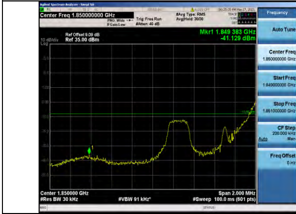
Band25-1.4MHz-QPSK-26047-1RB#5
