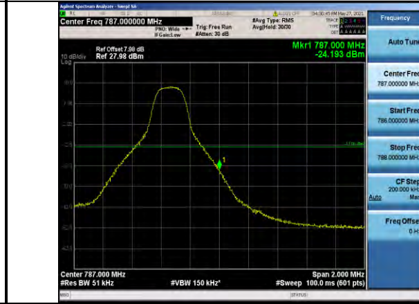
Band13-5MHz-16QAM-23255-1RB#24
