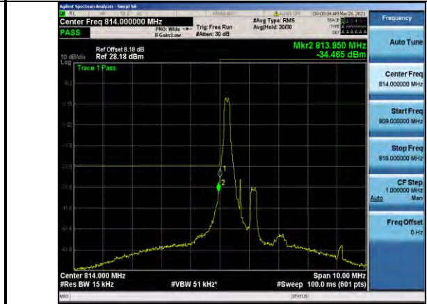
Band26-1.4MHz-16QAM-26697-1RB#0
