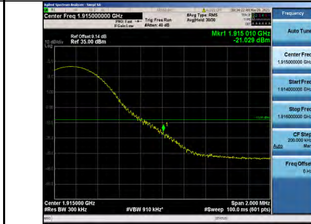
Band25-15MHz-QPSK-26615-1RB#74
