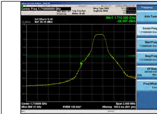
Band66-5MHz-16QAM-131997-1RB#0
