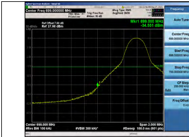
Band12-10MHz-16QAM-23060-1RB#0
