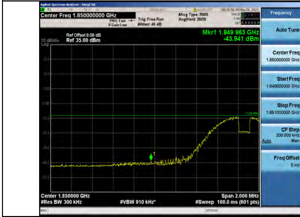
Band25-15MHz-16QAM-26115-1RB#74
