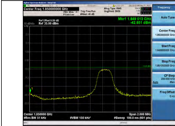
Band25-3MHz-QPSK-26055-1RB#14
