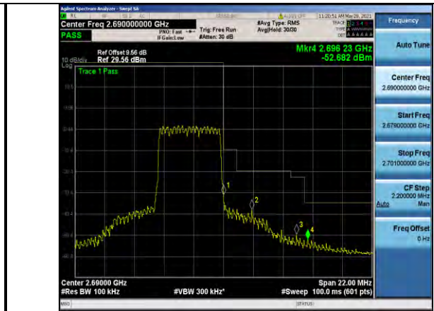
Band41-5MHz-16QAM-41565-25RB#0
