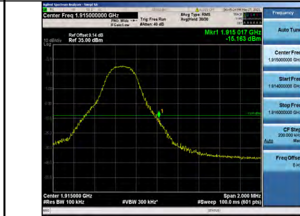
Band25-5MHz-QPSK-26665-1RB#24
