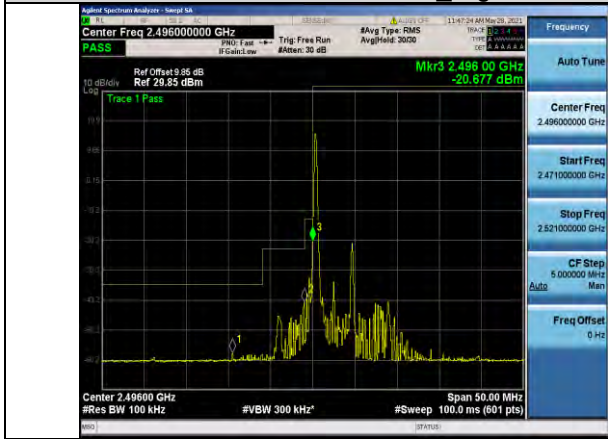
Band41-5MHz-QPSK-39675-1RB#0
