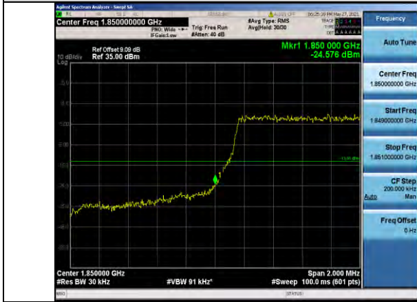
Band25-1.4MHz-QPSK-26047-6RB#0
