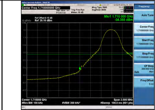
Band66-10MHz-QPSK-132022-1RB#0
