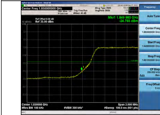
Band25-5MHz-16QAM-26065-25RB#0
