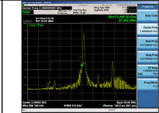
Band41-15MHz-16QAM-39725-1RB#0
