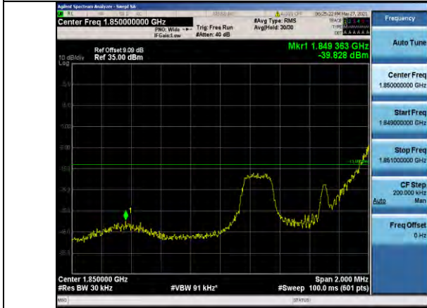
Band25-1.4MHz-16QAM-26047-1RB#5
