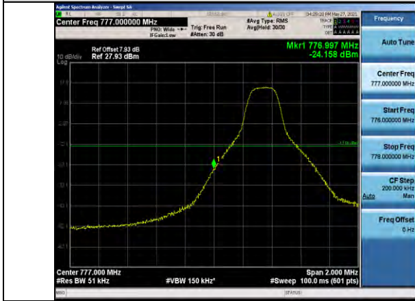
Band13-5MHz-16QAM-23205-1RB#0
