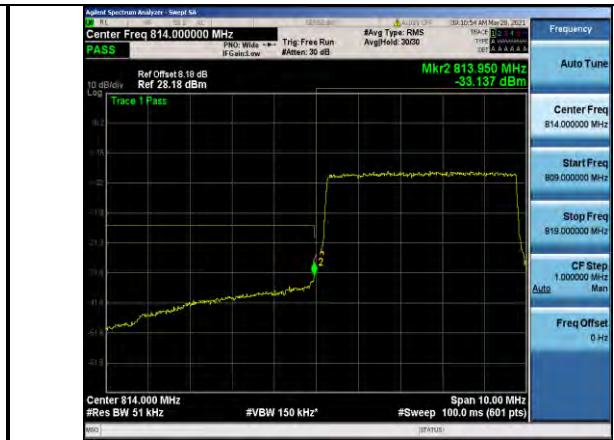
Band26-5MHz-16QAM-26715-25RB#0
