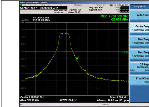
Band66-3MHz-QPSK-132657-1RB#14
