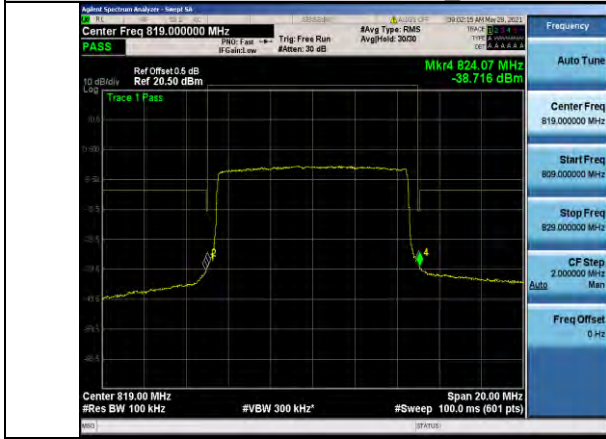
Band26-10MHz-QPSK-26740 Left-50RB#0
