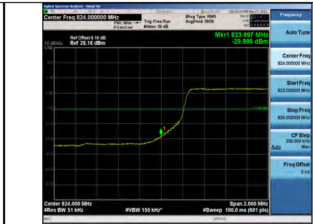
Band5-5MHz-16QAM-20425-25RB#0
