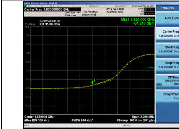
Band25-15MHz-16QAM-26115-75RB#0
