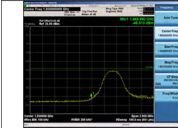
Band25-5MHz-16QAM-26065-1RB#24
