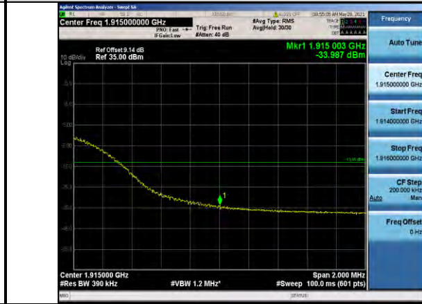
Band25-20MHz-16QAM-26590-100RB#0
