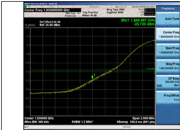
Band25-20MHz-16QAM-26140-1RB#0
