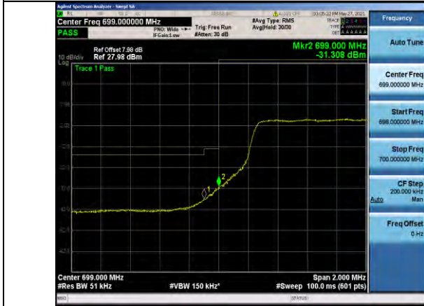
Band12-5MHz-QPSK-23035-25RB#0
