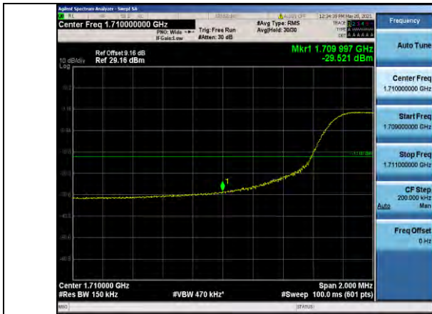
Band4-15MHz-16QAM-20025-1RB#0
