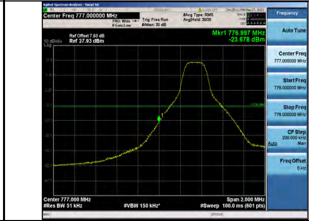
Band13-5MHz-QPSK-23205-1RB#0
