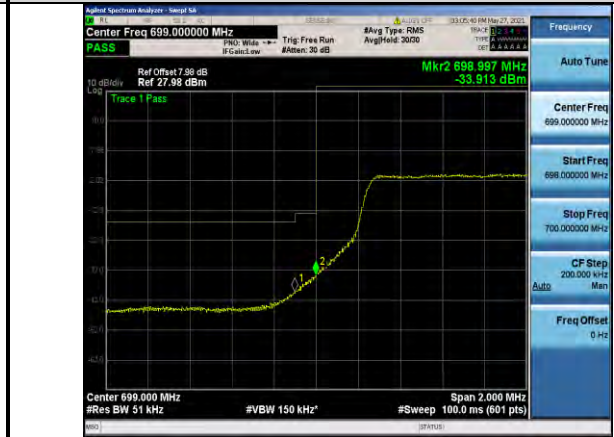
Band12-5MHz-16QAM-23035-25RB#0
