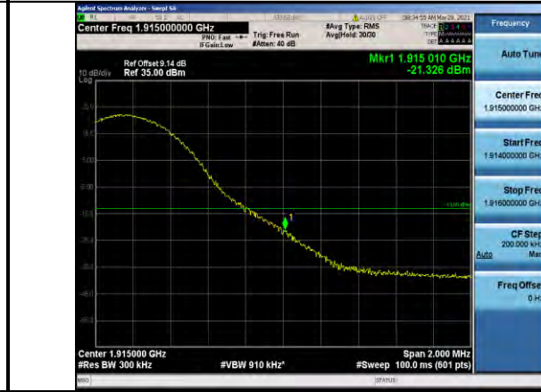
Band25-15MHz-16QAM-26615-1RB#74
