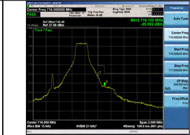
Band12-1.4MHz-QPSK-23173-1RB#5
