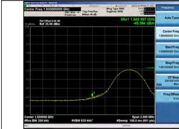
Band25-10MHz-QPSK-26090-1RB#49
