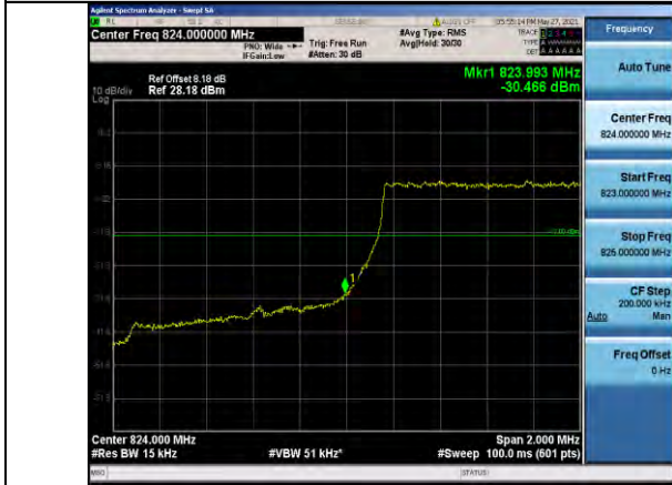
Band5-1.4MHz-QPSK-20407-6RB#0
