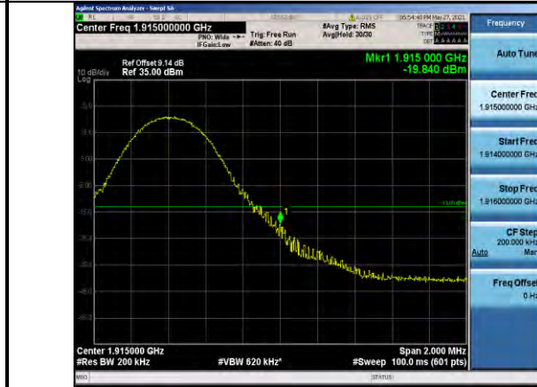
Band25-10MHz-16QAM-26640-1RB#49
