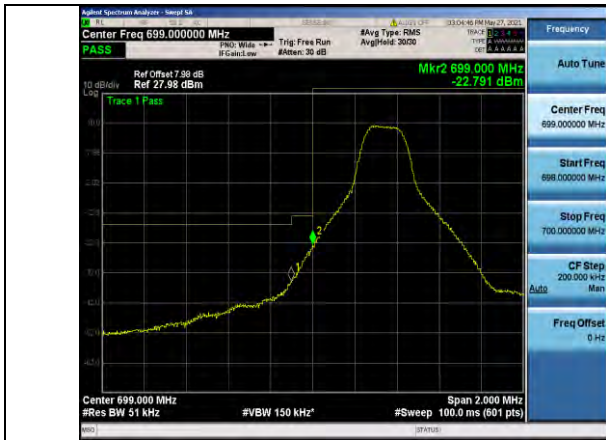
Band12-5MHz-QPSK-23035-1RB#0
