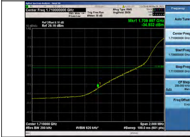
Band4-20MHz-16QAM-20050-1RB#0
