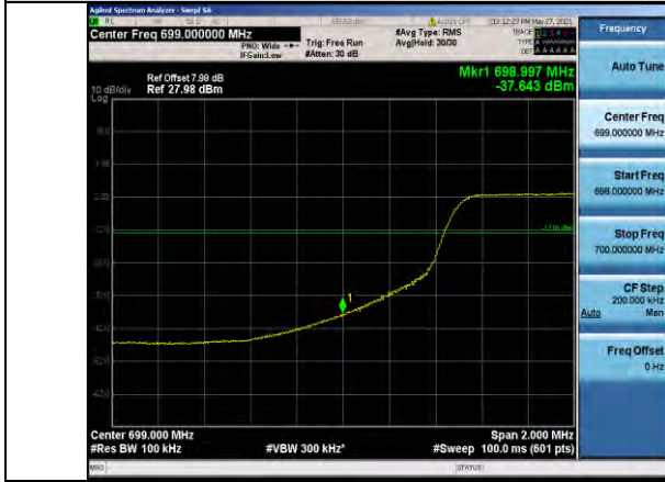
Band12-10MHz-16QAM-23060-50RB#0
