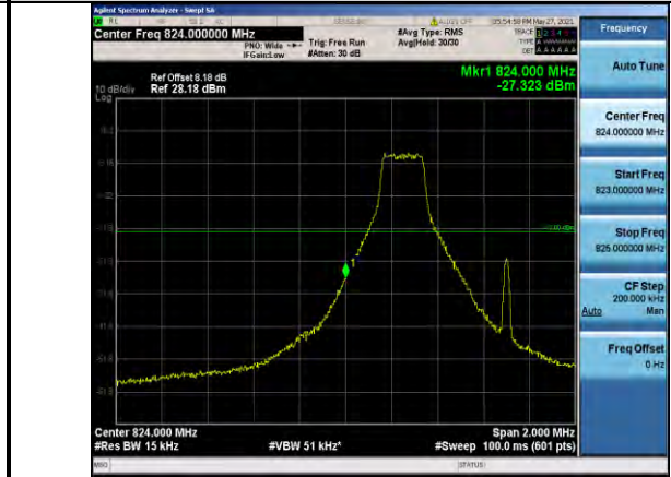
Band5-1.4MHz-16QAM-20407-1RB#0
