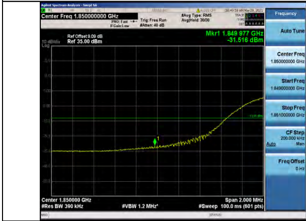
Band25-20MHz-16QAM-26140-100RB#0
