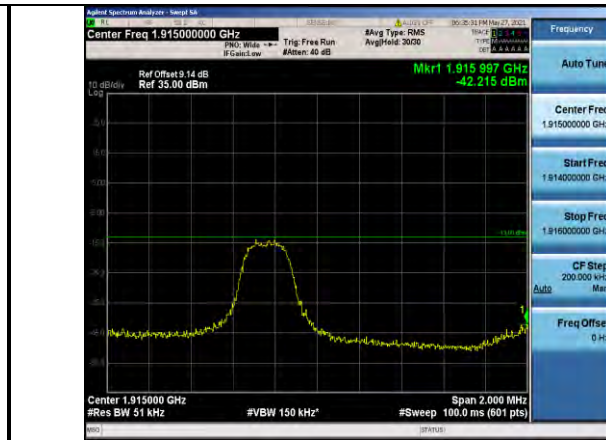
Band25-3MHz-16QAM-26675-1RB#0
