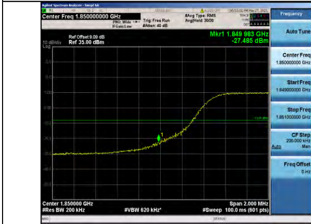
Band25-10MHz-QPSK-26090-50RB#0
