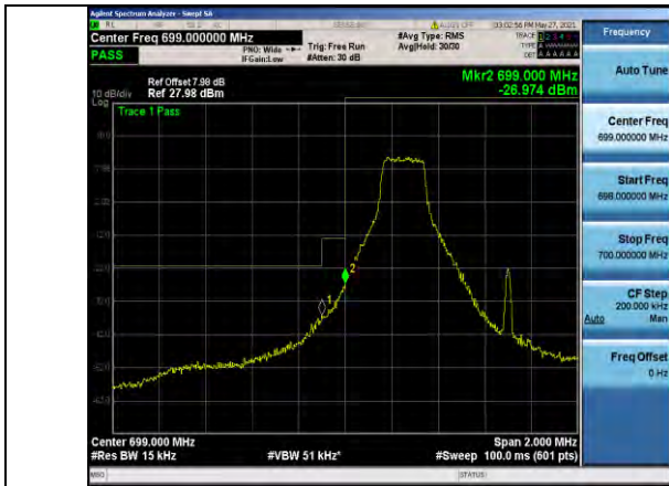
Band12-1.4MHz-16QAM-23017-1RB#0
