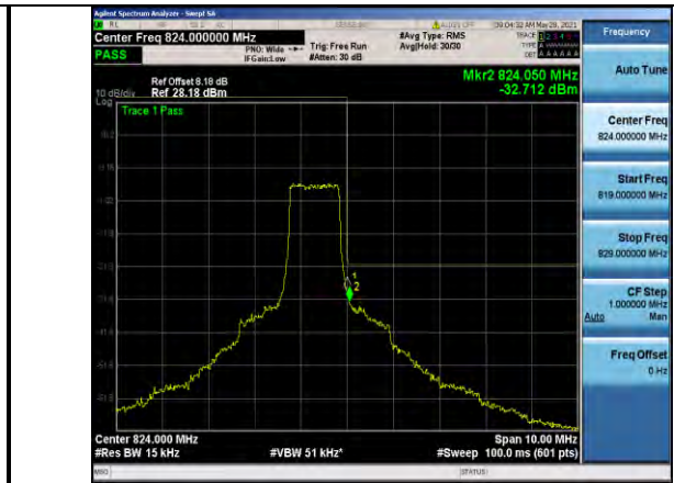
Band26-1.4MHz-QPSK-26783-6RB#0
