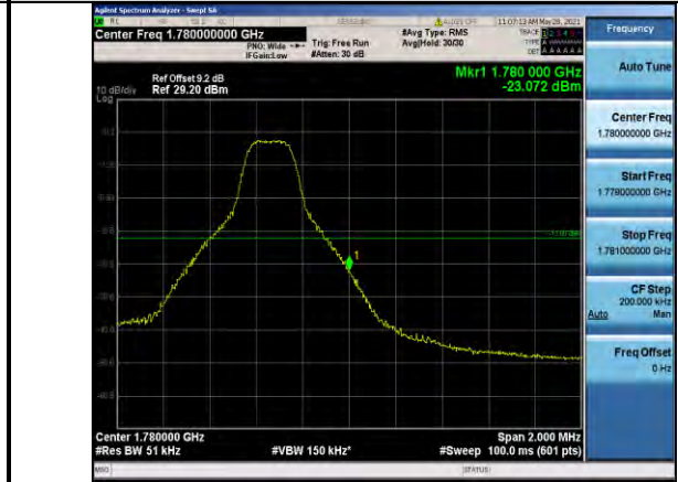
Band66-5MHz-QPSK-132647-1RB#24
