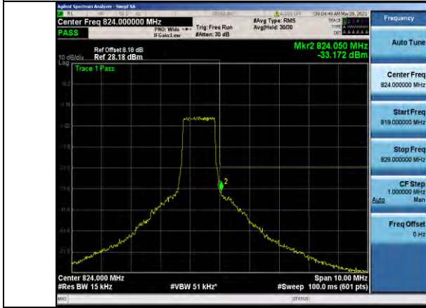
Band26-1.4MHz-16QAM-26783-6RB#0
