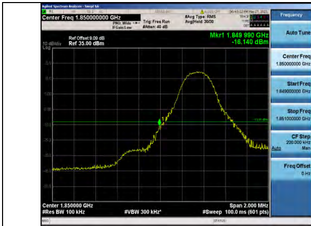
Band25-5MHz-16QAM-26065-1RB#0
