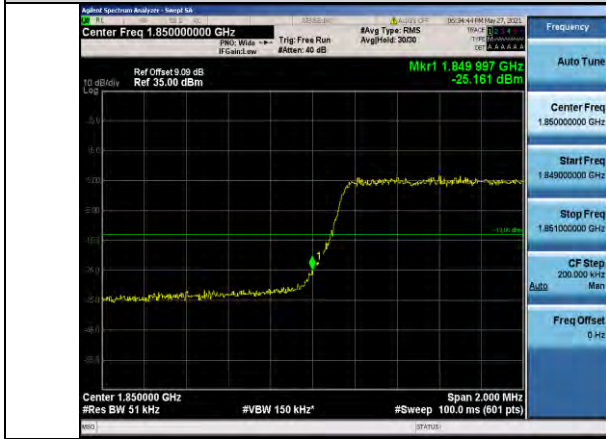
Band25-3MHz-16QAM-26055-15RB#0
