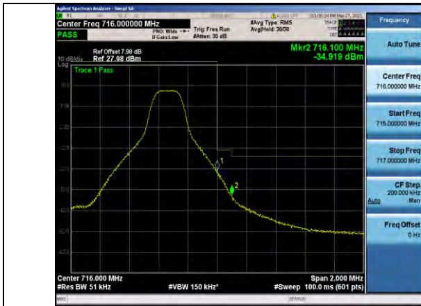
Band12-5MHz-16QAM-23155-1RB#24
