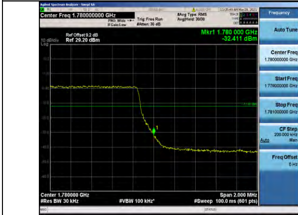
Band66-3MHz-16QAM-132657-15RB#0
