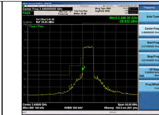
Band41-5MHz-QPSK-39675-25RB#0
