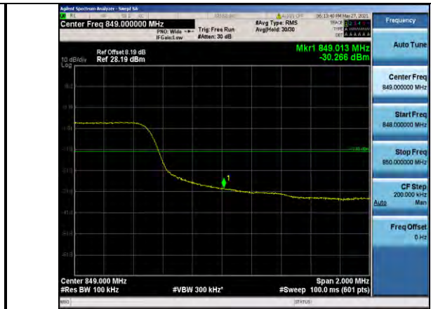
Band5-10MHz-QPSK-20600-50RB#0
