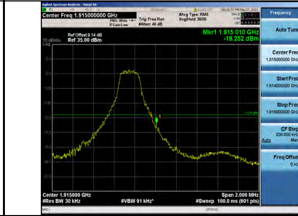
Band25-1.4MHz-QPSK-26683-1RB#5
