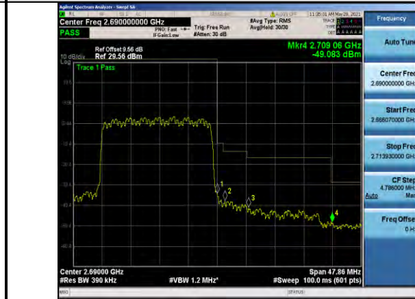
Band41-20MHz-QPSK-41490-100RB#0
