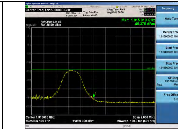
Band25-5MHz-16QAM-26665-1RB#0
