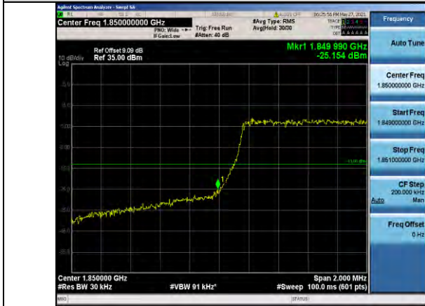
Band25-1.4MHz-16QAM-26047-6RB#0
