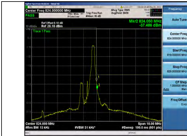
Band26-1.4MHz-16QAM-26783-1RB#5
