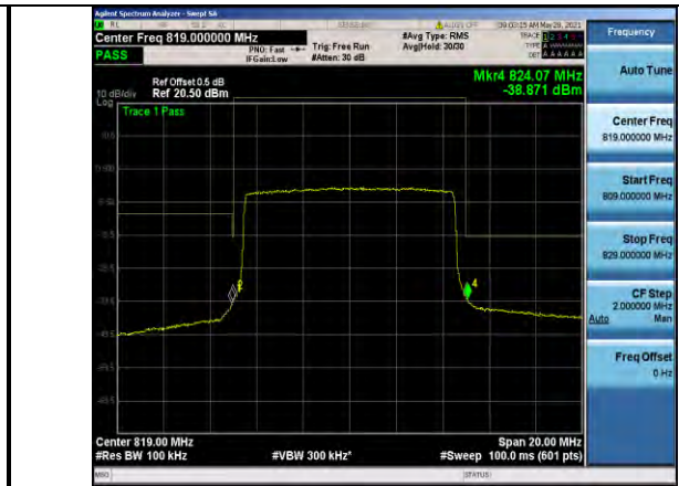
Band26-10MHz-QPSK-26740 Right-50RB#0
