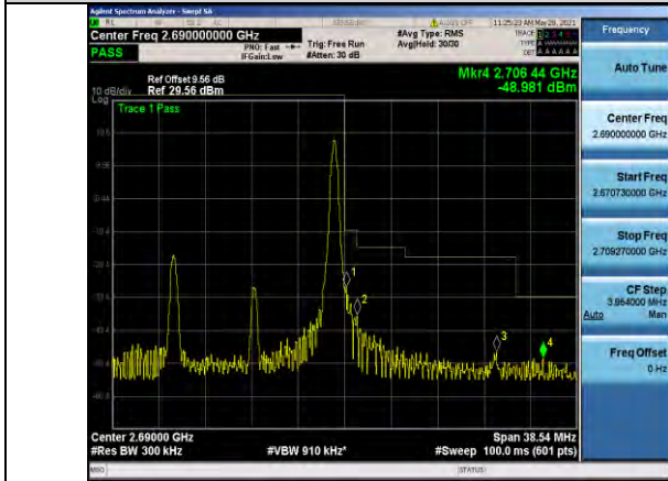
Band41-15MHz-QPSK-41515-1RB#74
