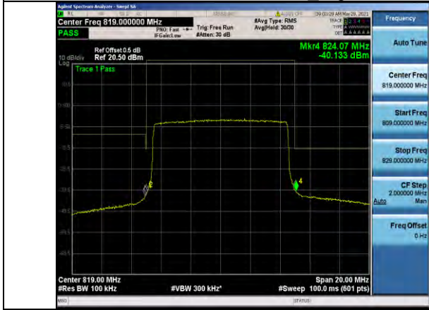
Band26-10MHz-16QAM-26740_Right-50RB#0
