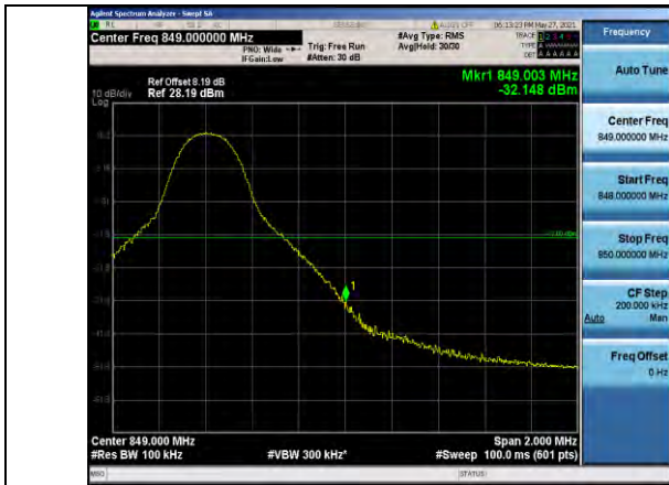
Band5-10MHz-16QAM-20600-1RB#49
