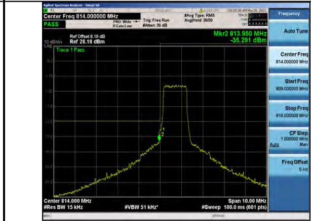
Band26-1.4MHz-16QAM-26697-6RB#0
