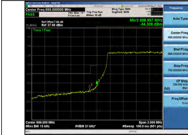
Band12-1.4MHz-16QAM-23017-6RB#0
