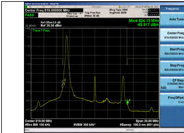
Band26-10MHz-QPSK-26740 Left-1RB#0
