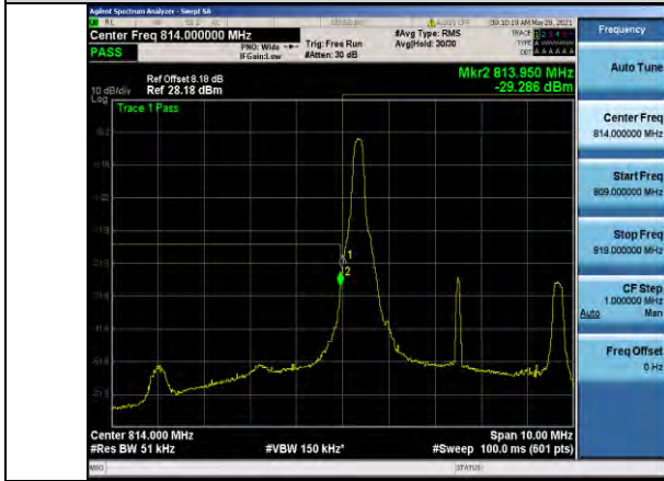
Band26-5MHz-16QAM-26715-1RB#0
