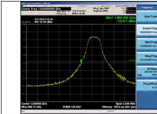
Band25-3MHz-QPSK-26055-1RB#0
