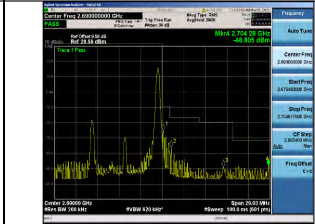
Band41-10MHz-16QAM-41540-1RB#49
