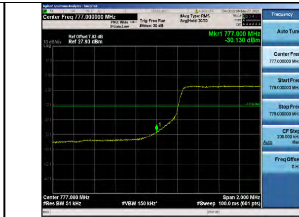
Band13-5MHz-16QAM-23205-25RB#0
