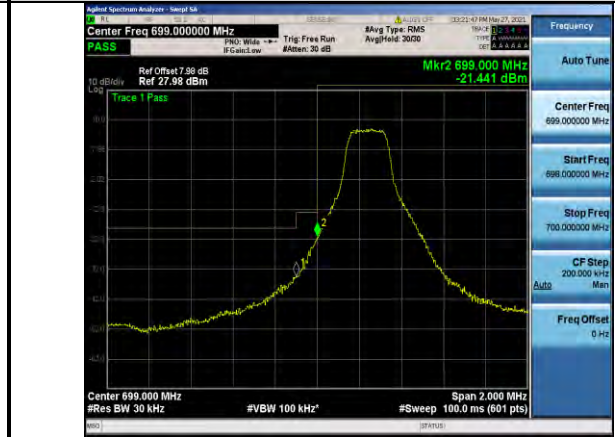
Band12-3MHz-QPSK-23025-1RB#0
