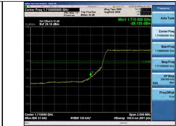
Band66-5MHz-QPSK-131997-25RB#0
