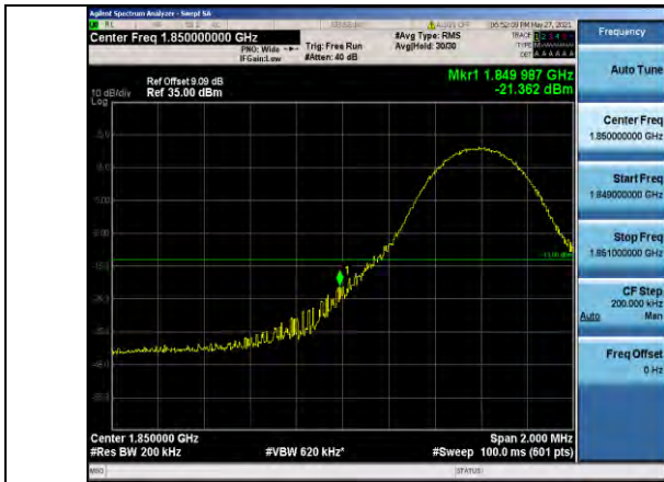
Band25-10MHz-16QAM-26090-1RB#0
