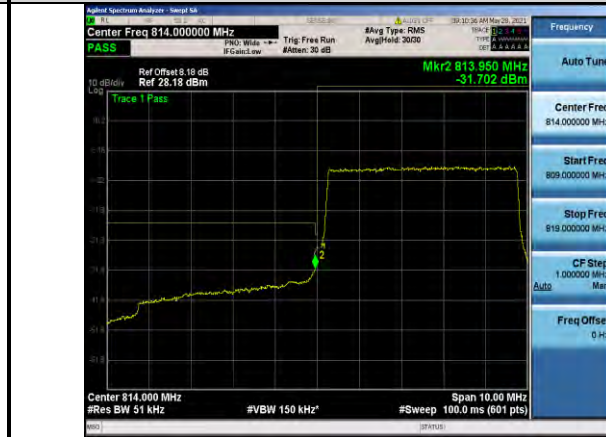
Band26-5MHz-QPSK-26715-25RB#0
