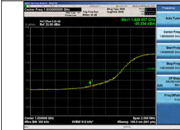
Band25-15MHz-QPSK-26115-75RB#0
