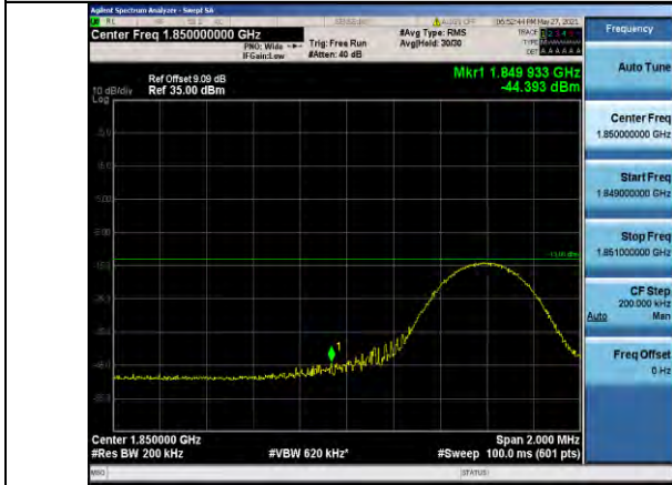
Band25-10MHz-16QAM-26090-1RB#49
