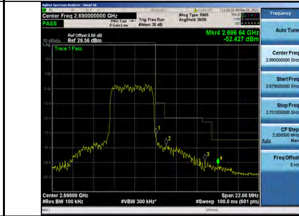
Band41-5MHz-QPSK-41565-25RB#0
