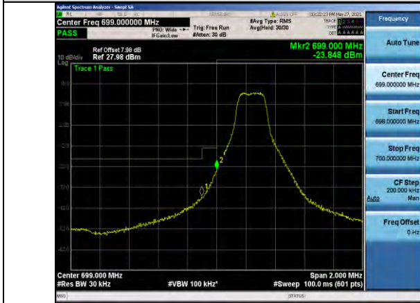
Band12-3MHz-16QAM-23025-1RB#0
