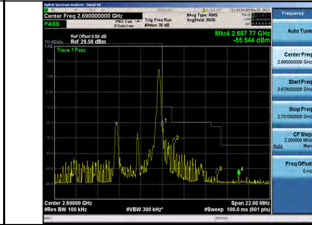
Band41-5MHz-QPSK-41565-1RB#24
