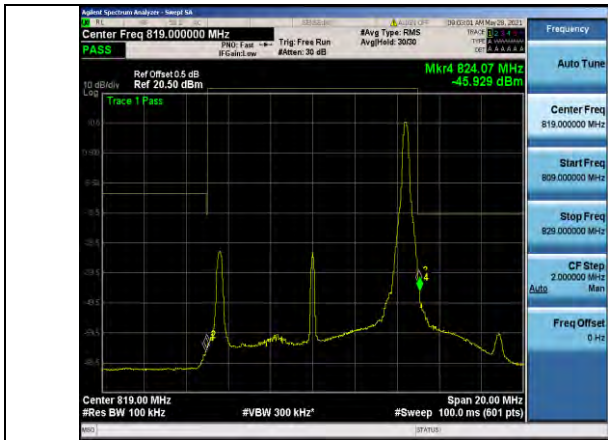
Band26-10MHz-16QAM-26740_Right-1RB#49
