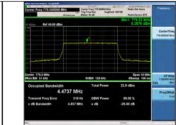
Band13-5MHz-16QAM-23205-25RB#0-4.4737
