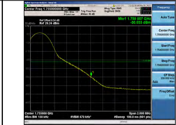
Band4-15MHz-QPSK-20325-1RB#74
