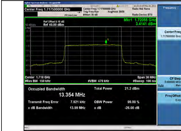
Band66-15MHz-16QAM-132047-75RB#0-13.354
