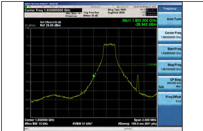
Band2-1.4MHz-QPSK-18607-1RB#0
