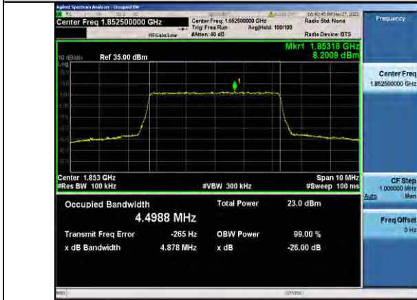
Band25-5MHz-QPSK-26065-25RB#0-4.4988
