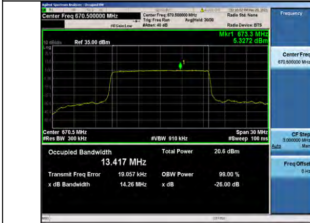
Band71-15MHz-16QAM-133197-75RB#0-13.417
