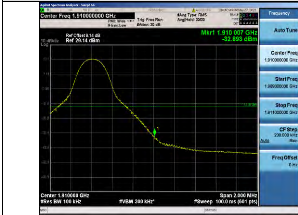
Band2-10MHz-QPSK-19150-1RB#49
