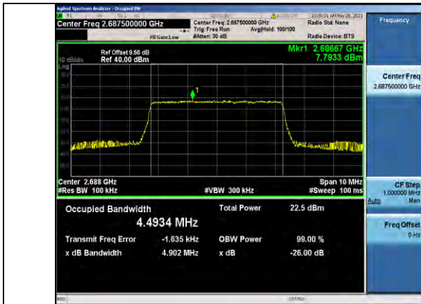
Band41-5MHz-QPSK-41565-25RB#0-4.4934
