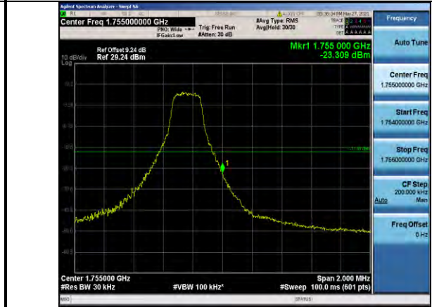
Band4-3MHz-QPSK-20385-1RB#14
