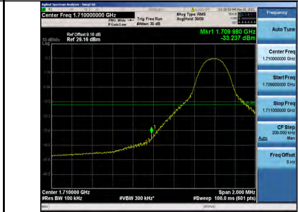
Band4-10MHz-16QAM-20000-1RB#0
