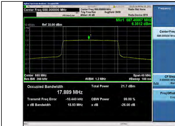
Band71-20MHz-QPSK-133372-100RB#0-17.889
