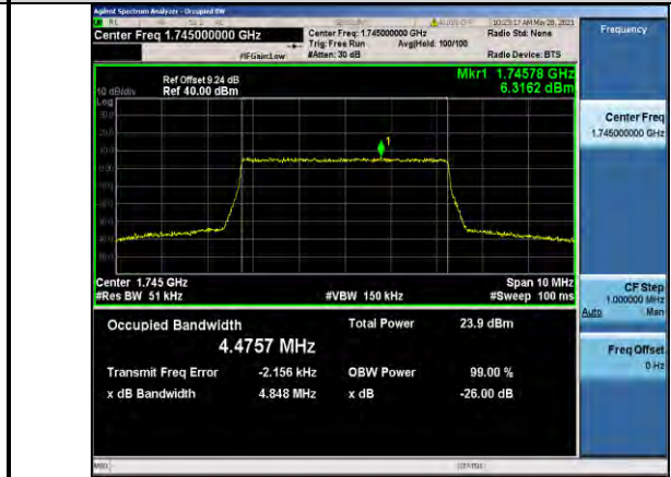
Band66-5MHz-QPSK-132322-25RB#0-4.4757
