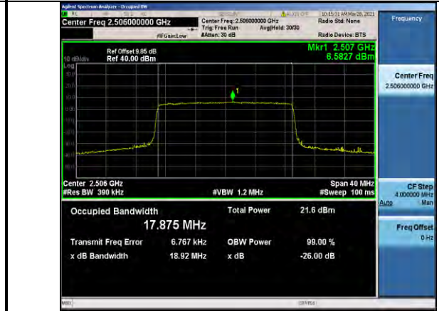
Band41-20MHz-QPSK-39750-100RB#0-17.875
