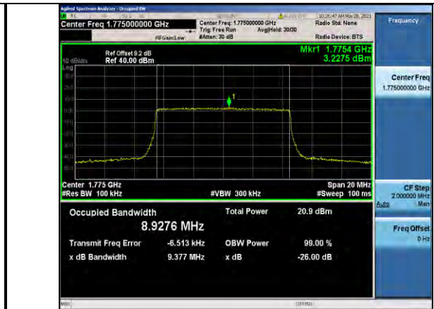
Band66-10MHz-16QAM-132622-50RB#0-8.9276
