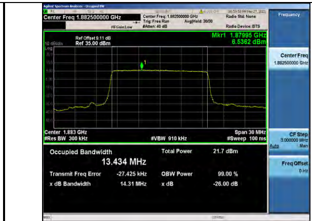
Band25-15MHz-QPSK-26365-75RB#0-13.434
