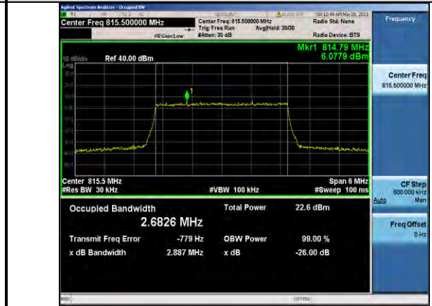
Band26-3MHz-16QAM-26705-15RB#0-2.6826
