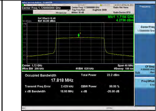
Band66-20MHz-QPSK-132072-100RB#0-17.818
