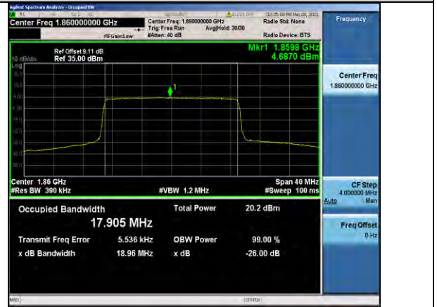
Band25-20MHz-16QAM-26140-100RB#0-17.905
