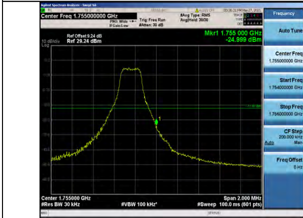
Band4-3MHz-16QAM-20385-1RB#14
