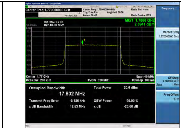
Band66-20MHz-16QAM-132572-100RB#0-17.802
