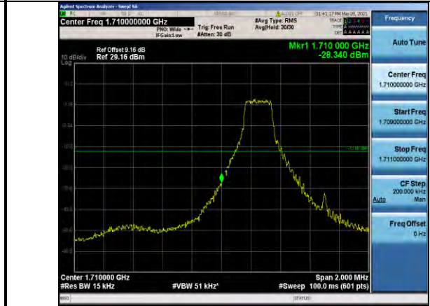
Band4-1.4MHz-16QAM-19957-1RB#0
