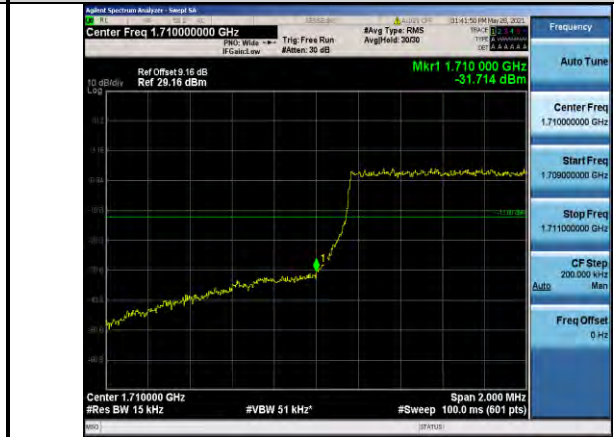
Band4-1.4MHz-16QAM-19957-6RB#0
