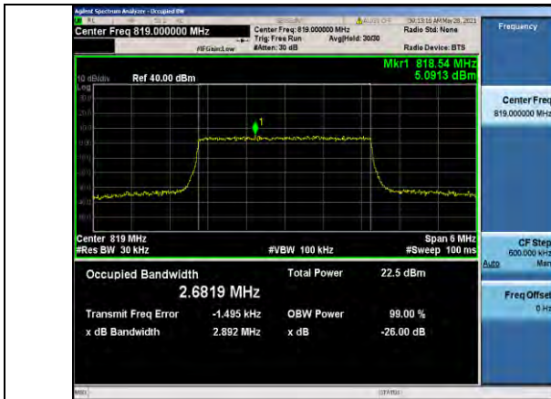
Band26-3MHz-16QAM-26740-15RB#0-2.6819
