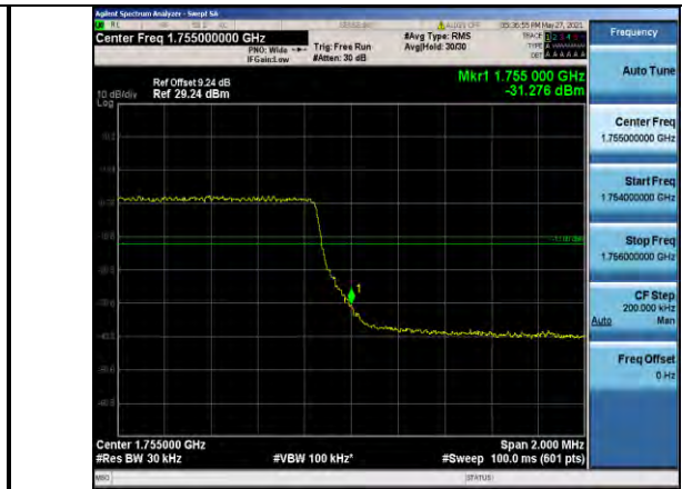
Band4-3MHz-16QAM-20385-15RB#0
