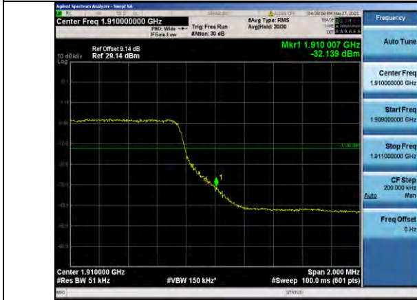
Band2-5MHz-QPSK-19175-25RB#0
