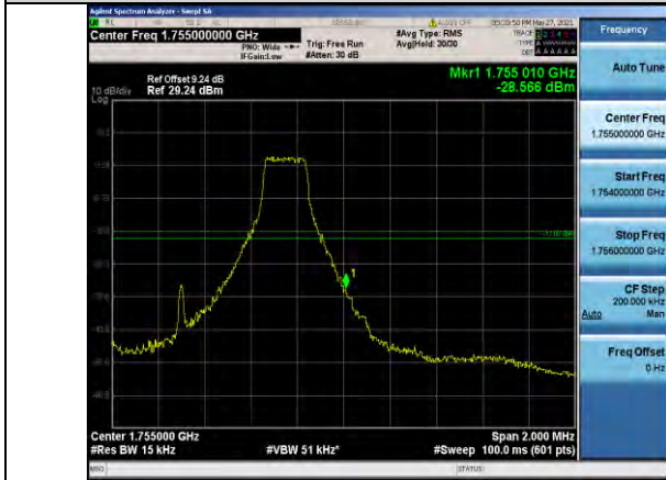
Band4-1.4MHz-QPSK-20393-1RB#5
