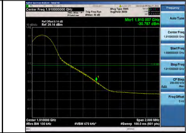
Band2-15MHz-QPSK-19125-1RB#74
