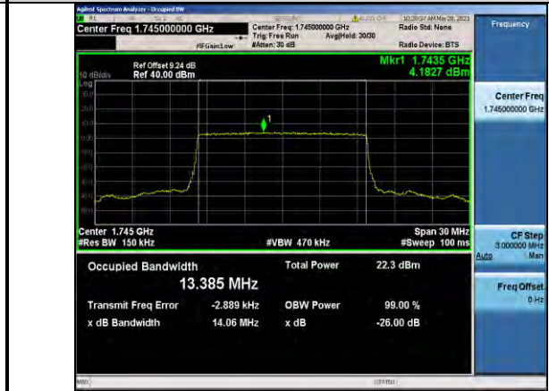
Band66-15MHz-QPSK-132322-75RB#0-13.385
