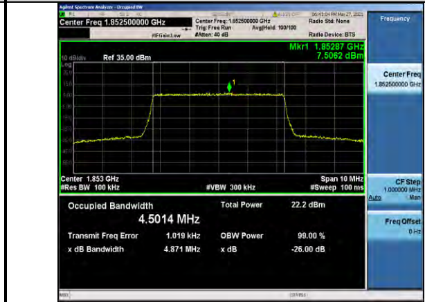
Band25-5MHz-16QAM-26065-25RB#0-4.5014
