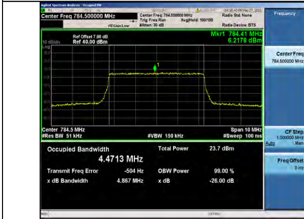
Band13-5MHz-QPSK-23255-25RB#0-4.4713
