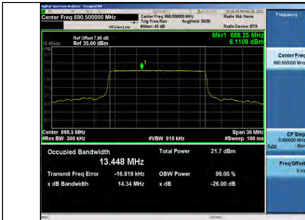
Band71-15MHz-QPSK-133397-75RB#0-13.448
