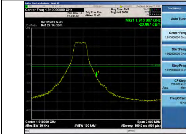
Band2-3MHz-16QAM-19185-1RB#14
