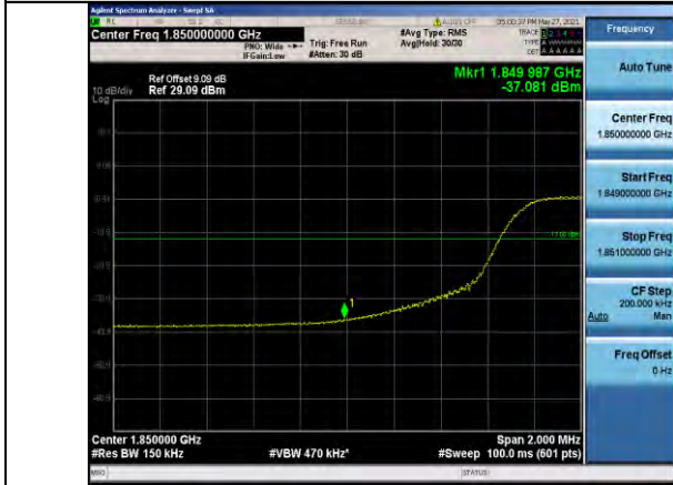
Band2-15MHz-16QAM-18675-75RB#0
