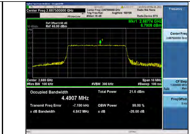
Band41-5MHz-16QAM-41565-25RB#0-4.4907
