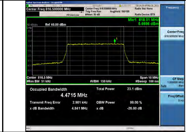
Band26-5MHz-16QAM-26715-25RB#0-4.4715
