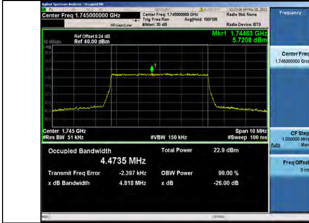
Band66-5MHz-16QAM-132322-25RB#0-4.4735
