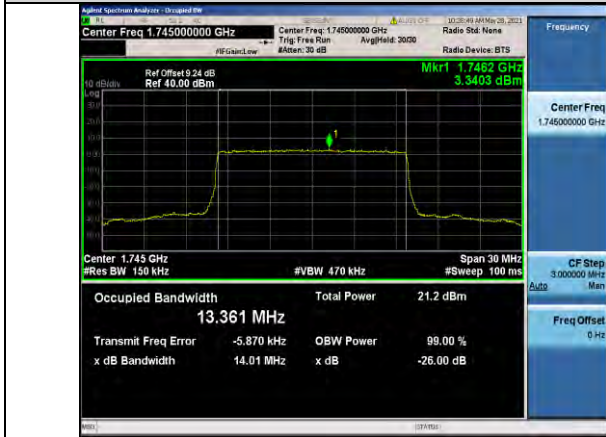
Band66-15MHz-16QAM-132322-75RB#0-13.361
