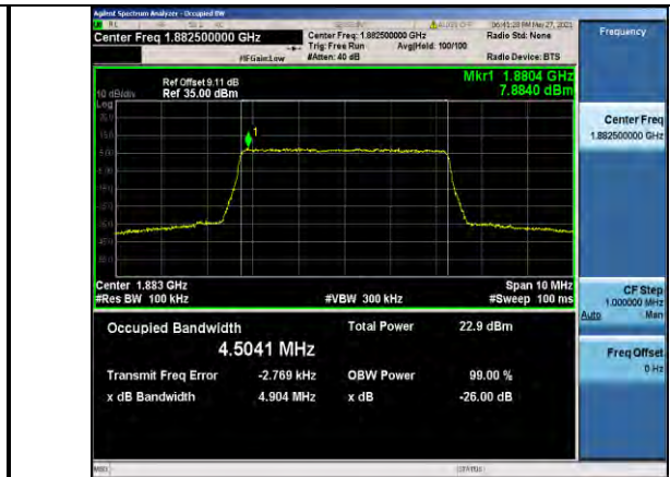
Band25-5MHz-QPSK-26365-25RB#0-4.5041
