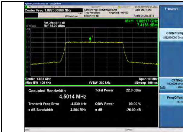
Band25-5MHz-16QAM-26365-25RB#0-4.5014
