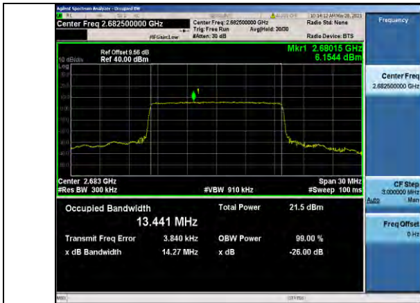
Band41-15MHz-QPSK-41515-75RB#0-13.441
