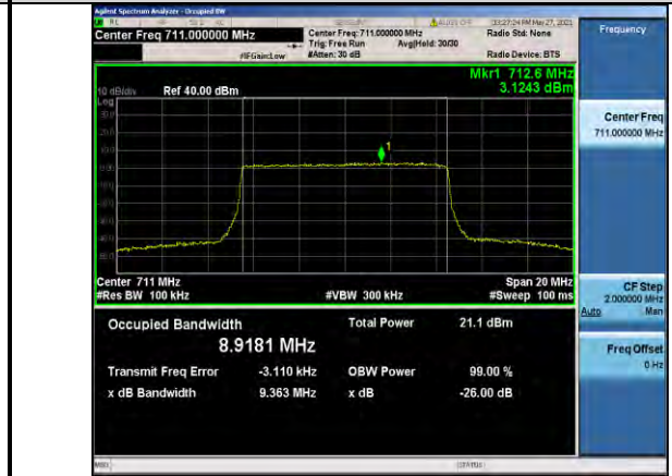
Band12-10MHz-16QAM-23130-50RB#0-8.9181
