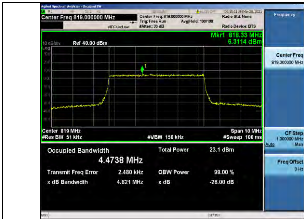
Band26-5MHz-16QAM-26740-25RB#0-4.4738
