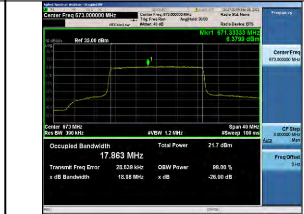
Band71-20MHz-QPSK-133222-100RB#0-17.863
