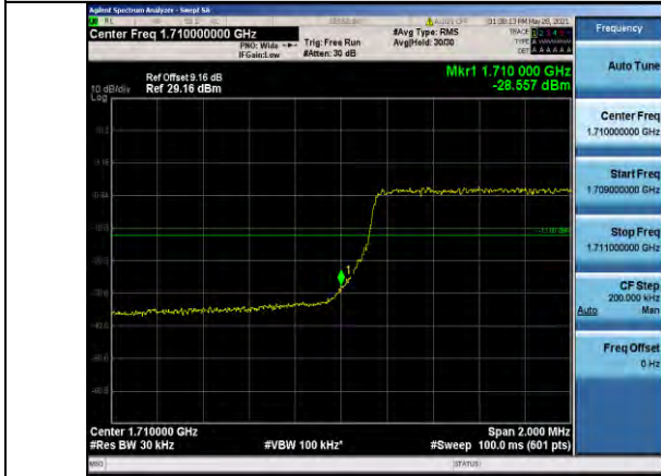
Band4-3MHz-16QAM-19965-15RB#0
