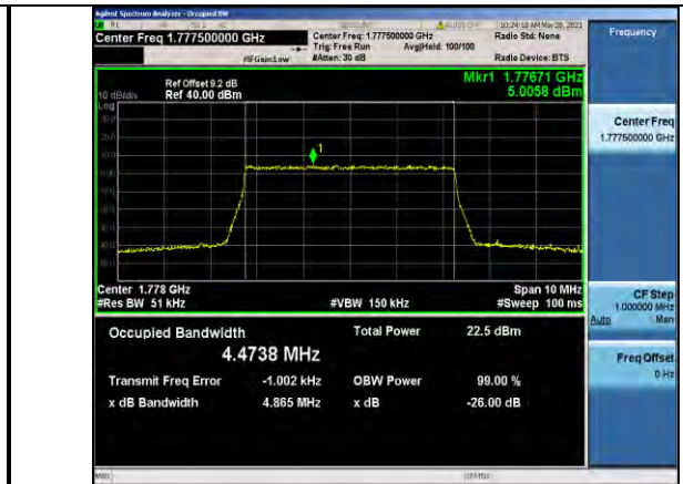
Band66-5MHz-16QAM-132647-25RB#0-4.4738
