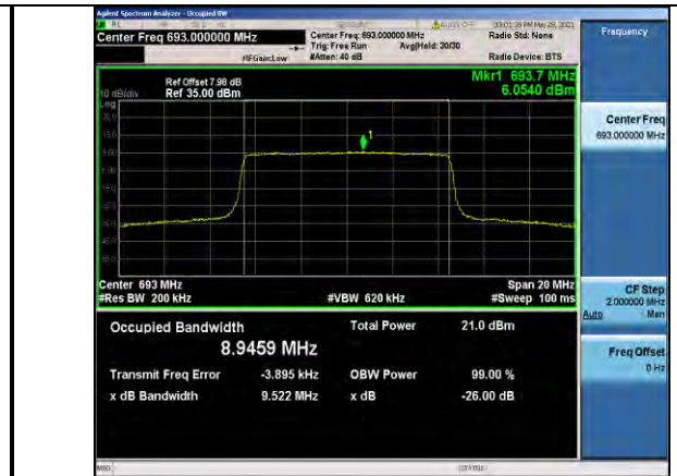
Band71-10MHz-16QAM-133422-50RB#0-8.9459
