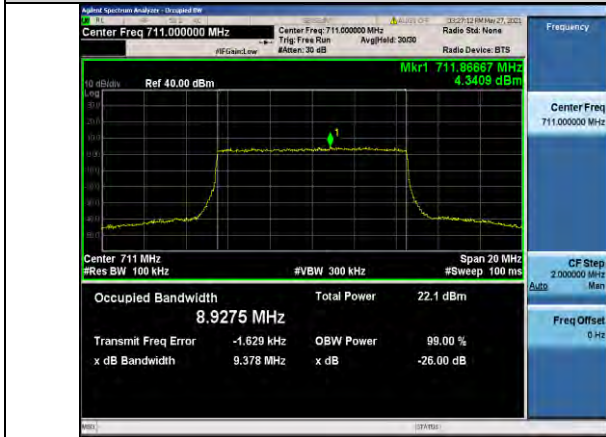
Band12-10MHz-QPSK-23130-50RB#0-8.9275
