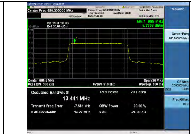
Band71-15MHz-16QAM-133397-75RB#0-13.441
