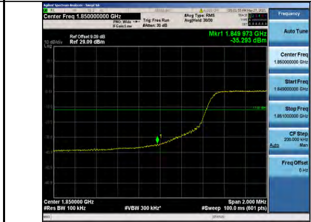
Band2-10MHz-16QAM-18650-50RB#0
