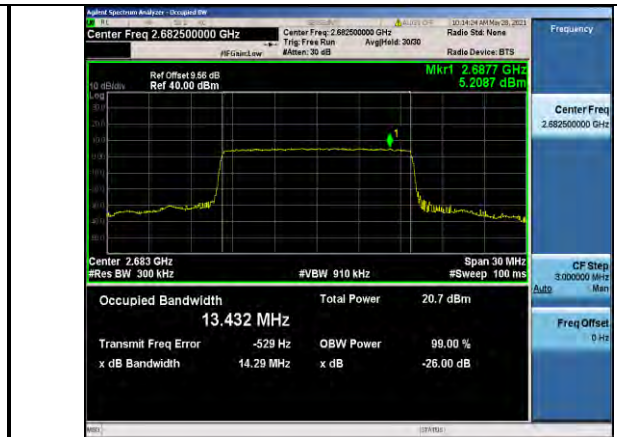
Band41-15MHz-16QAM-41515-75RB#0-13.432
