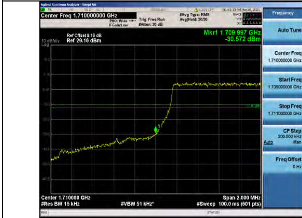
Band4-1.4MHz-QPSK-19957-6RB#0
