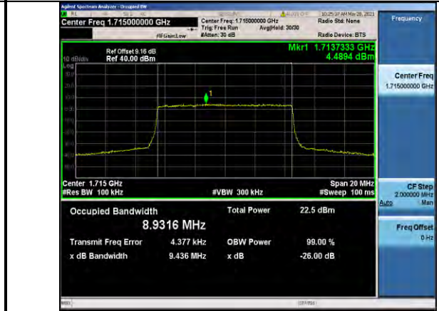
Band66-10MHz-QPSK-132022-50RB#0-8.9316
