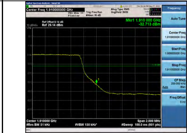
Band2-5MHz-16QAM-19175-25RB#0
