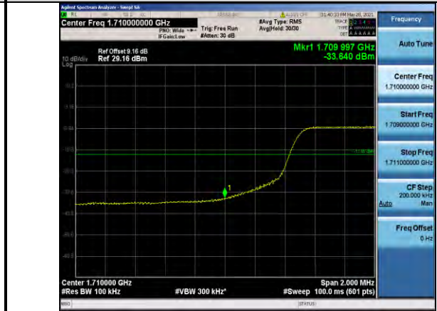
Band4-10MHz-16QAM-20000-50RB#0
