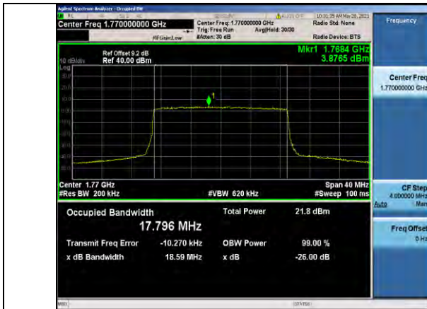
Band66-20MHz-QPSK-132572-100RB#0-17.796
