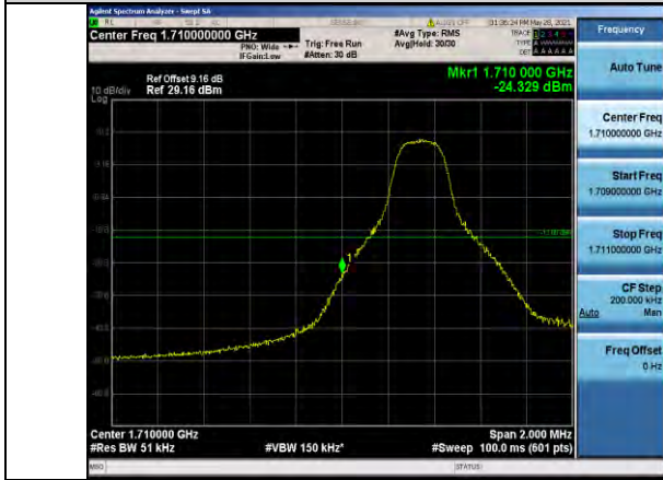
Band4-5MHz-16QAM-19975-1RB#0
