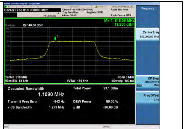
Band26-1.4MHz-QPSK-26740-6RB#0-1.1090
