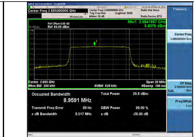
Band41-10MHz-16QAM-41540-50RB#0-8.9591
