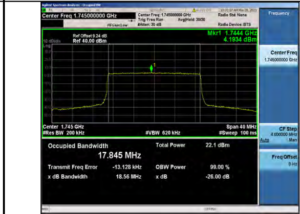
Band66-20MHz-QPSK-132322-100RB#0-17.845
