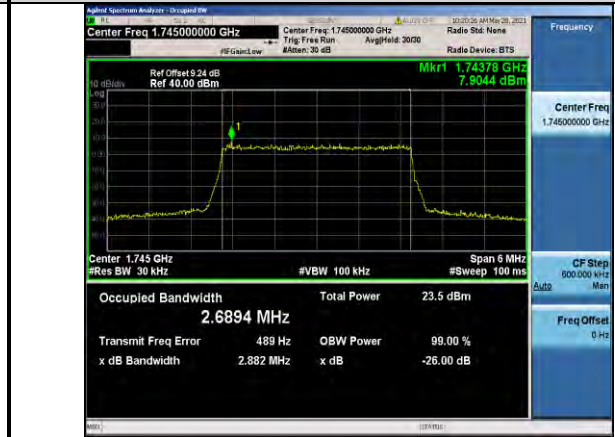
Band66-3MHz-QPSK-132322-15RB#0-2.6894
