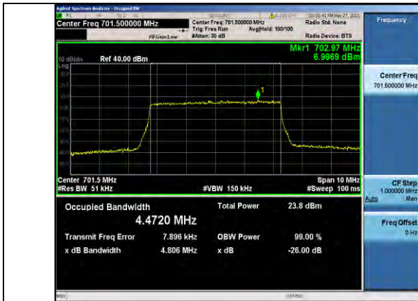
Band12-5MHz-QPSK-23035-25RB#0-4.4720
