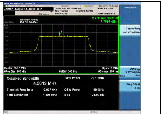
Band71-5MHz-16QAM-133447-25RB#0-4.5019
