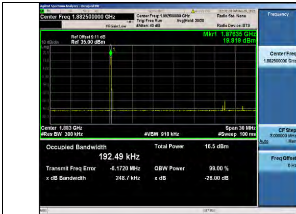
Band25-15MHz-16QAM-26365-75RB#0-0.19249
