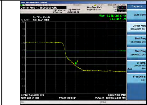
Band4-5MHz-16QAM-20375-25RB#0
