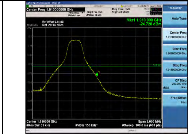
Band2-5MHz-16QAM-19175-1RB#24
