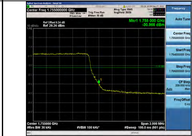
Band4-3MHz-QPSK-20385-15RB#0
