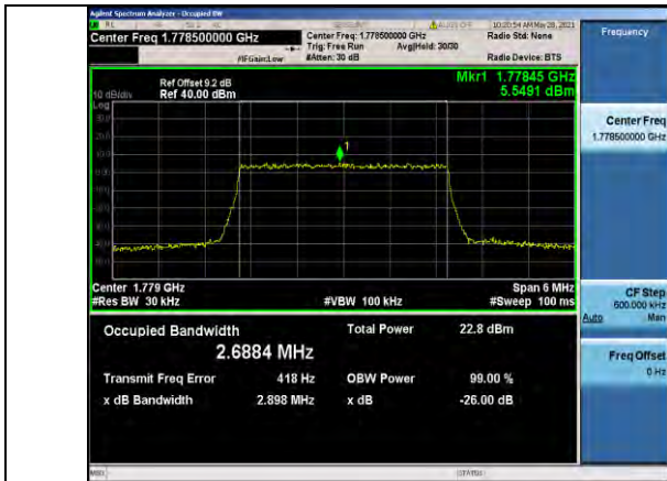
Band66-3MHz-QPSK-132657-15RB#0-2.6884
