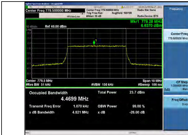
Band13-5MHz-QPSK-23205-25RB#0-4.4699
