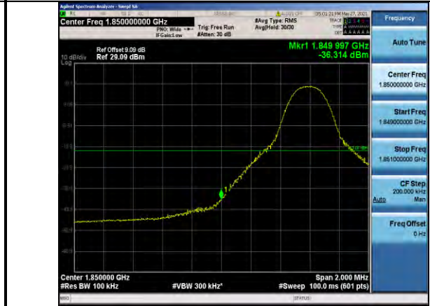
Band2-10MHz-16QAM-18650-1RB#0
