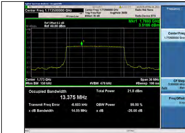
Band66-15MHz-QPSK-132597-75RB#0-13.375
