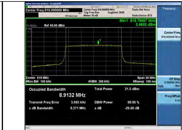
Band26-10MHz-16QAM-26740-50RB#0-8.9132
