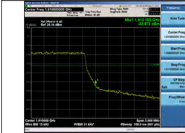
Band2-1.4MHz-16QAM-19193-6RB#0
