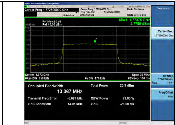
Band66-15MHz-16QAM-132597-75RB#0-13.367
