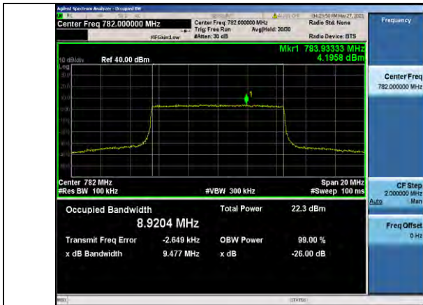
Band13-10MHz-QPSK-23230-50RB#0-8.9204
