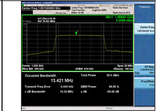
Band25-15MHz-16QAM-26115-75RB#0-13.421
