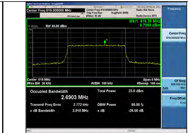
Band26-3MHz-QPSK-26740-15RB#0-2.6903
