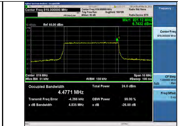
Band26-5MHz-QPSK-26740-25RB#0-4.4771
