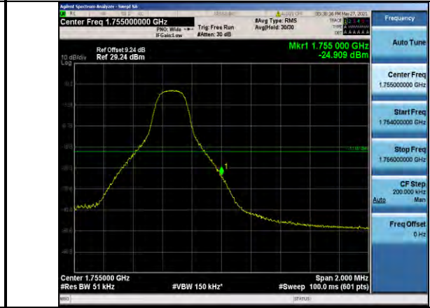
Band4-5MHz-16QAM-20375-1RB#24
