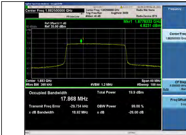
Band25-20MHz-16QAM-26365-100RB#0-17.868
