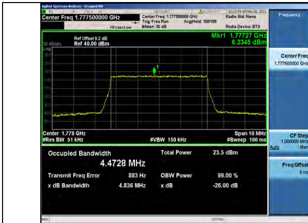
Band66-5MHz-QPSK-132647-25RB#0-4.4728
