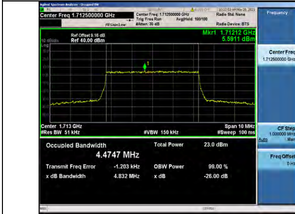
Band66-5MHz-16QAM-131997-25RB#0-4.4747
