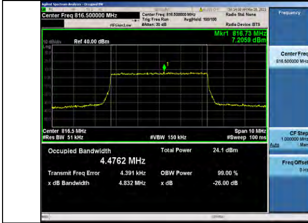
Band26-5MHz-QPSK-26715-25RB#0-4.4762
