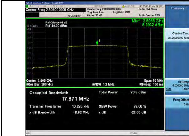
Band41-20MHz-16QAM-39750-100RB#0-17.871
