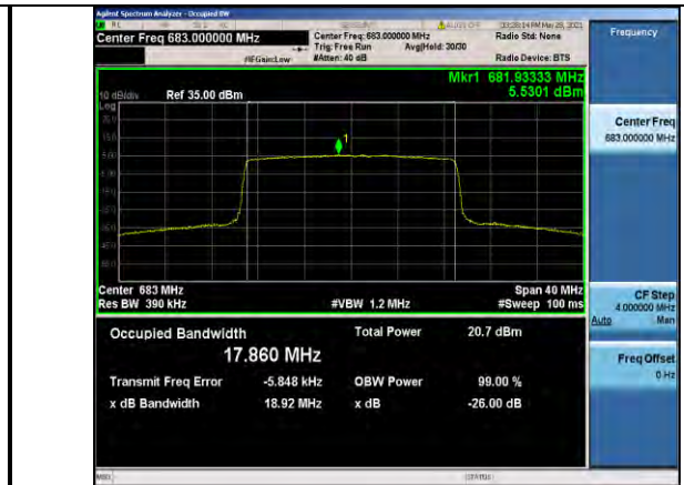
Band71-20MHz-16QAM-133322-100RB#0-17.860
