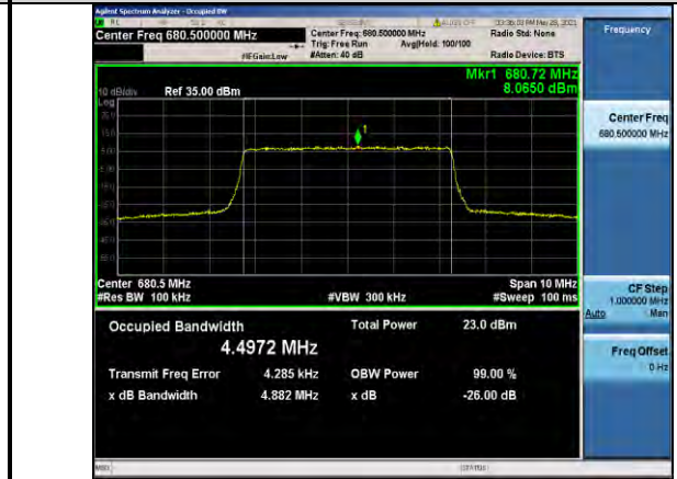
Band71-5MHz-QPSK-133297-25RB#0-4.4972
