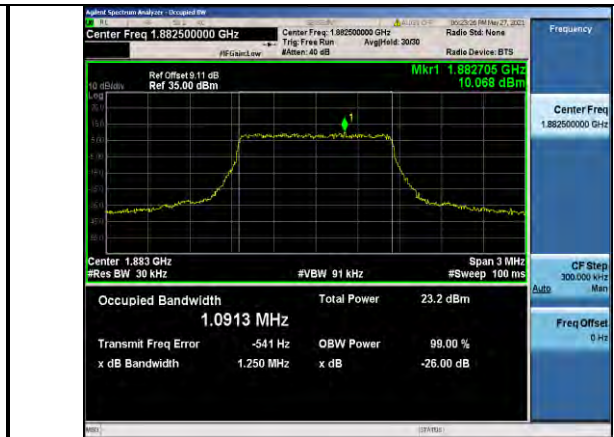
Band25-1.4MHz-QPSK-26365-6RB#0-1.0913
