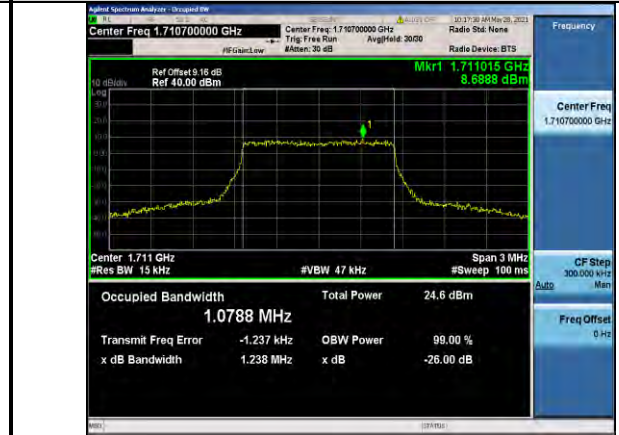
Band66-1.4MHz-QPSK-131979-6RB#0-1.0788
