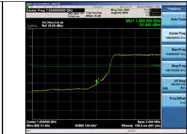
Band2-5MHz-16QAM-18625-25RB#0
