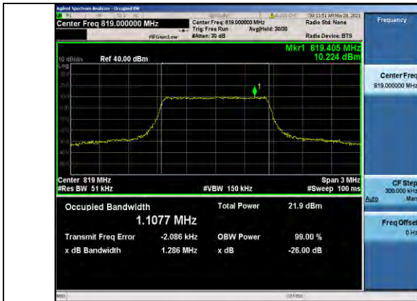
Band26-1.4MHz-16QAM-26740-6RB#0-1.1077
