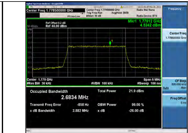
Band66-3MHz-16QAM-132657-15RB#0-2.6834
