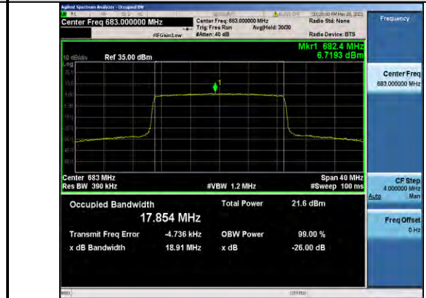
Band71-20MHz-QPSK-133322-100RB#0-17.854
