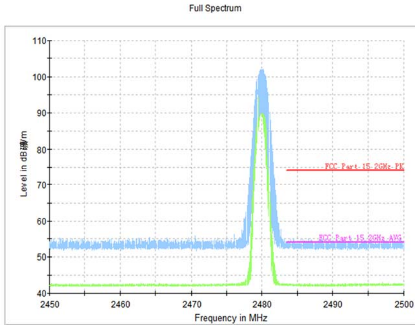
Fig.16. Frequency Band Edges: \pi/4 DQPSK, Channel 78, 2.45GHz - 2.50GHz
