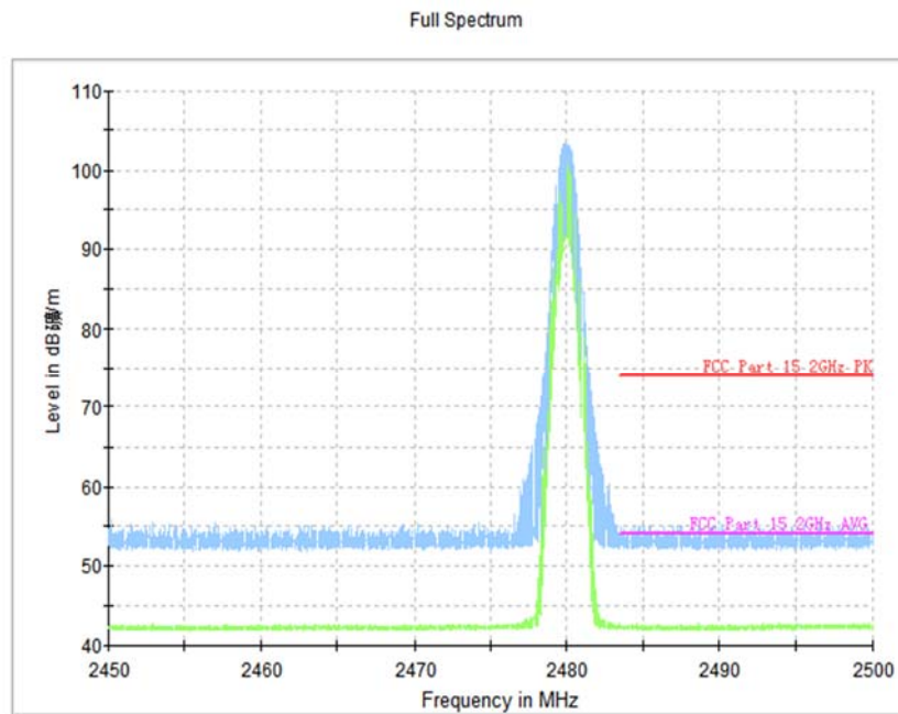
Fig.14. Frequency Band Edges: GFSK, Channel 78, 2.45GHz - 2.50GHz
