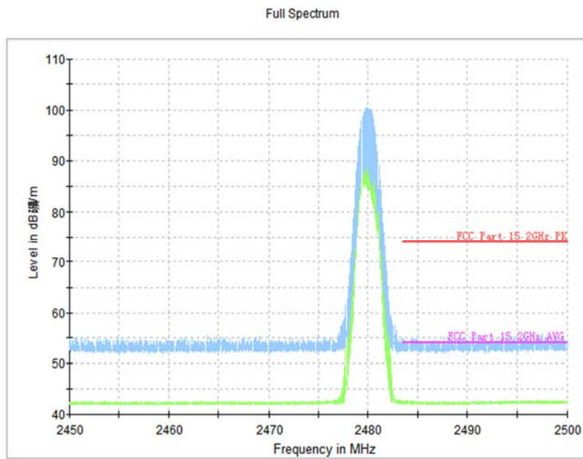
Fig.18. Frequency Band Edges: 8DPSK, Channel 78, 2.45 GHz - 2.50
