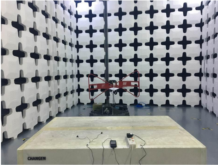
3. Radiated Emissions (Part 15B Charger Mode, 30MHz-1GHz)
