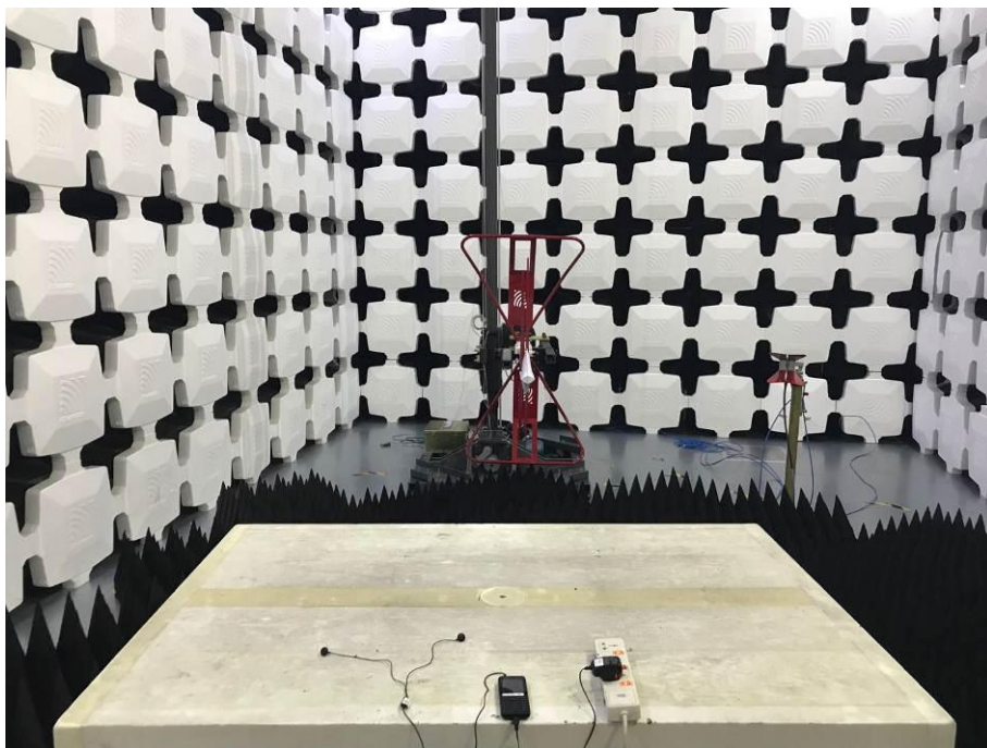
4. Radiated Emissions (Part 15B Charger Mode, 1GHz-18GHz)
