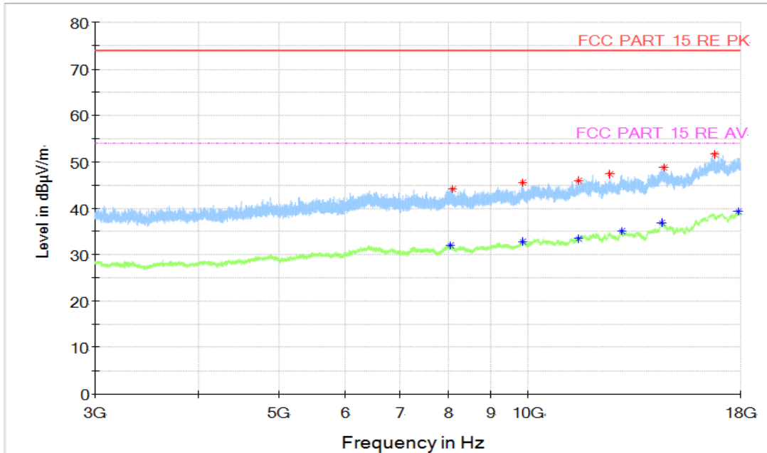
Figure A.6 Radiated Emission (Set.1, Charging and WCDMA Band 5 idle , 3GHz to 18GHz)
