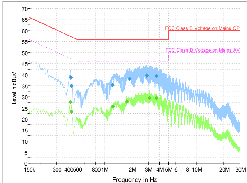
Fig.A.11.1 AC Powerline Conducted Emission-802.11b
