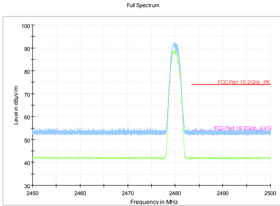
Fig.18. Frequency Band Edges: 8DPSK, Channel 78, 2.45 GHz - 2.50GHz
