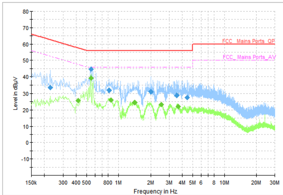
Fig.81 AC Power line Conducted Emission (Idle, AE2, 120V)
