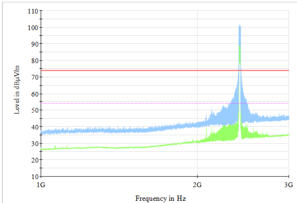
Fig.61 Radiated Spurious Emission (802.11n HT20, CH1, 1GHz-3GHz)
