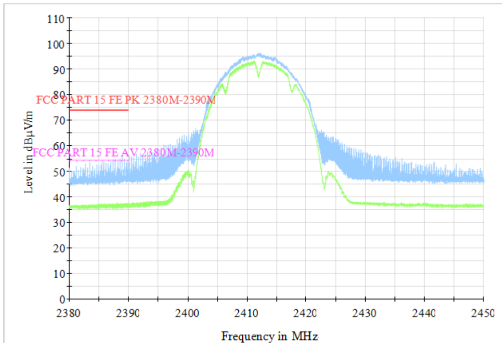
Fig.51 Radiated Restricted Band (802.11b, CH1, 2.38GHz~2.45GHz)
