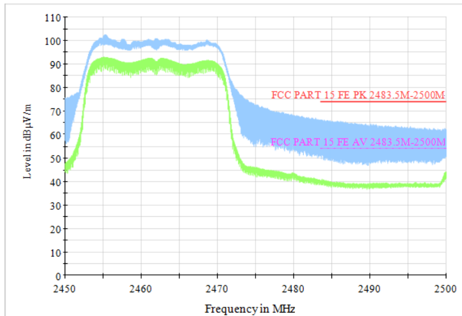
Fig.68 Radiated Restricted Band (802.11n HT20, CH11, 2.45GHz~2.5GHz)
