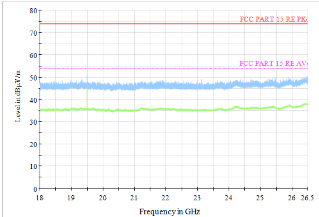
Fig.79 Radiated Spurious Emission (All Channels, 18GHz-26.5GHz)
