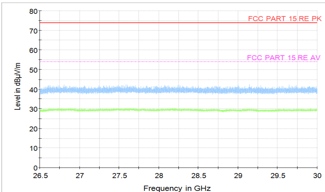
Figure A.5 Radiated Emission (Set.1, Data Transfer Mode , 26.5GHz to 30GHz)
