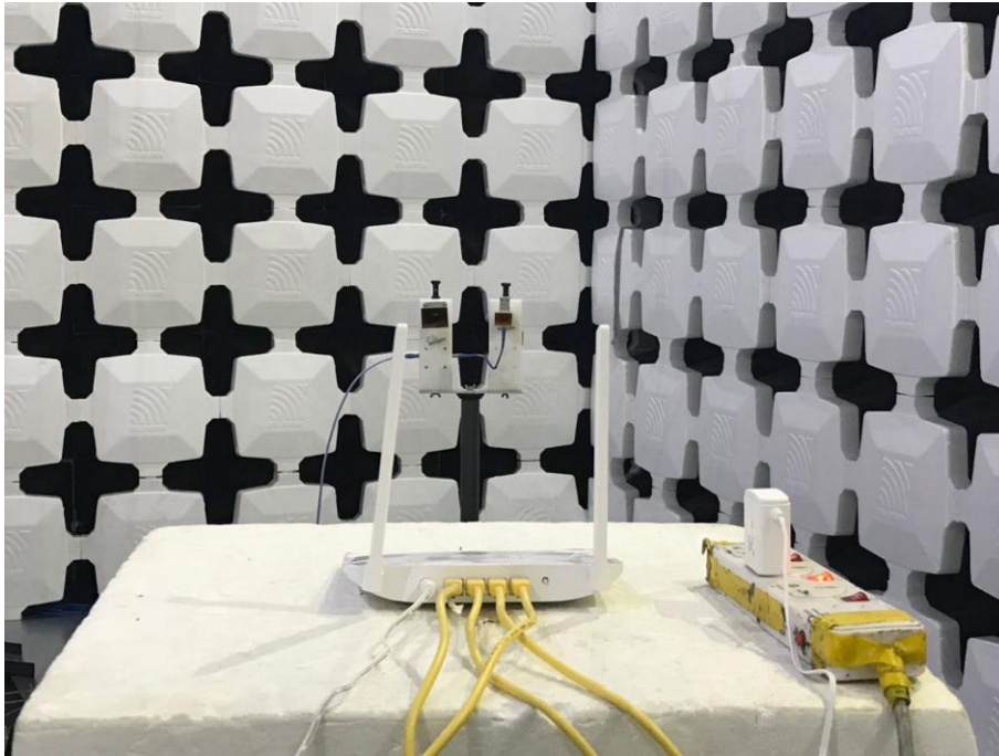
7. Radiated Emissions (Part 15C&15E) (18-26.5GHz)
