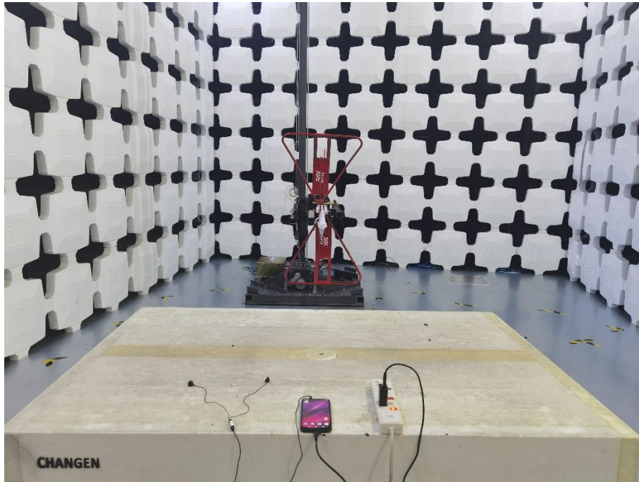
3. Radiated Emissions (Part 15B GSM receiver/WCDMA receiver/Camera/ Video Player/FM receiver,30MHz-1GHz)
