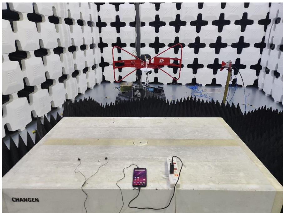
4. Radiated Emissions (Part 15B GSM receiver/WCDMA receiver/Camera/ Video Player/FM receiver,1GHz-18GHz)
