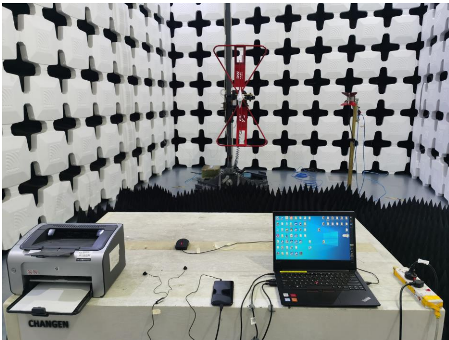
4. Radiated Emissions (Part 15B, Data Transfer Mode) (1GHz-18GHz)
