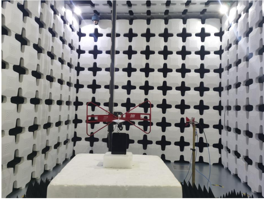
9. Radiated Spurious Emissions (Part 22/24/27) (30MHz-18GHz)
