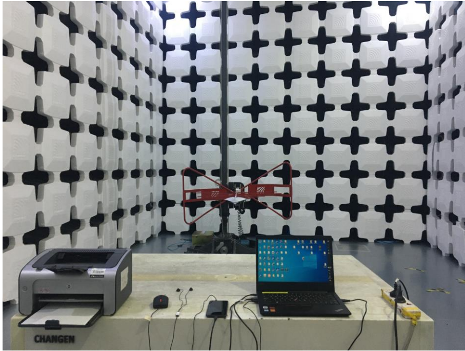
3. Radiated Emissions (Part 15B, Data Transfer Mode) (30MHz-1GHz)
