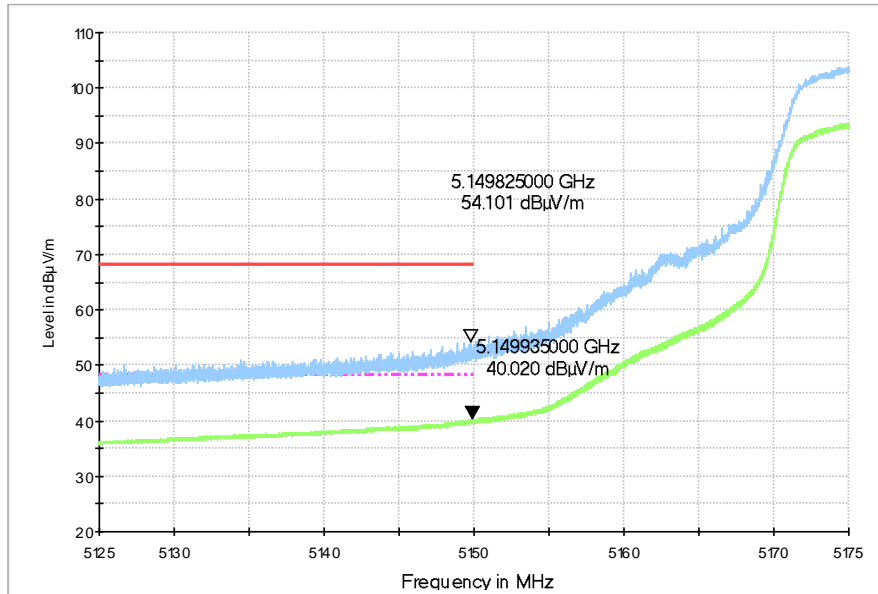
Fig.19 Band Edges (802.11ac-HT20, 5180MHz)
