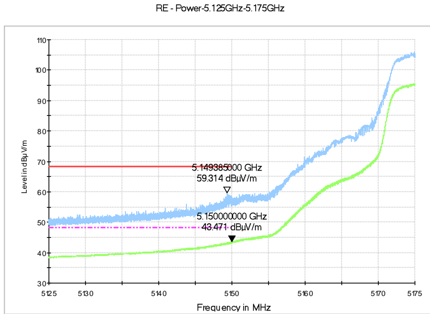
Fig.15 Band Edges (802.11a, 5180MHz)
