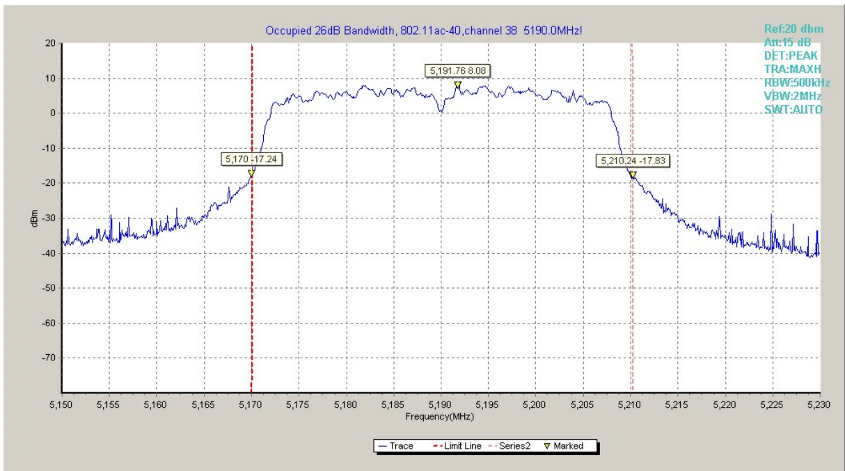
Fig.12 Occupied 26dB Bandwidth (802.11ac-HT40, 5190MHz)
