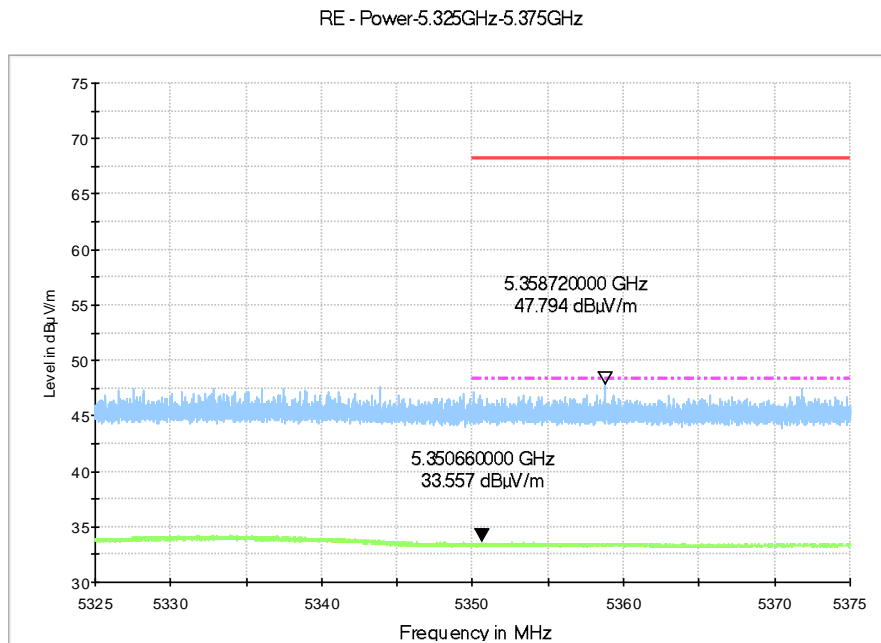
Fig.16 Band Edges (802.11a, 5320MHz)
