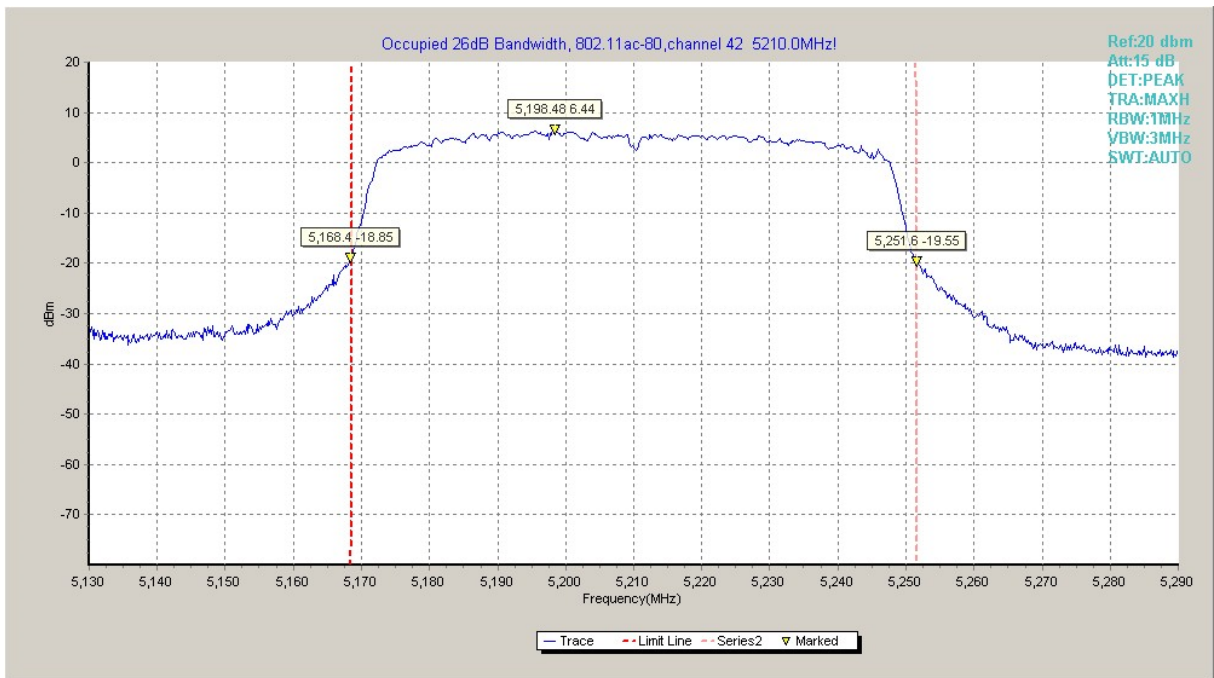
Fig.14 Occupied 26dB Bandwidth (802.11ac-HT80, 5210MHz)
