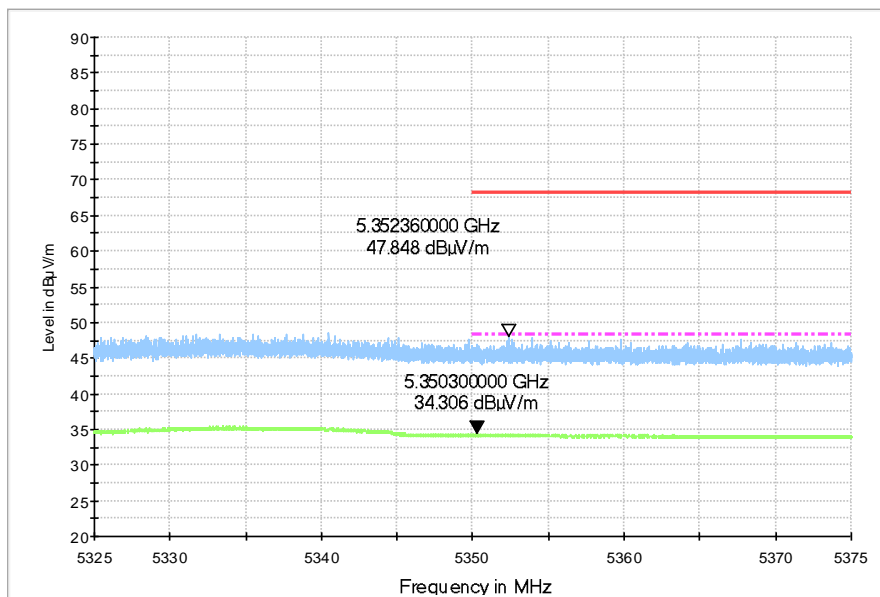
Fig.20 Band Edges (802.11ac-HT20, 5320MHz)
