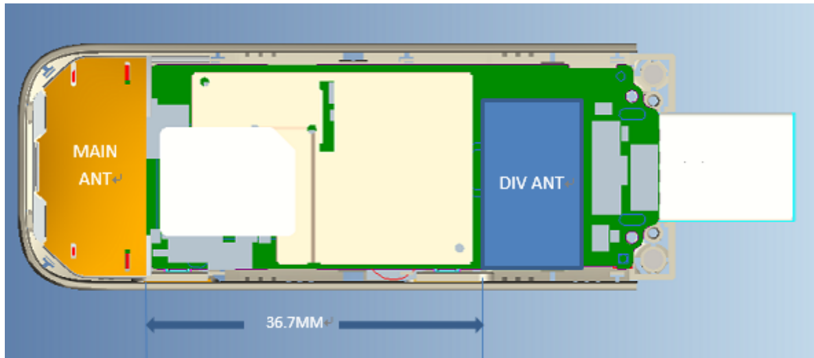
Picture 12.1 Antenna Position and size
