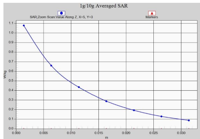
Fig. 1-3 Z-Scan at power reference point (WCDMA850 Body)
