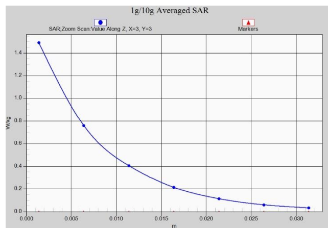
Fig. 1-6 Z-Scan at power reference point (LTE band40 Body)
