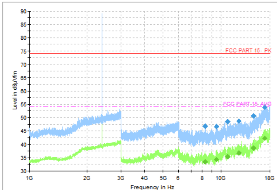
Fig.20 Radiated Spurious Emission (LE 1M, Ch0, 1 GHz ~18 GHz)
