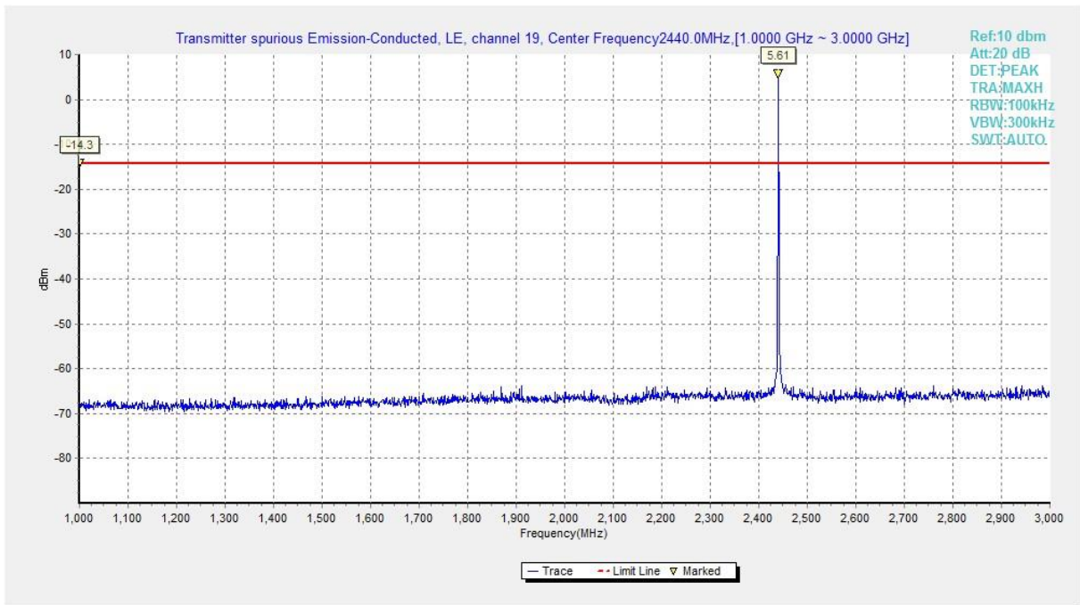
Fig.13 Conducted Spurious Emission (Ch19, 1 GHz-3 GHz)
