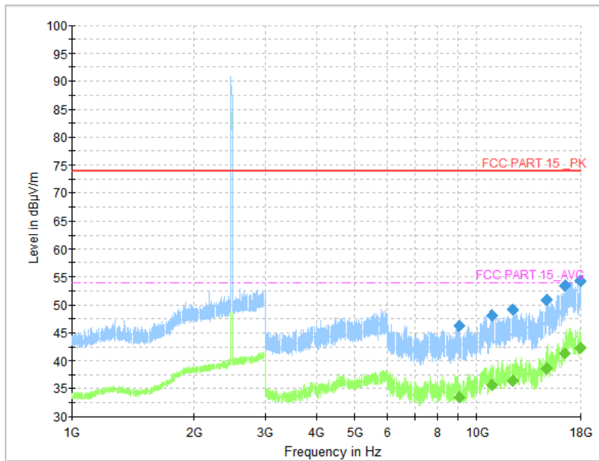
Fig.22 Radiated Spurious Emission (LE 1M, Ch39, 1 GHz ~18 GHz)
