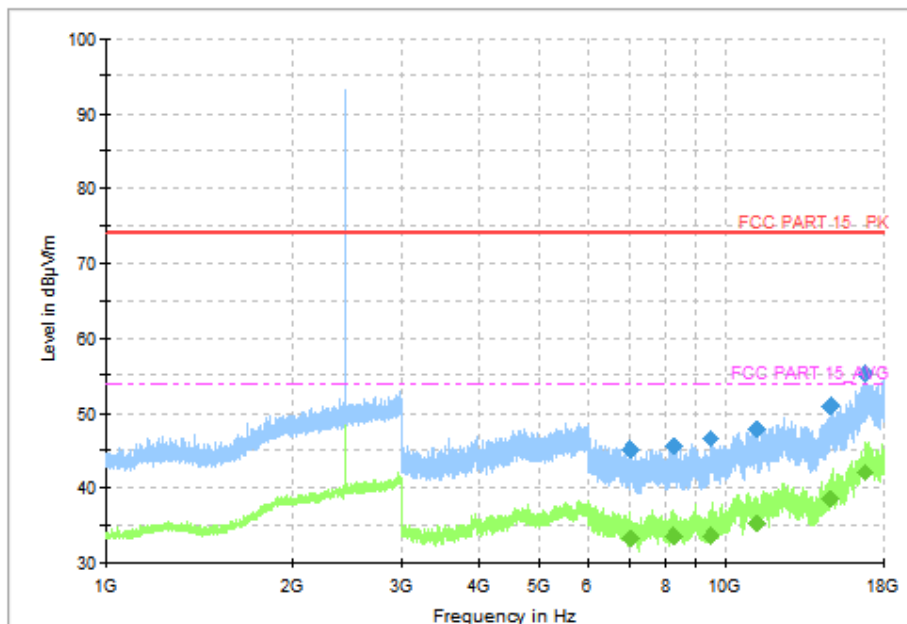
Fig.21 Radiated Spurious Emission (LE 1M, Ch19, 1 GHz ~18 GHz)
