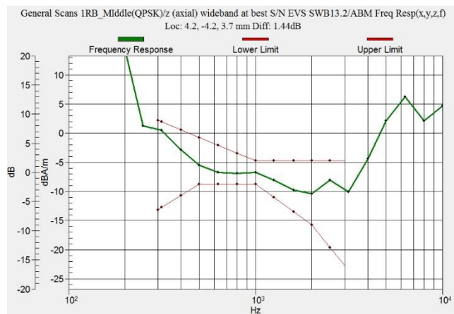
Figure C.9 Frequency Response of LTE B25
