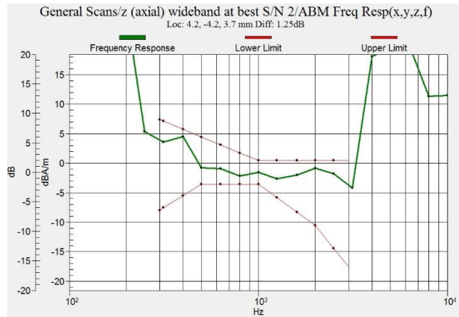
Figure C.20 Frequency Response of LTE B41 Power Class 2 - OTT VoIP
