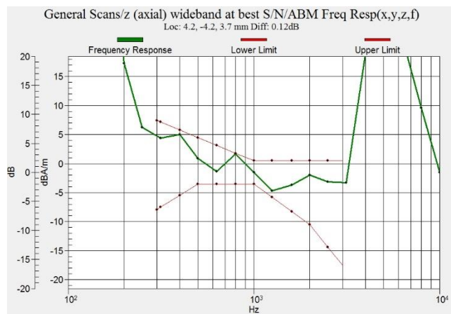
Figure C.18 Frequency Response of W850 - OTT VoIP
