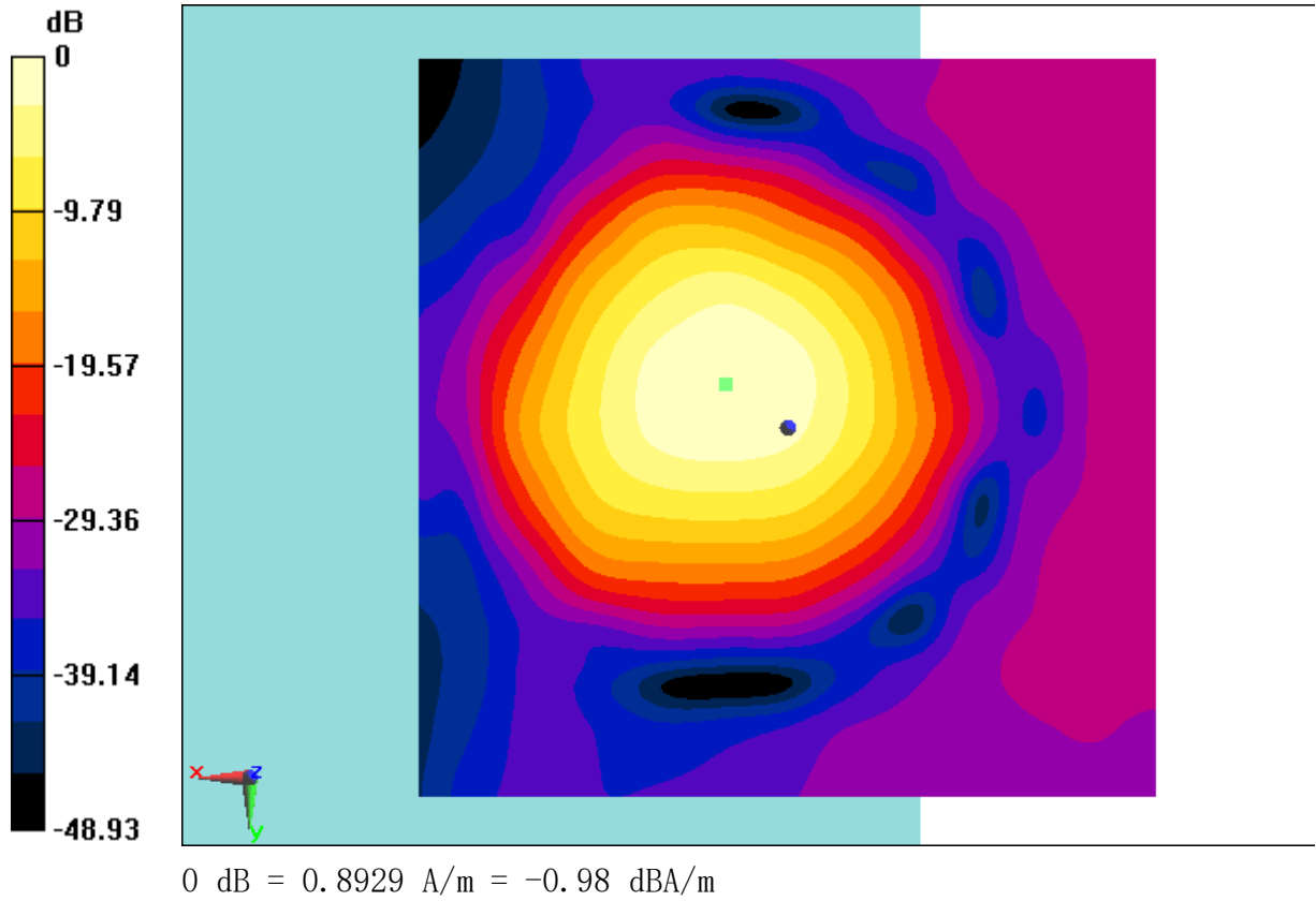
Fig B.16 T-Coil LTE B13
