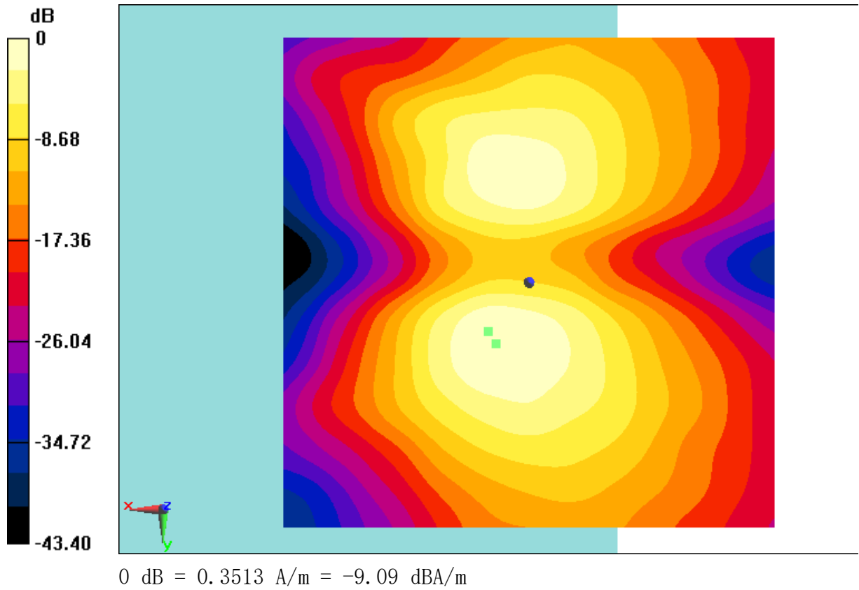
Fig B.11 T-Coil LTE B7
