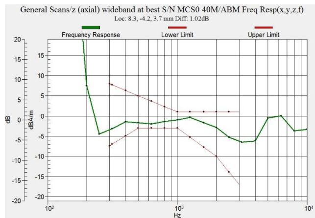
Figure C.21 Frequency Response of WiFi-2.4G - OTT VoIP
