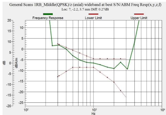
Figure C.11 Frequency Response of LTE B41 Power Class 2
