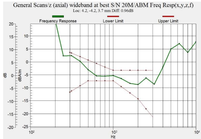
Figure C.8 Frequency Response of LTE B13
