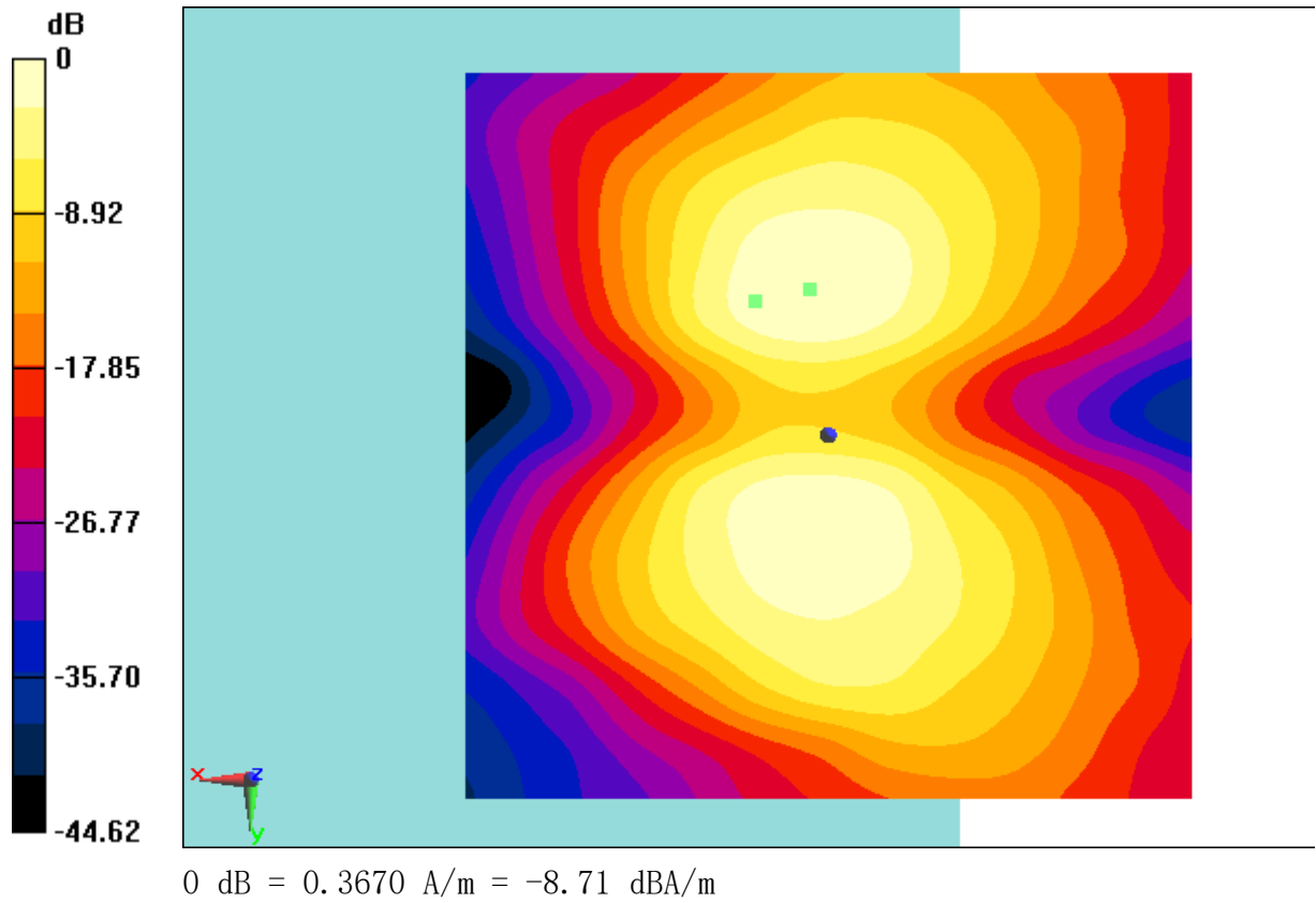
Fig B.17 T-Coil LTE B25
