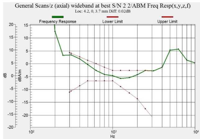
Figure C.17 Frequency Response of EDGE 850 - OTT VoIP
