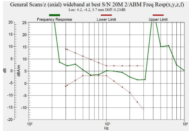
Figure C.19 Frequency Response of LTE B25 - OTT VoIP
