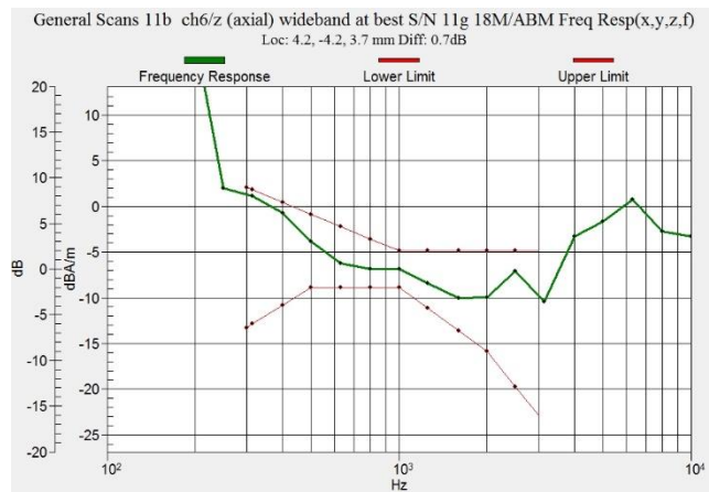
Figure C.15 Frequency Response of WiFi-2.4G
