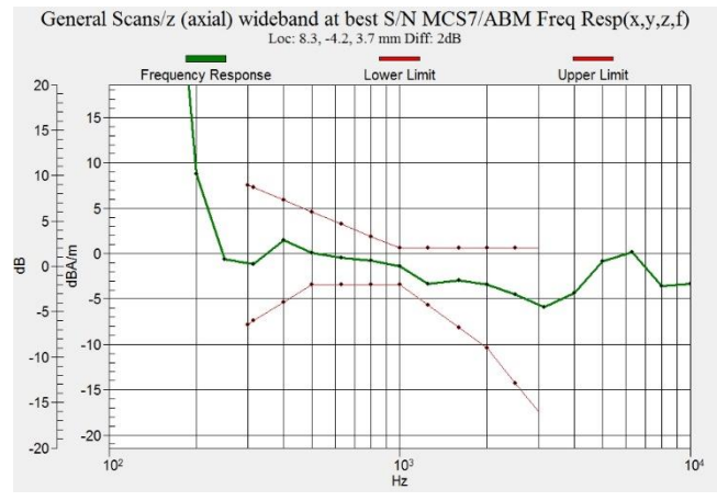
Figure C.22 Frequency Response of WiFi-5G - OTT VoIP
