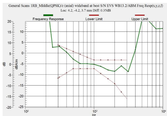
Figure C.12 Frequency Response of LTE B41 Power Class 3
