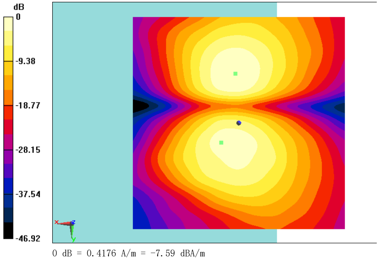
Fig B.27 T-Coil LTE B71
