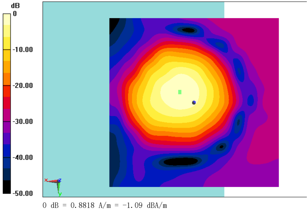
Fig B.14 T-Coil LTE B12
