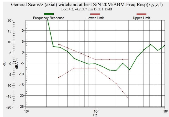
Figure C.10 Frequency Response of LTE B26
