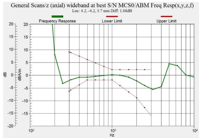
Figure C.16 Frequency Response of WiFi-5G
