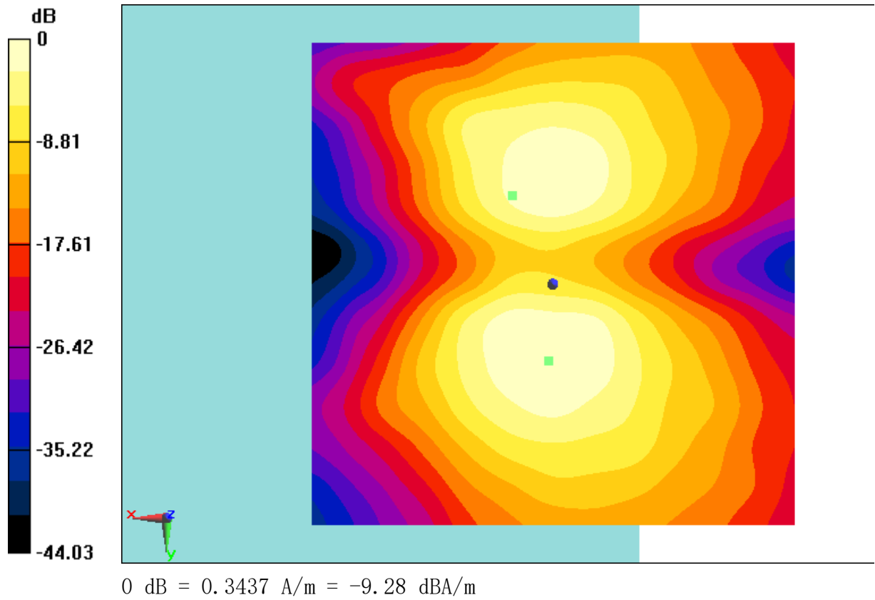
Fig B.15 T-Coil LTE B13
