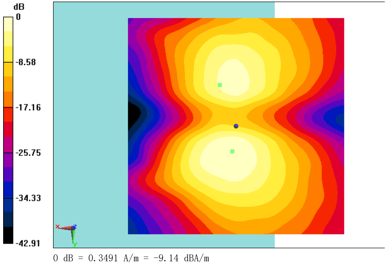
Fig B.19 T-Coil LTE B26
