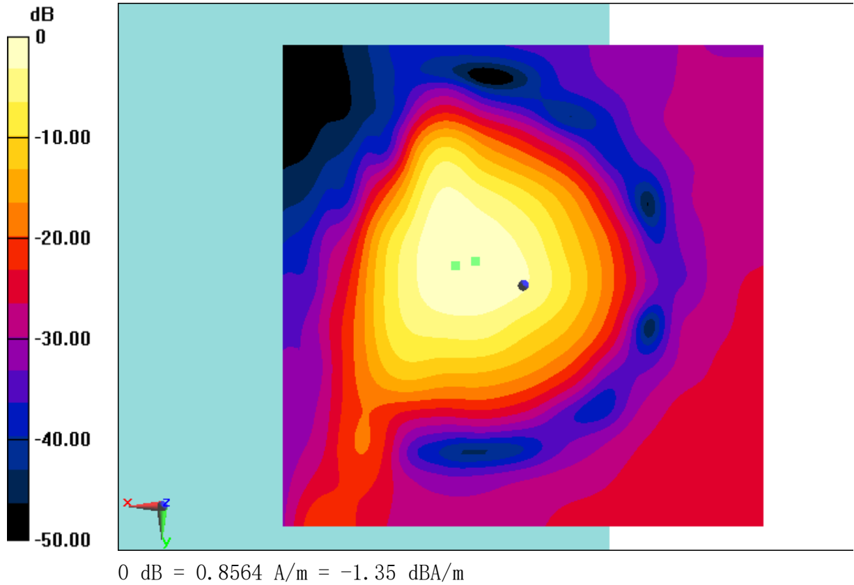
Fig B.22 T-Coil LTE B41
