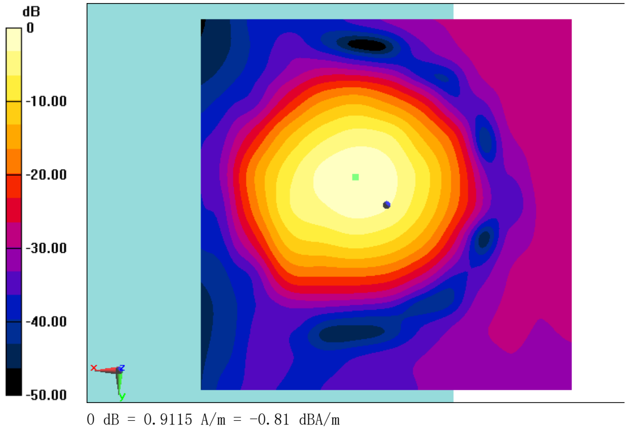
Fig B.12 T-Coil LTE B7
