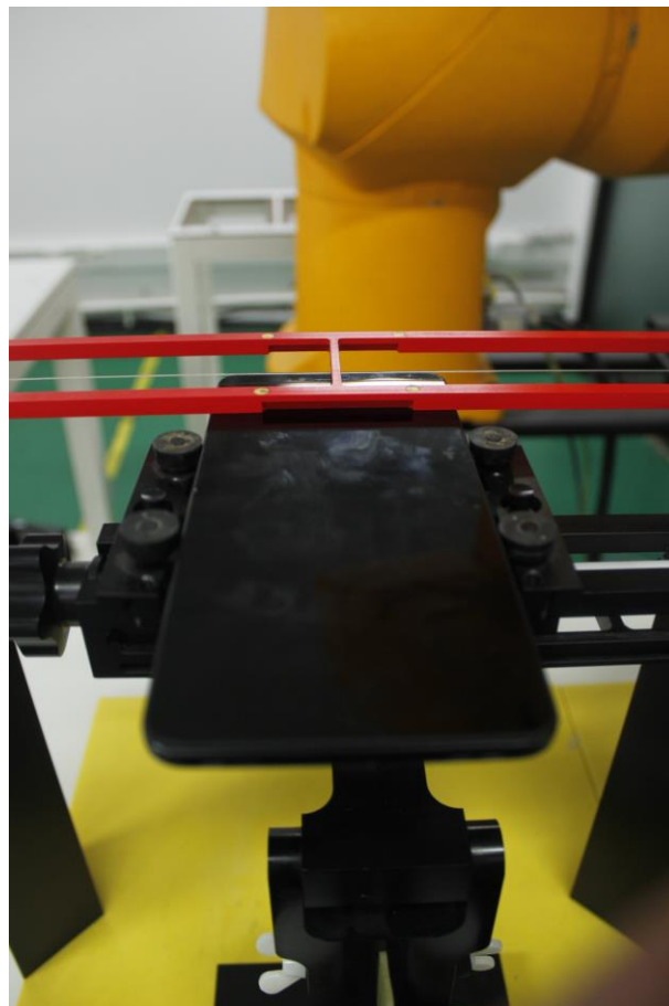
Picture 2: EUT Positioning for RF/T-coil
