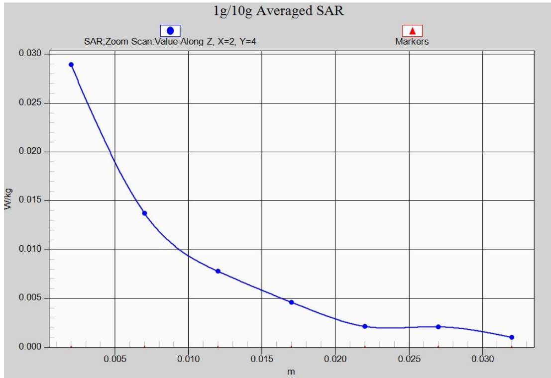
Fig. 27-1 Z-Scan at power reference point (LTE Band41)
