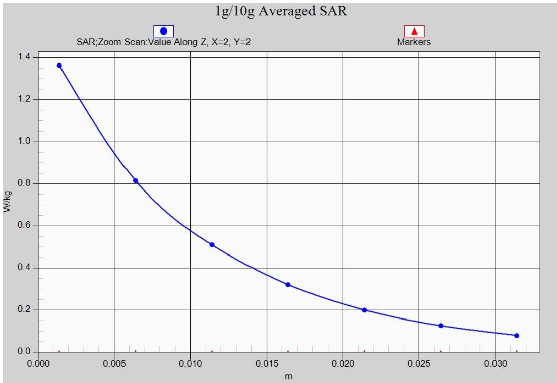
Fig. 21-1 Z-Scan at power reference point (LTE Band25)
