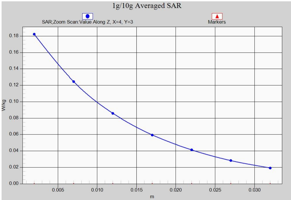
Fig. 29-1 Z-Scan at power reference point (LTE Band66)
