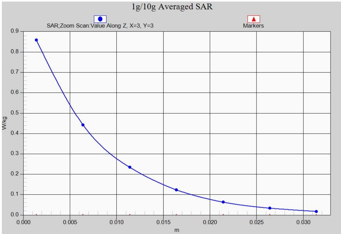
Fig. 35-1 Z-Scan at power reference point (2450 MHz)
