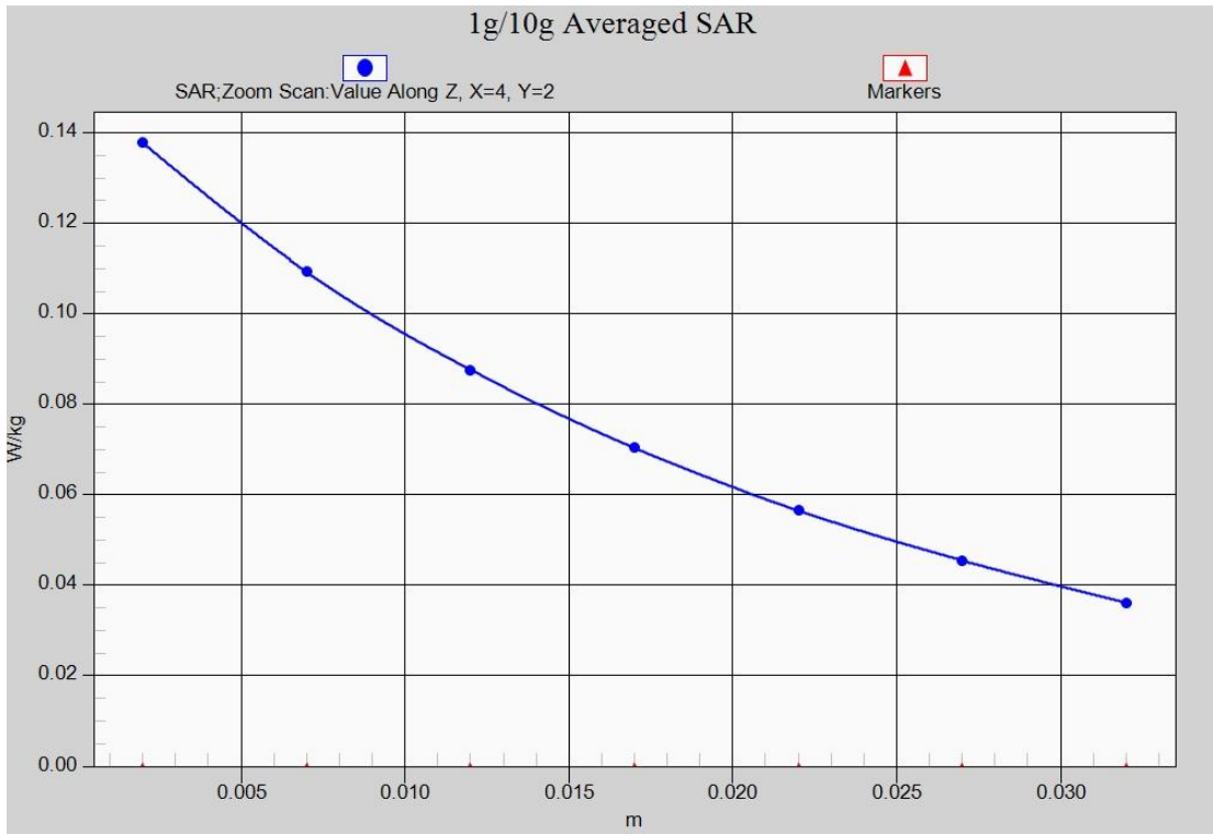
Fig. 23-1 Z-Scan at power reference point (LTE Band26)
