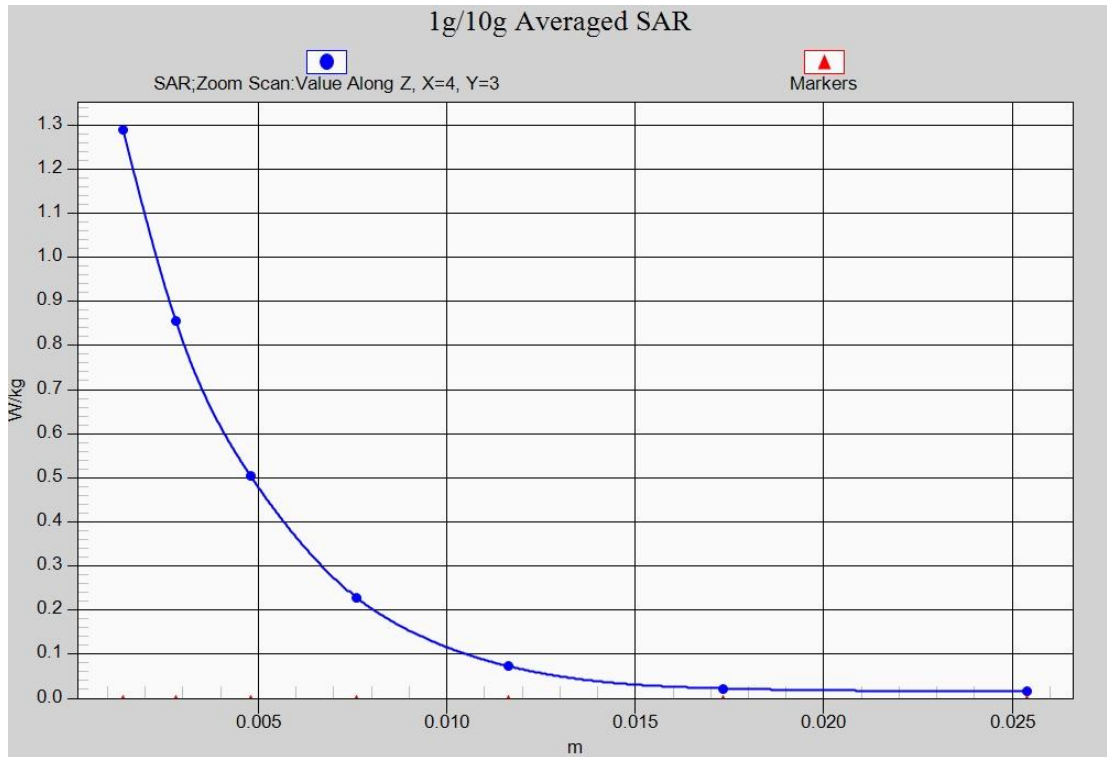
Fig. 36-1 Z-Scan at power reference point (5GHz)
