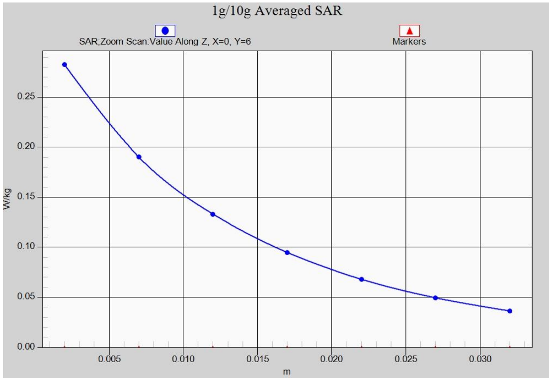
Fig. 33-1 Z-Scan at power reference point (LTE Band71)
