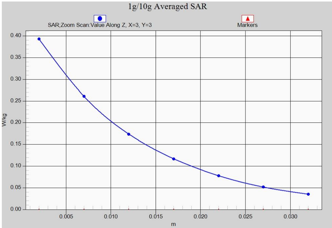
Fig. 20-1 Z-Scan at power reference point (LTE Band25)
