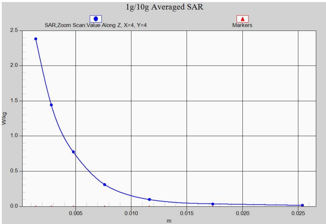
Fig. 37-1 Z-Scan at power reference point (5GHz)
