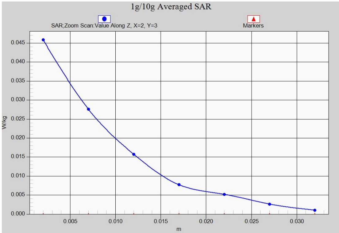
Fig. 25-1 Z-Scan at power reference point (LTE Band41)
