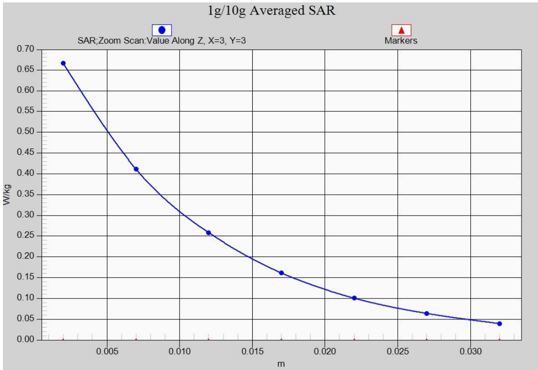
Fig. 22-1 Z-Scan at power reference point (LTE Band25)
