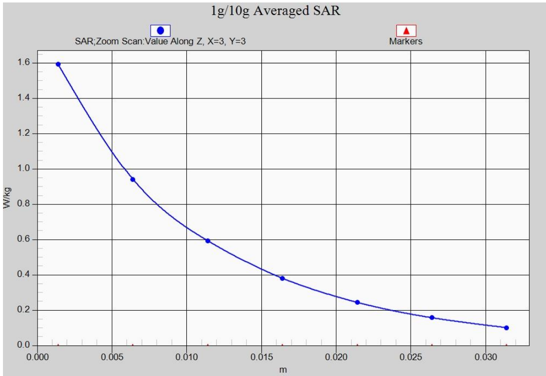
Fig. 30-1 Z-Scan at power reference point (LTE Band66)
