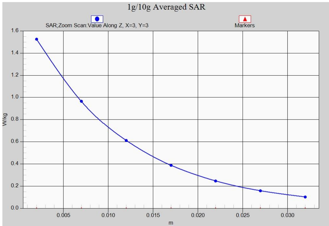
Fig. 31-1 Z-Scan at power reference point (LTE Band66)
