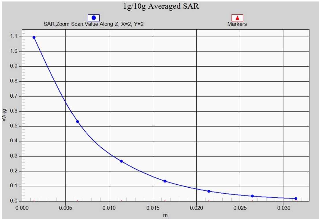
Fig. 28-1 Z-Scan at power reference point (LTE Band41)
