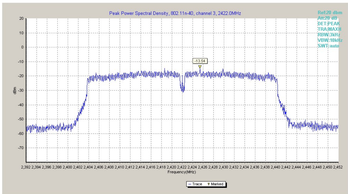
Fig.A.3.10 Power Spectral Density (802.11n-HT40, Ch 3)
