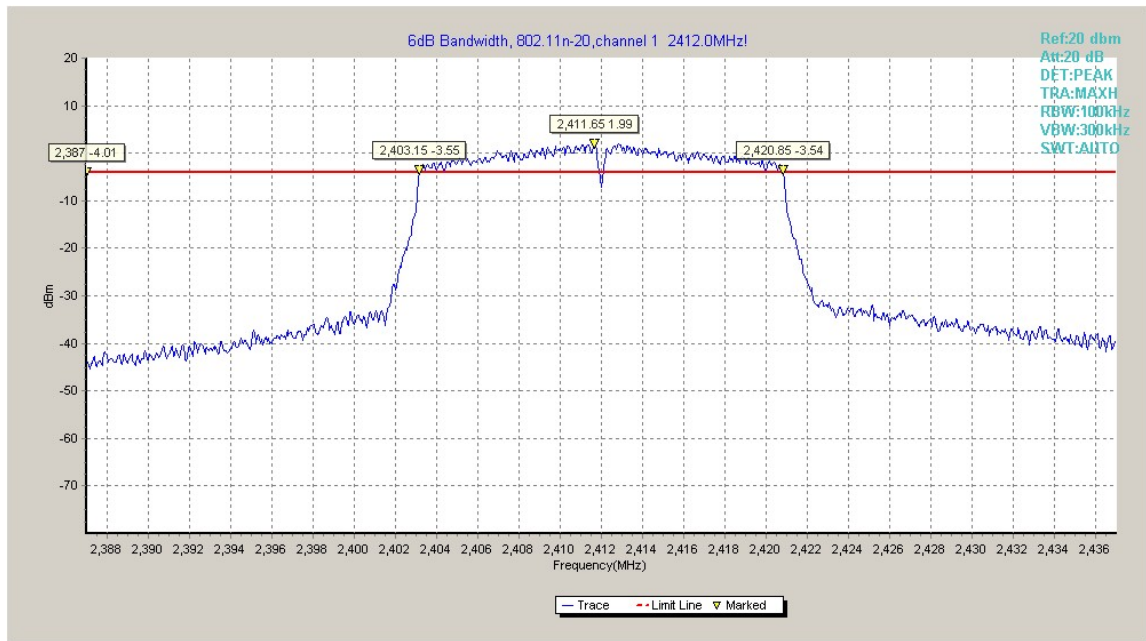
Fig.A.4.7 Occupied 6dB Bandwidth (802.11n-20MHz, Ch 1)
