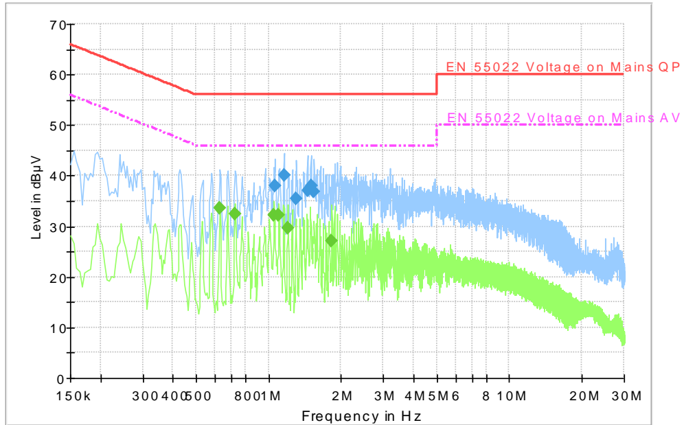
Fig.A.7.3 AC Power line Conducted Emission-802.11b
