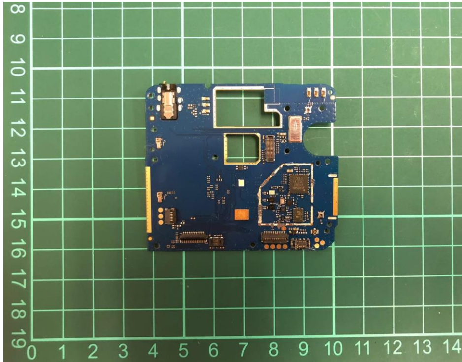
Mobile phone (5009A) Disassembly
