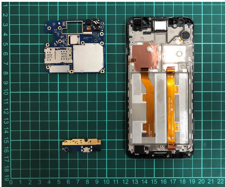
Mobile phone (5009U) Disassembly
