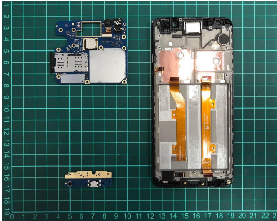
Mobile phone (5009A) Disassembly
