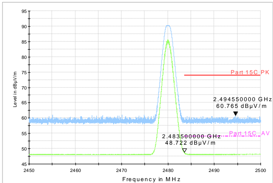
RE - Power-2.45GHz-2.5GHz
