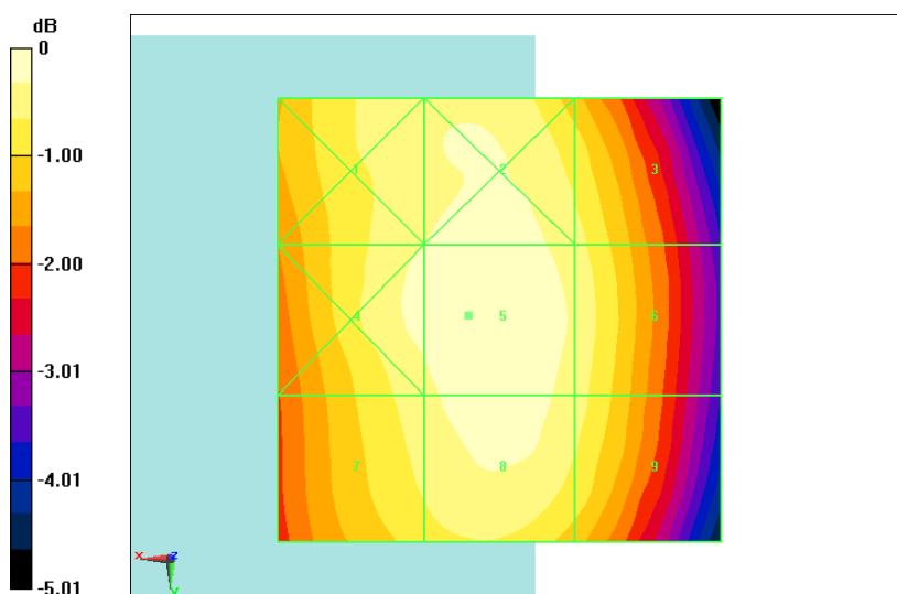
Fig B.1 HAC RF E-Field GSM 850 High
