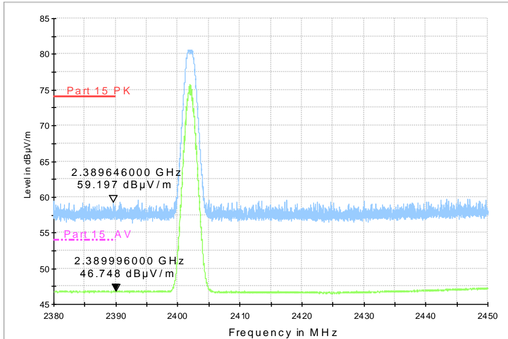
RE - Power-2.38GHz-2.45GHz
