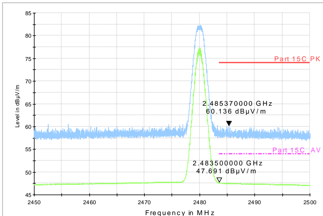
RE - Power-2.45GHz-2.5GHz
