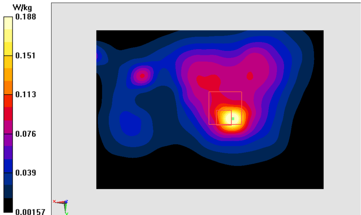
Fig.10 2450 MHz
