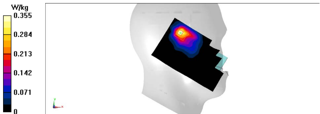
Fig.9 2450 MHz
