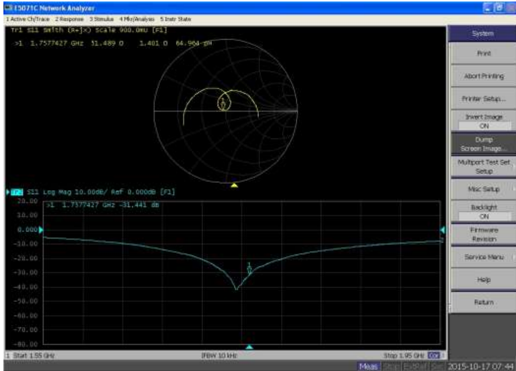
1750MHz Head
