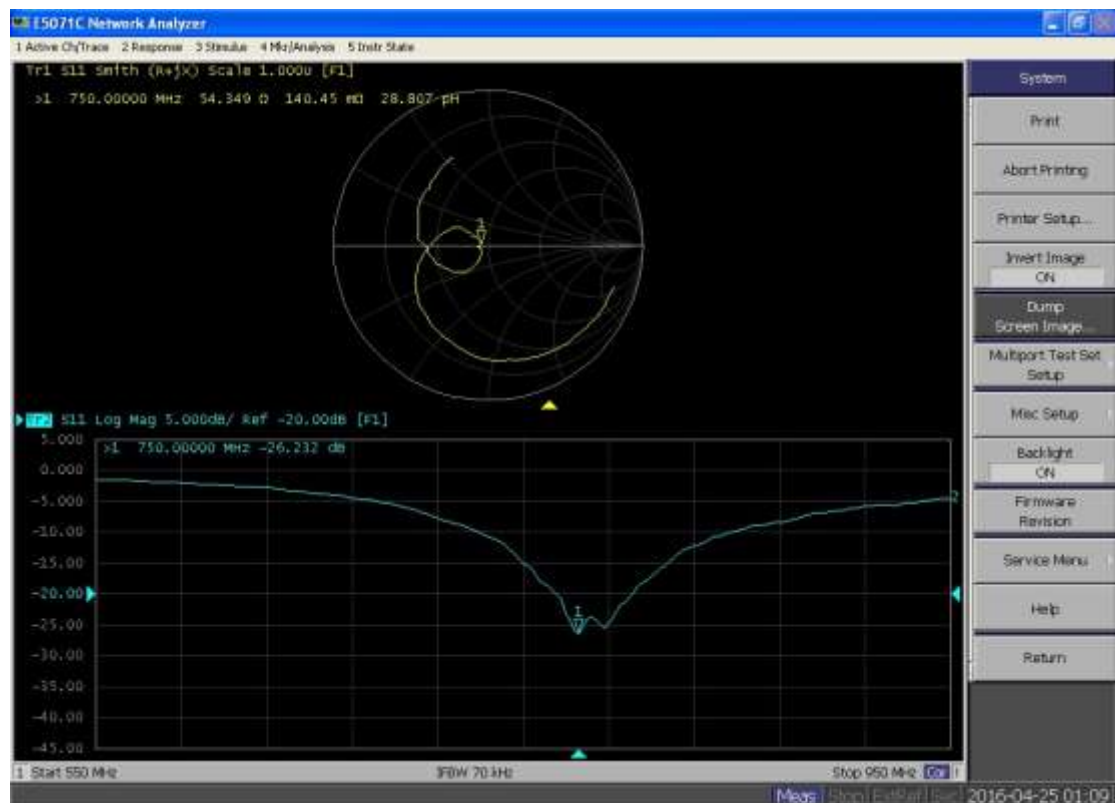
750MHz Head
