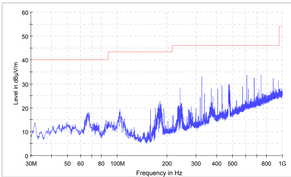
Normal Sweep_TT2m
