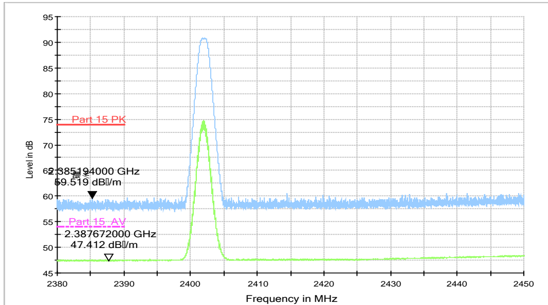
RE - Power-2.38GHz-2.45GHz
