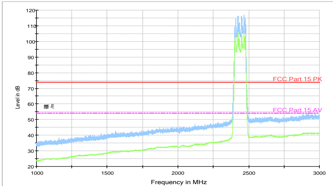
RE - TX - WLAN BT +AV+PK_1GHz-3GHz
