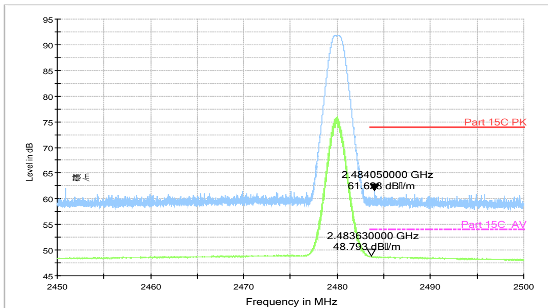
RE - Power-2.45GHz-2.5GHz
