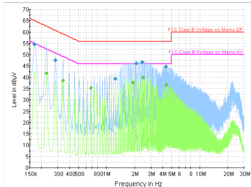
Fig.A.7.1 AC Powerline Conducted Emission-802.11b withCBA3068AGAC1
