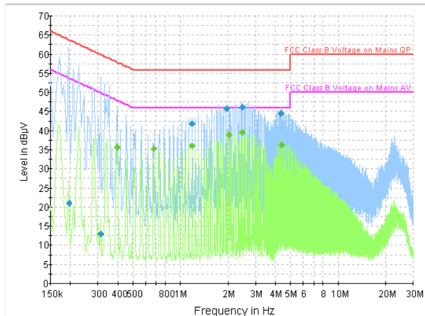
Fig.A.7.2 AC Powerline Conducted Emission-Idle withCBA3068AGAC1
