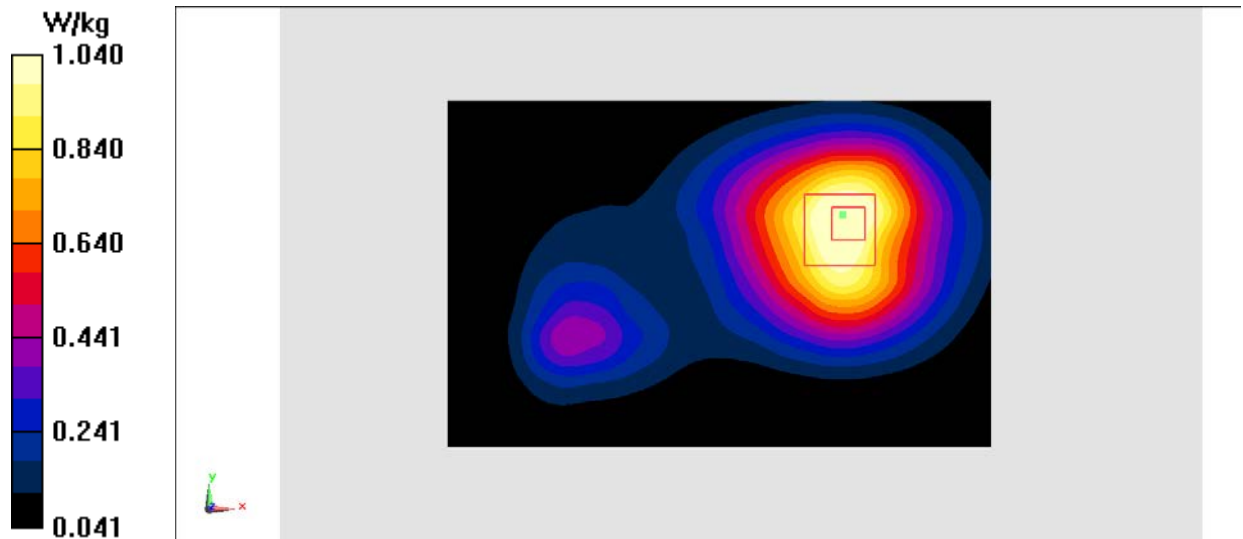
Fig.8 1700 MHz
