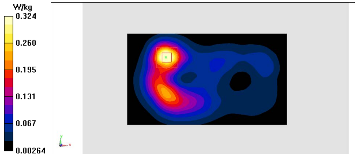
Fig.20 2450 MHz
