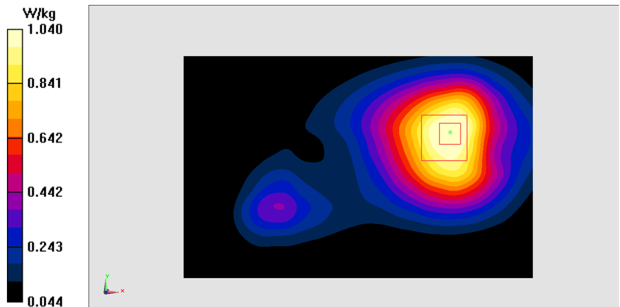
Fig.8 1700 MHz
