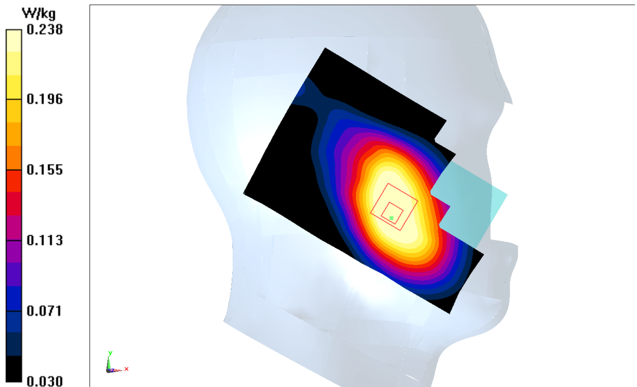
Fig.19 LTE Band12
