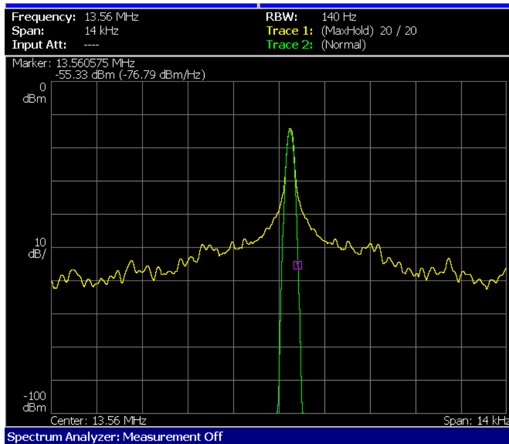
Figure A-4: Test result of EUT2 at test set. NFC02
