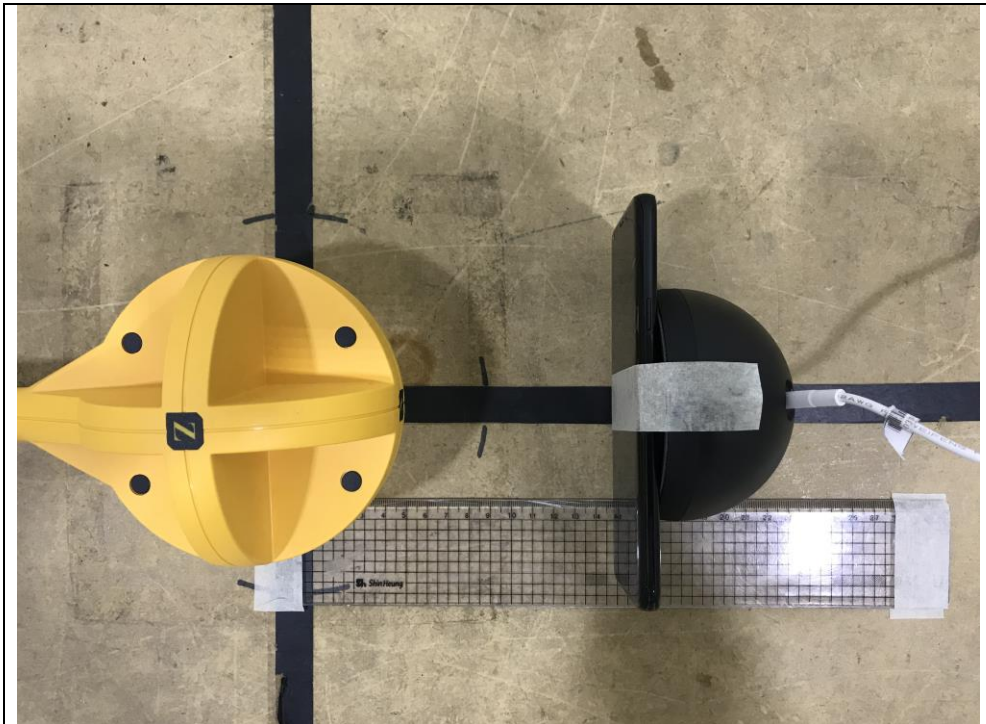
- 5 W Charging mode_Position E (H-Field)
