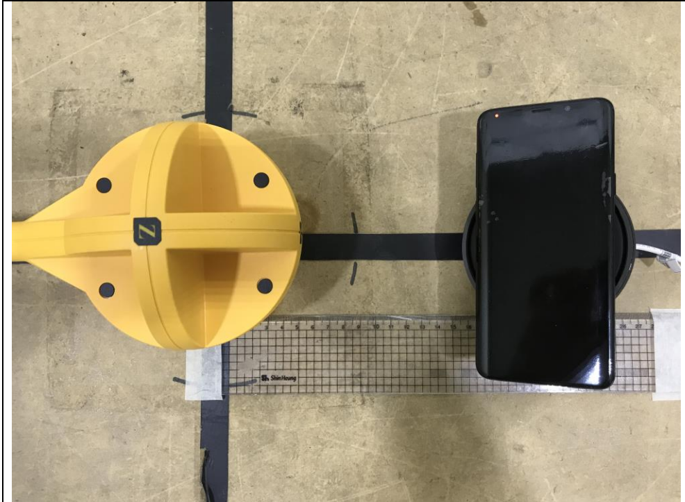
- 5 W Charging mode_Position D (H-Field)
