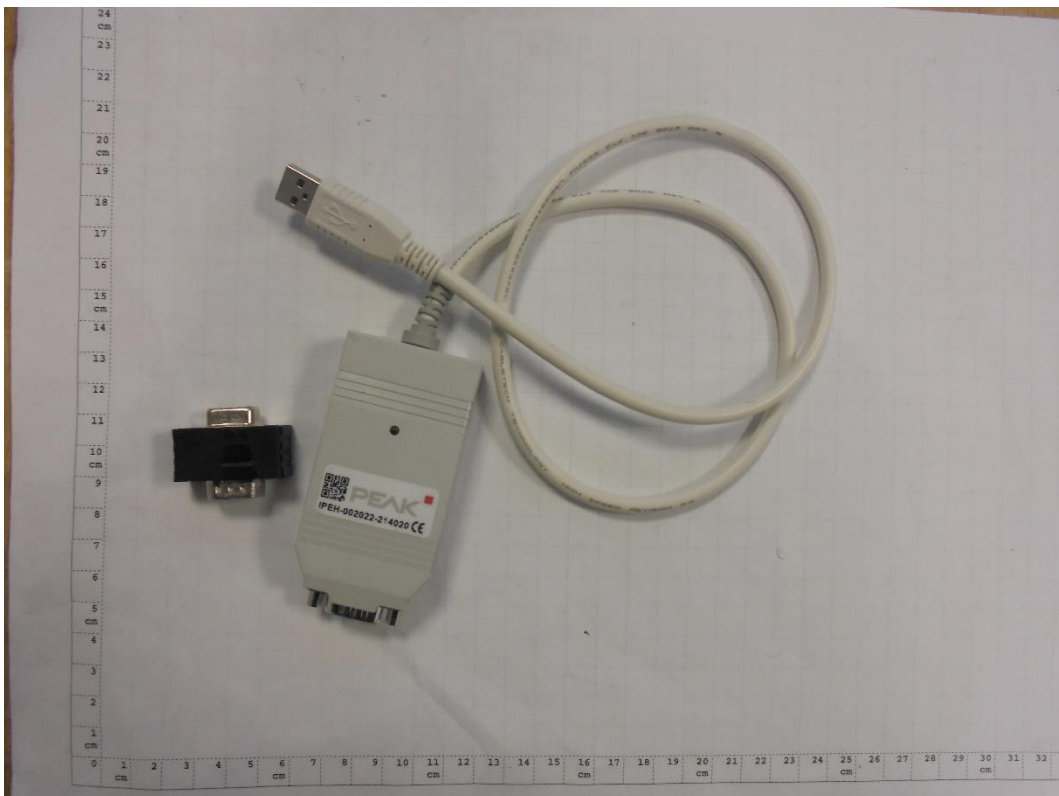
Photograph 9: CAN to USB Adapter with 120 Ohm Termination
