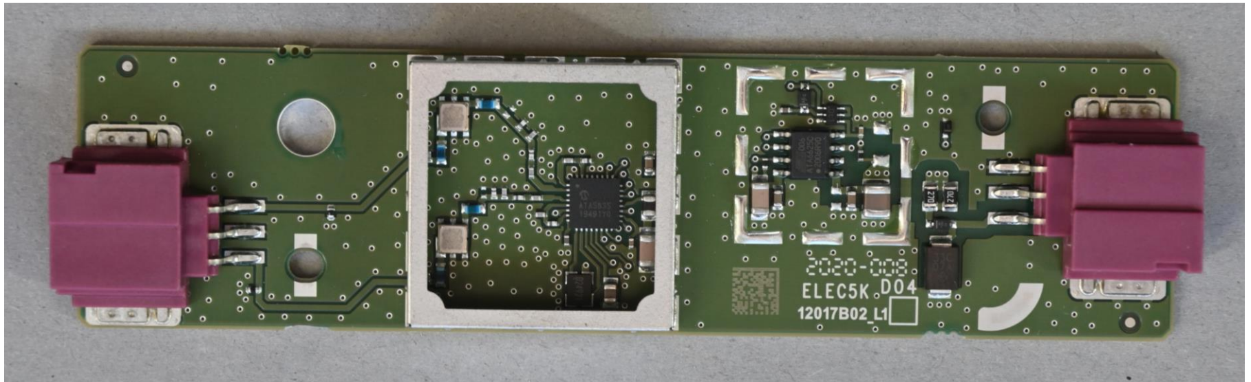
PCB top – RF shielding open
