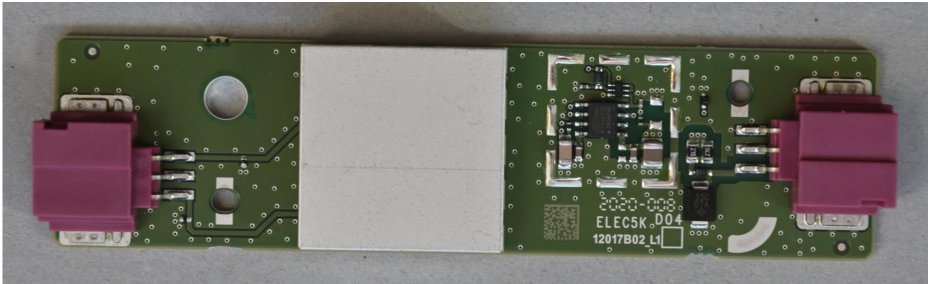
PCB top – RF shielding closed
