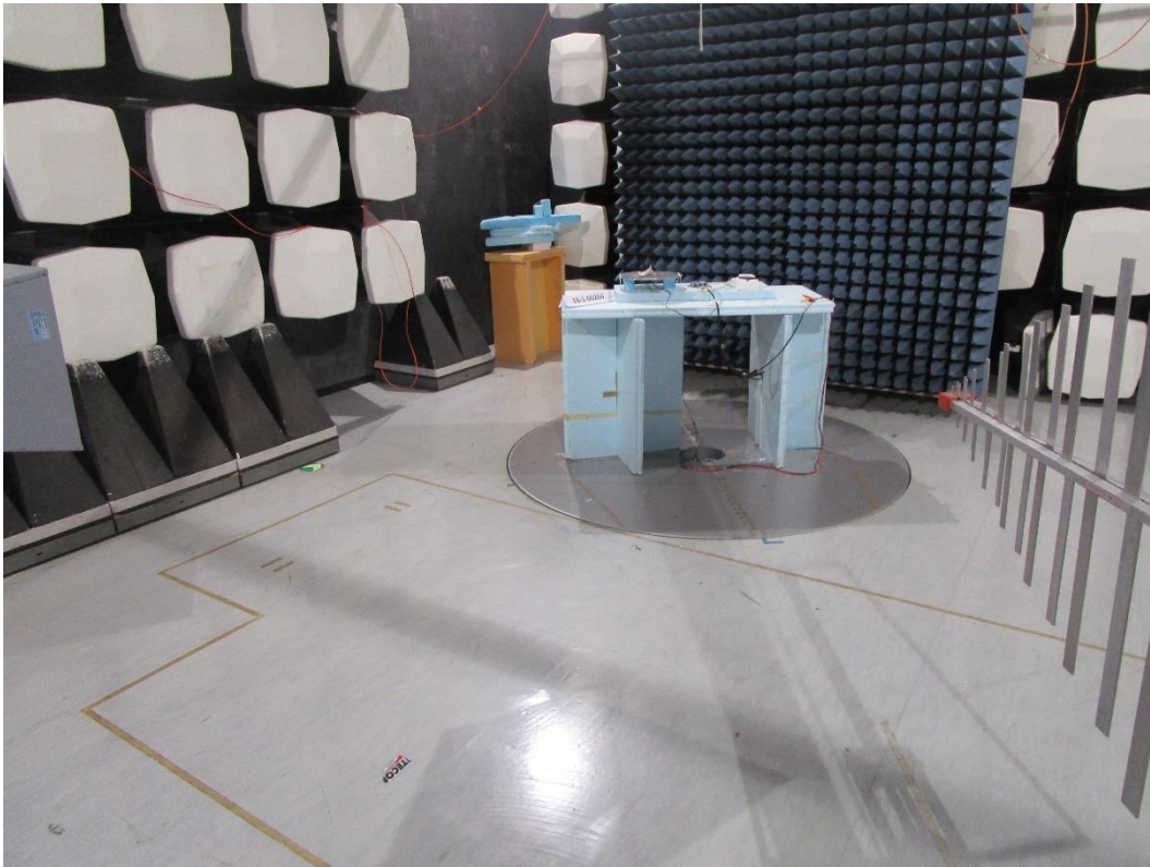
Photograph 1: Radiated measurements test set-up overview
