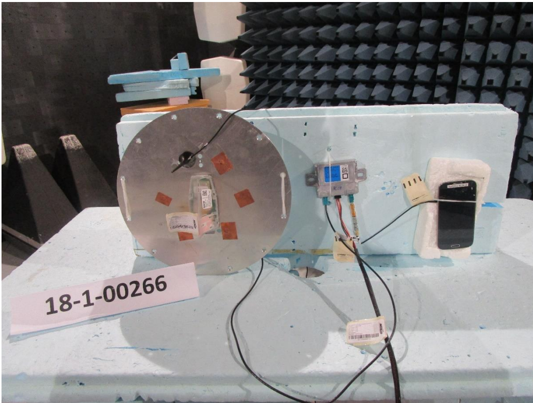
Photograph 3: Radiated measurements test set-up standing close view
