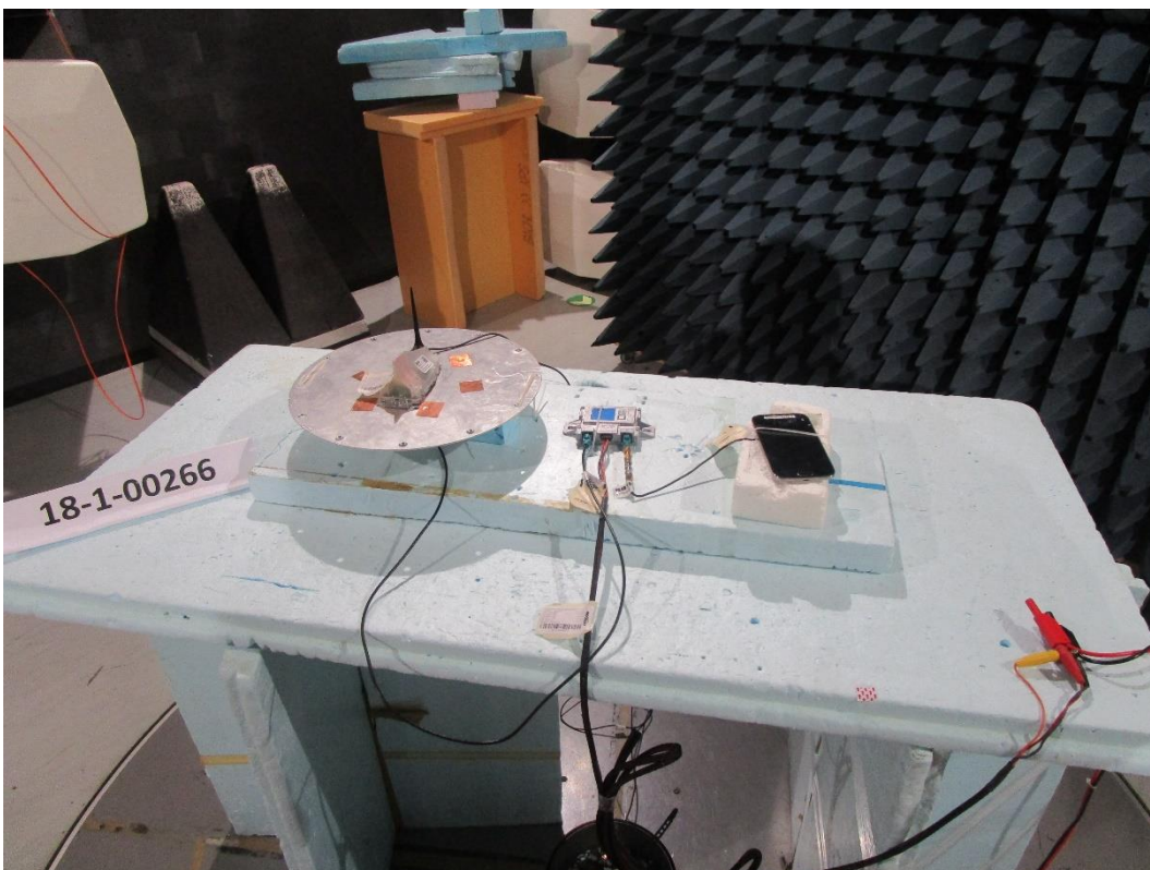
Photograph 2: Radiated measurements test set-up laying close view
