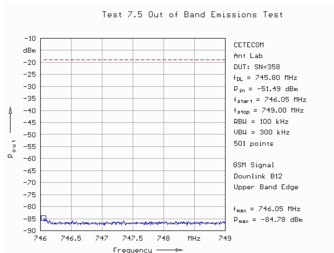
Fig. 77: Out-of-band emissions in downlink in band 12 applying a GSM signal for the upper band edge.
