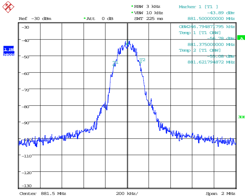
Fig. 229: Occupied bandwidth for GSM signal when using a through in band 5 downlink.
