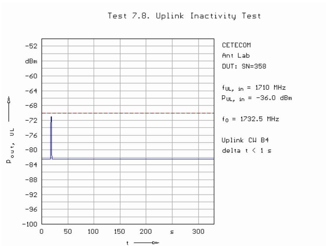
Fig. 196: Uplink inactivity test in band 4.
