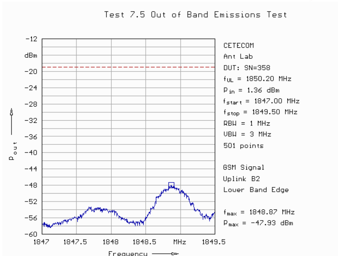
Fig. 60: Out-of-band emissions in uplink in band 2 applying a GSM signal for the lower band edge.
