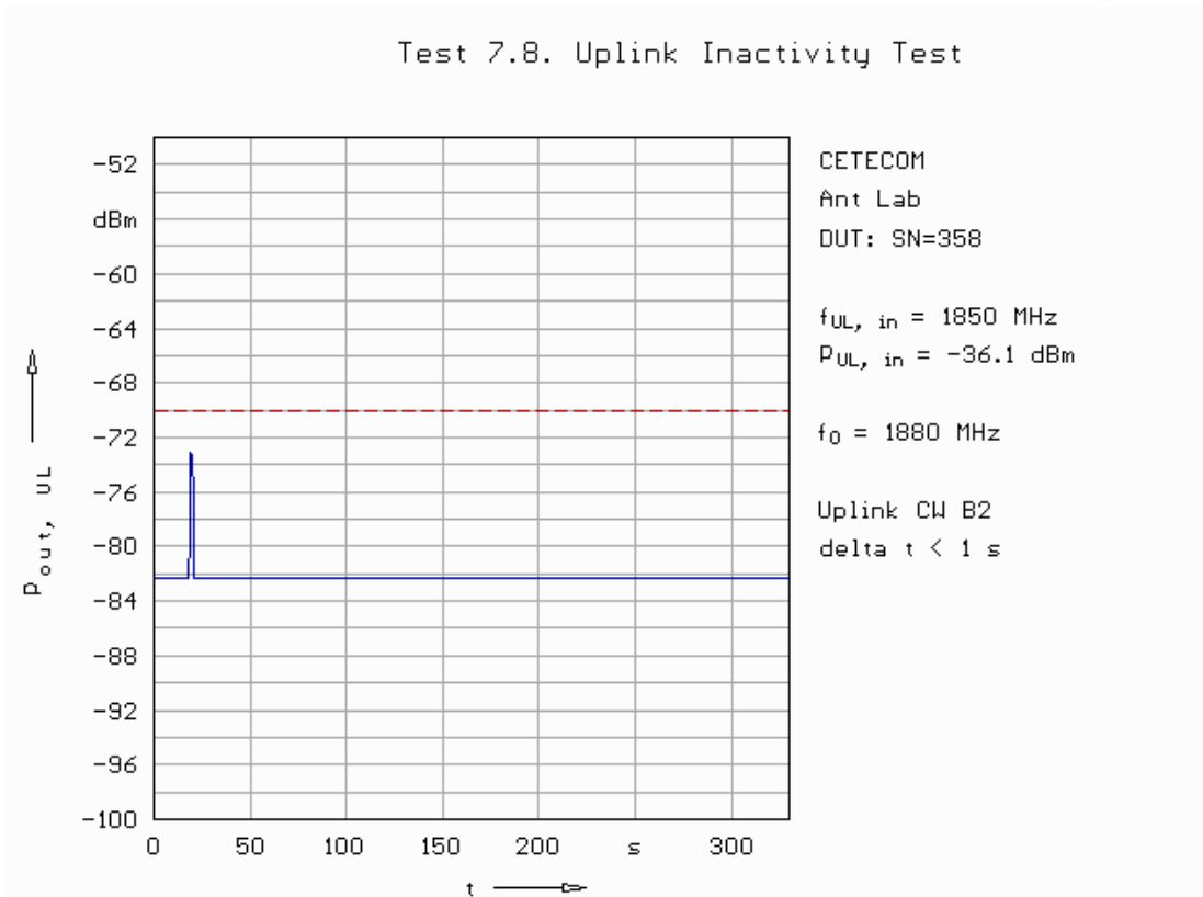
Fig. 195: Uplink inactivity test in band 2.
