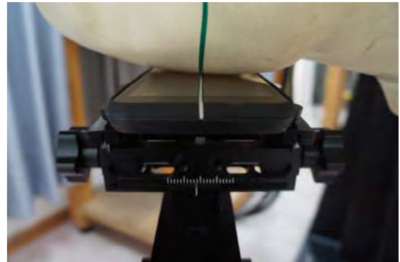
Fig.3 Right Head Section / Cheek-Touch Position
