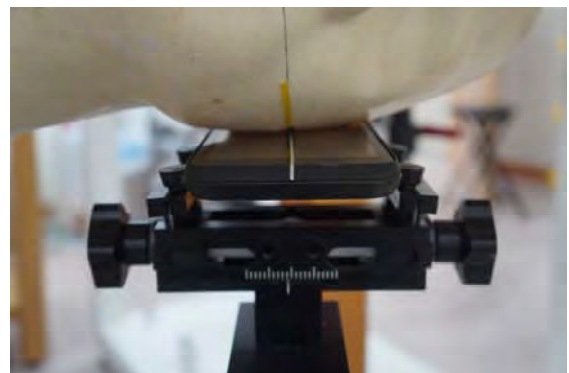
Fig.4 Right Head Section / Ear-Tilt Position(15°)
