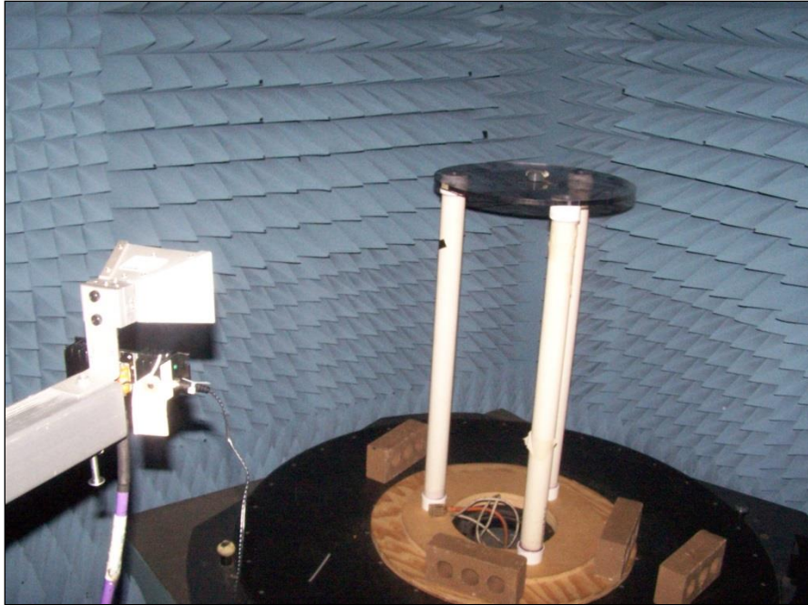
Photograph 4. Radiated Spurious Emissions, Test Setup, 18 GHz – 25 GHz
