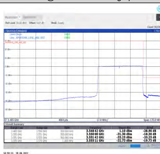
1-N77-3450-3550--30-50-H-6-CP-QPSK-Outer_Fu ll-133@0-Ant1-PASS-see graph
