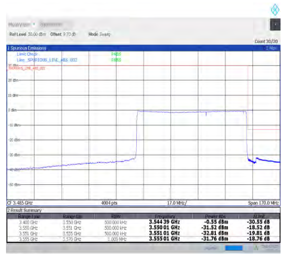
1-N77-3450-3550--30-70-L-6-CP-QPSK-Outer_Ful I-189@0-Ant1-PASS-see graph
