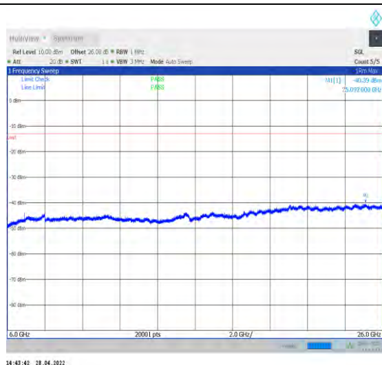
1-N77-3450-3550--30-100-M-1-DFT-QPSK-Edge_1R B_Left-1@0-6000-26000-Ant1--40.39--13-PASS
