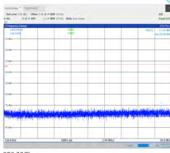
1-N77-3450-3550--30-100-H-1-DFT-QPSK-Edge_1R B_Left-1@0-0.15-30-Ant2--71.12--33-PASS
