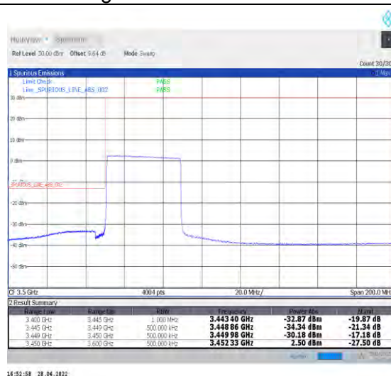
1-N77-3450-3550--30-40-L-6-CP-QPSK-Outer_Ful I-106@0-Ant1-PASS-see graph
