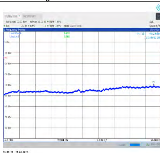
1-N77-3450-3550--30-100-L-1-DFT-QPSK-Edge_1R B_Left-1@0-6000-26000-Ant1--40.24--13-PASS
