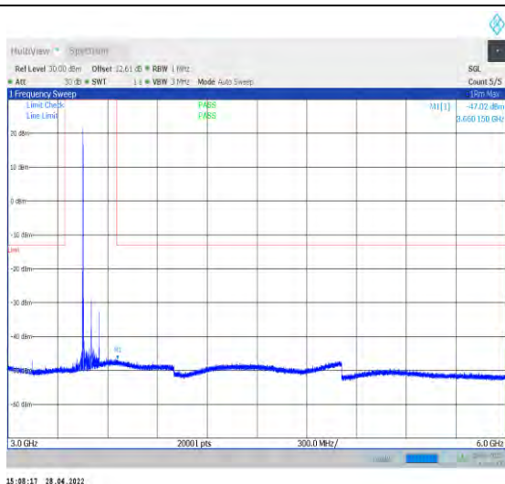
1-N77-3450-3550--30-100-L-1-DFT-QPSK-Edge_1R B_Left-1@0-3000-6000-Ant1--47.02--13-PASS
