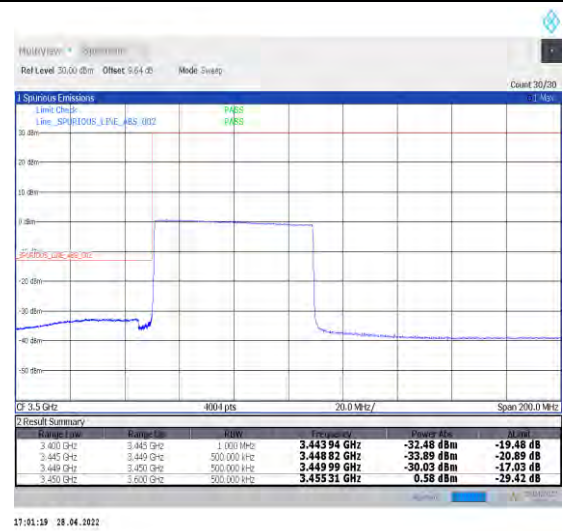
1-N77-3450-3550--30-60-L-6-CP-QPSK-Outer_Ful I-162@0-Ant1-PASS-see graph
