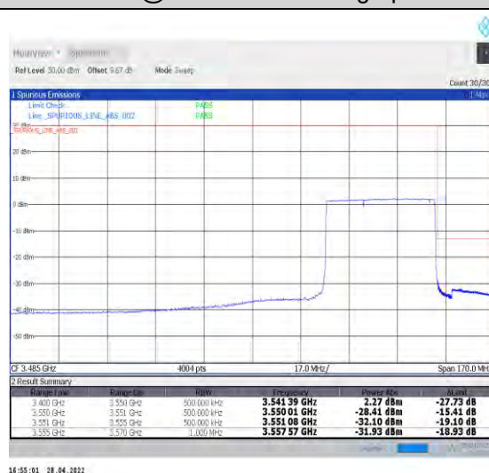
1-N77-3450-3550--30-40-H-6-CP-QPSK-Outer_Fu ll-106@0-Ant1-PASS-see graph
