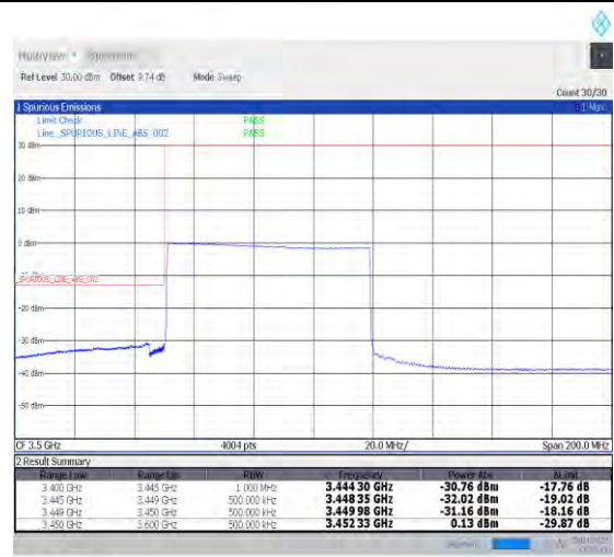
1-N77-3450-3550--30-70-L-6-CP-QPSK-Outer_Ful I-189@0-Ant1-PASS-see graph
