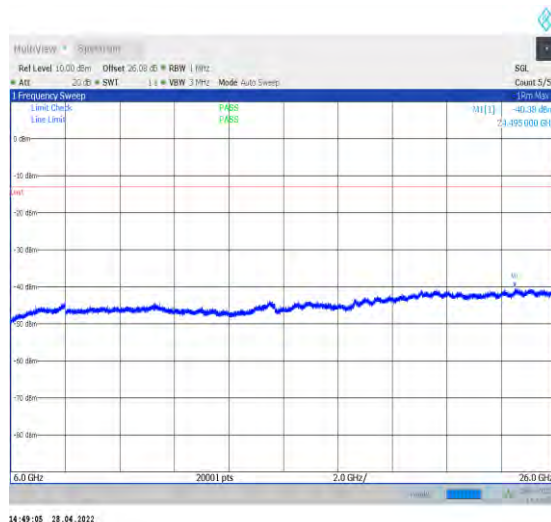
1-N77-3450-3550--30-100-H-1-DFT-QPSK-Edge_1R B_Left-1@0-6000-26000-Ant2--40.38--13-PASS
