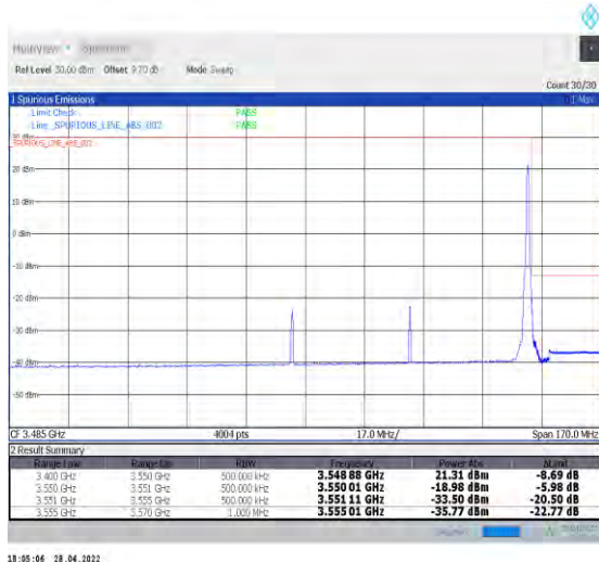
1-N77-3450-3550--30-70-H-5-CP-QPSK-Edge_1RB_Ri ght-1@188-Ant2-PASS-see graph
