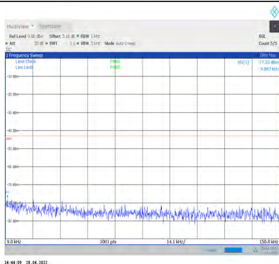
1-N77-3450-3550--30-100-H-1-DFT-QPSK-Edge_1R B_Left-1@0-0.009-0.15-Ant1--77.33--43-PASS
