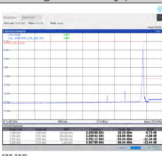
1-N77-3450-3550--30-40-H-5-CP-QPSK-Edge_1RB_Ri ght-1@105-Ant1-PASS-see graph
