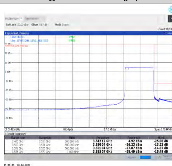
1-N77-3450-3550--30-30-H-6-CP-QPSK-Outer_Fu ll-78@0-Ant2-PASS-see graph
