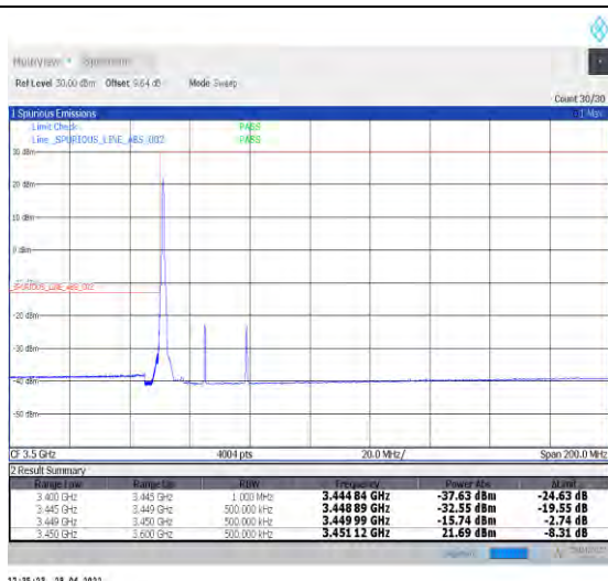
1-N77-3450-3550--30-30-L-4-CP-QPSK-Edge_1RB_Le ft-1@0-Ant2-PASS-see graph
