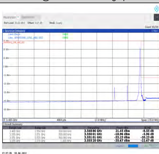
1-N77-3450-3550--30-30-H-5-CP-QPSK-Edge_1RB_Ri ght-1@77-Ant2-PASS-see graph
