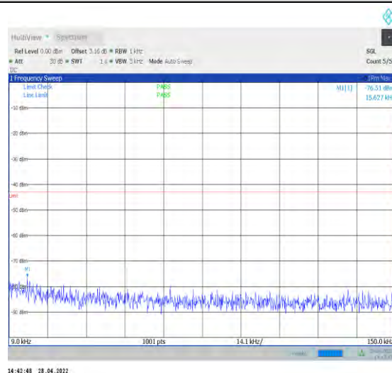
1-N77-3450-3550--30-100-M-1-DFT-QPSK-Edge_1R B_Left-1@0-0.009-0.15-Ant1--76.51--43-PASS
