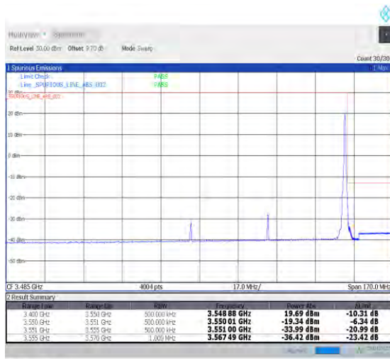
1-N77-3450-3550--30-70-L-4-CP-QPSK-Edge_1RB_Le ft-1@0-Ant1-PASS-see graph
