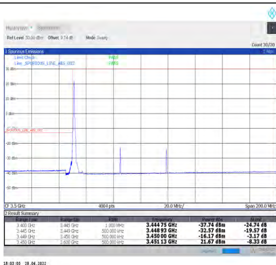
1-N77-3450-3550--30-70-L-4-CP-QPSK-Edge_1RB_Le ft-1@0-Ant2-PASS-see graph
