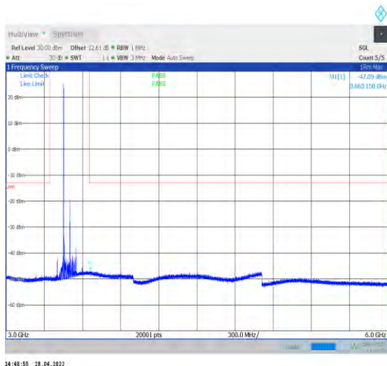
1-N77-3450-3550--30-100-H-1-DFT-QPSK-Edge_1R B_Left-1@0-3000-6000-Ant2--47.09--13-PASS
