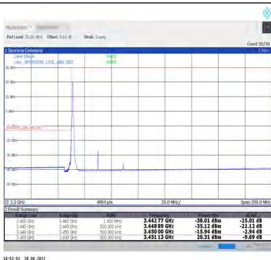
1-N77-3450-3550--30-40-L-4-CP-QPSK-Edge_1RB_Le ft-1@0-Ant1-PASS-see graph
