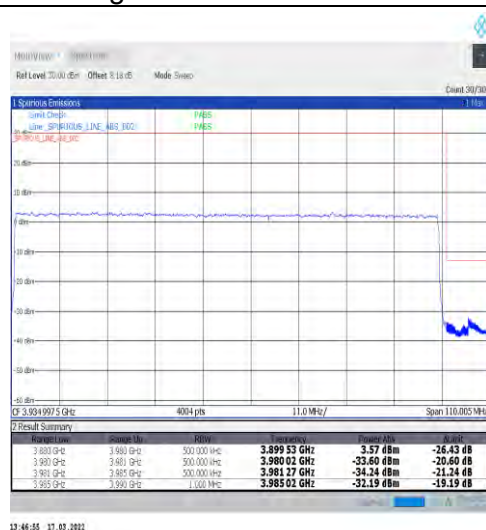
1-N77-3700-3980-30-100-H-3-DFT-PI2BPSK-Outer_Full-270@0-Ant1-PASS-see graph
