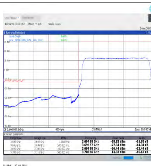
1-N77-3700-3980-30-10-L-3-DFT-PI2BPSK-Outer _Full-24@0-Ant1-PASS-see graph
